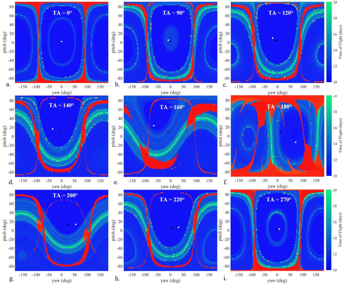
Figure 23. Recontact Maps for deployment with \Delta v = 1 m/s.
