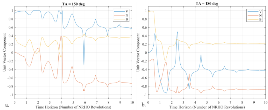
Figure 3. VNB components of the most-stretching directions as a function of time horizon for TA = 150° (a) and TA = 180° (b) in the CR3BP.
