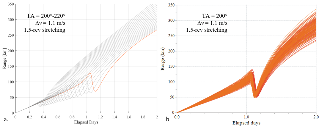
Figure 22. Decrease in the Gateway-cubesat range for deployments after apolune in the CR3BP (a) and the ephemeris model (b).
