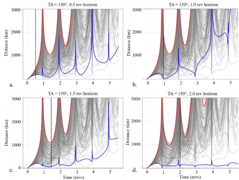
Figure 4. Gateway-cubesat range as a function of time past deployment for all directions at TA = 150° or EA = 84° in the CR3BP. Most-stretching (red) and most-restoring (blue) directions plotted for four time horizons.
