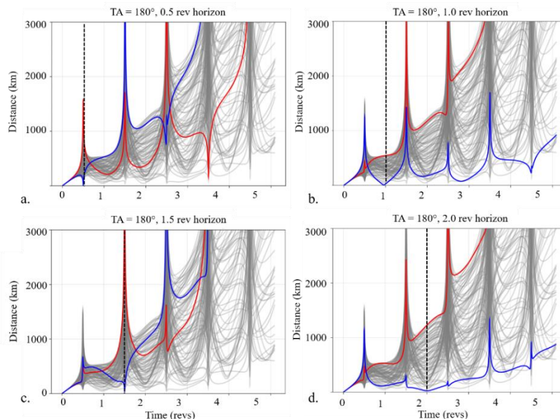
Figure 5. Gateway-cubesat range as a function of time past deployment for all directions at TA = EA = 180^\circ in the CR3BP. Most-stretching (red) and most-restoring (blue) directions plotted for four time horizons.
