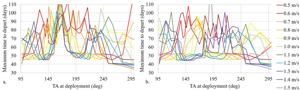
Figure 16. Maximum time to depart for deployment locations around the NRHO in the 1.5-revolution stretching direction (a) and the 6.5-revolution stretching direction (b).
