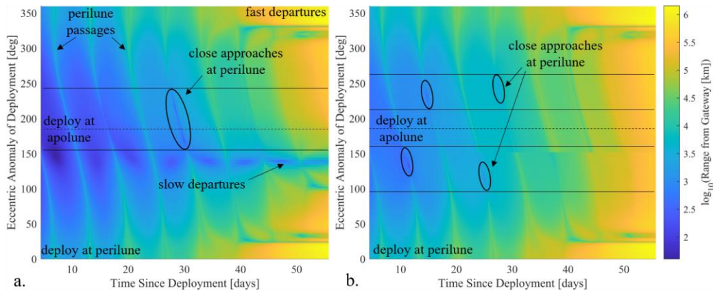
Figure 10. Gateway-cubesat range as a function of deployment EA and time past deployment in the CR3BP. Deployment in the most-stretching directions after 1.5 revolution time horizon (a) and 6.5 revolution time horizon (b) with a 1 m/s \Delta v .
