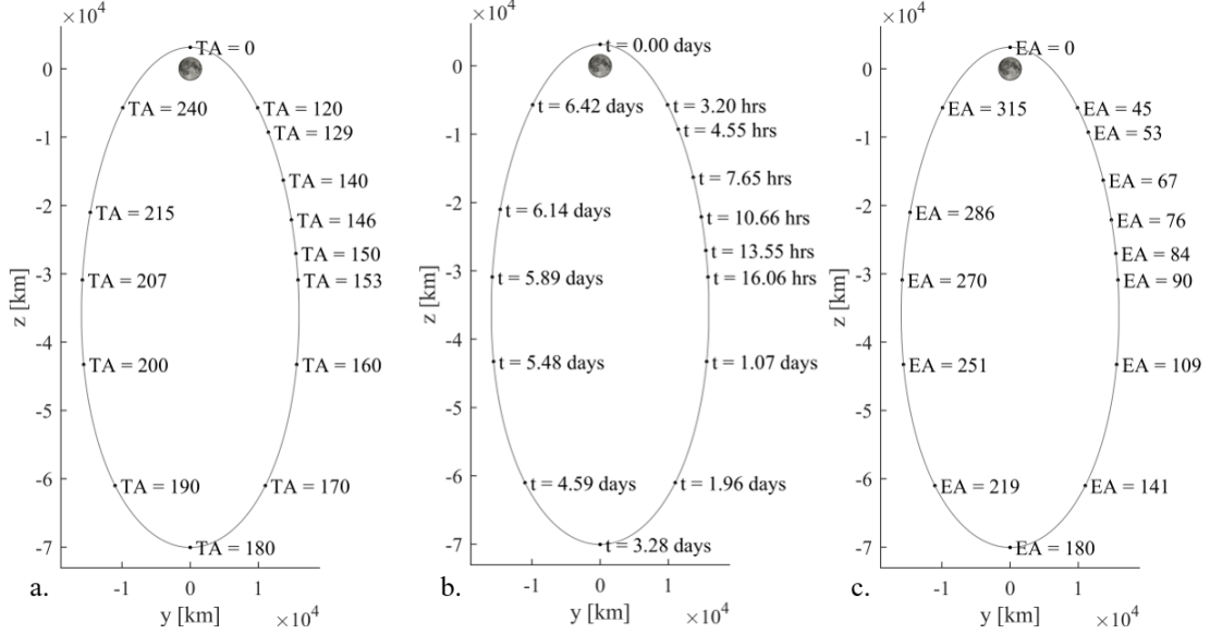
Figure 1. NRHO in the CR3BP parameterized by osculating true anomaly (a), time past perilune (b), and osculating eccentric anomaly (c).
