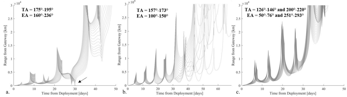
Figure 13. Gateway-cubesat range vs. time for three deployment regions with a 1 m/s \Delta v in a 1.5-revolution stretching direction. Close approach keep-out (a), slow departures (b), and desirable departures (c).
