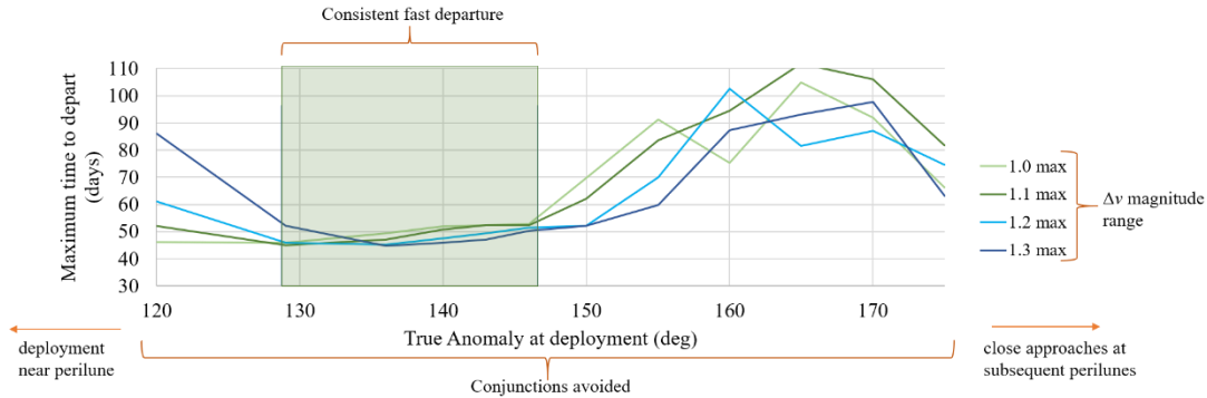
Figure 17. Green zone before apolune for deployment in the 1.5-revolution stretching direction.
