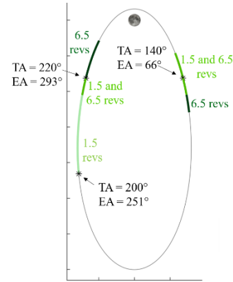
Figure 19. Candidate green zones along the NRHO.
