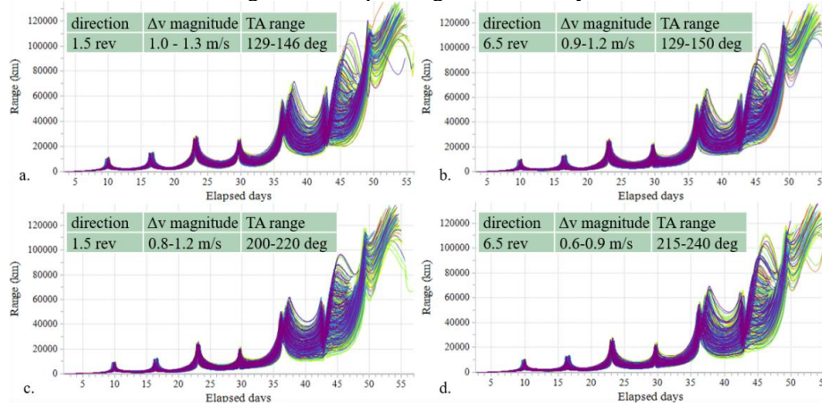
Figure 20. Gateway-cubesat range as a function of days past deployment for the candidate green zones over 56 revolutions in the NRHO. Deployment before apolune (top) and after apolune (bottom). No deployment errors considered.
