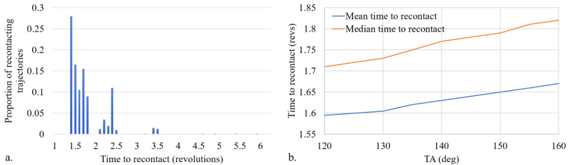
Figure 7. Histogram of recontact time for deployment in all directions from TA = 150^\circ ( EA = 84^\circ ) (a). Mean and median recontact times for deployment in all directions from 120^\circ < TA < 160^\circ (b).
