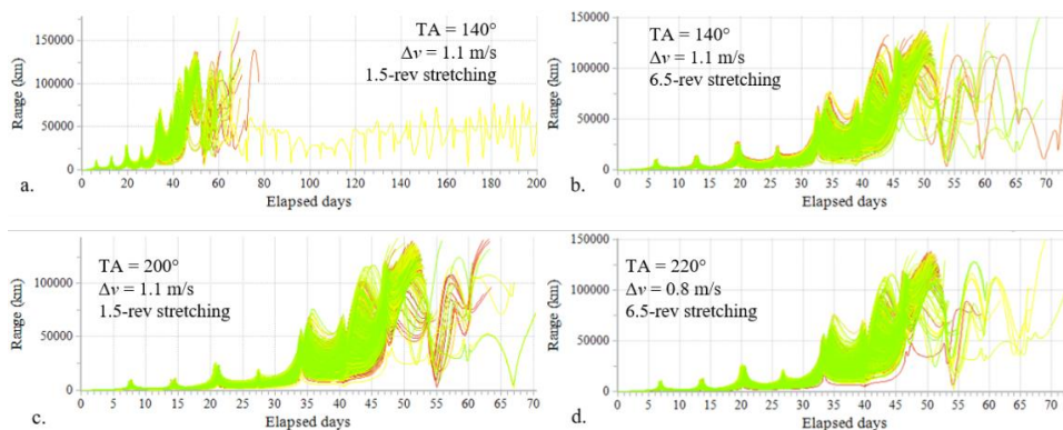
Figure 21. Gateway-cubesat range as a function of time past deployment for Monte Carlo cases A-D with large deployment execution errors.
