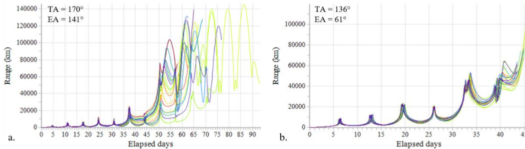
Figure 14. Cubesat deployment in the ephemeris model at the same location along the NRHO for 20 consecutive revolutions. TA = 170^\circ ( EA = 141^\circ ) (a), TA = 136^\circ ( EA = 61^\circ ) (b).
