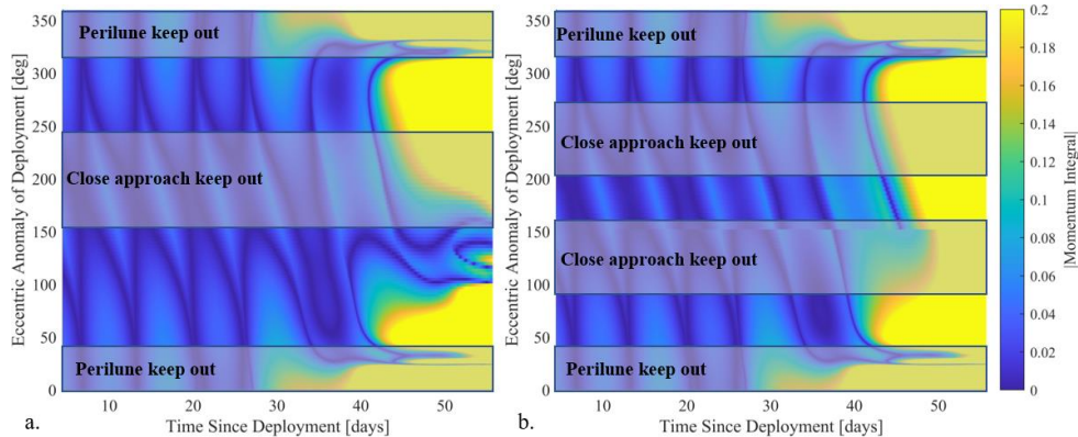
Figure 12. Momentum integral as a function of deployment EA and time past deployment in the CR3BP. Deployment in the most-stretching directions after 1.5 revolution time horizon (a) and 6.5 revolution time horizon (b) with a 1 m/s \Delta v .
