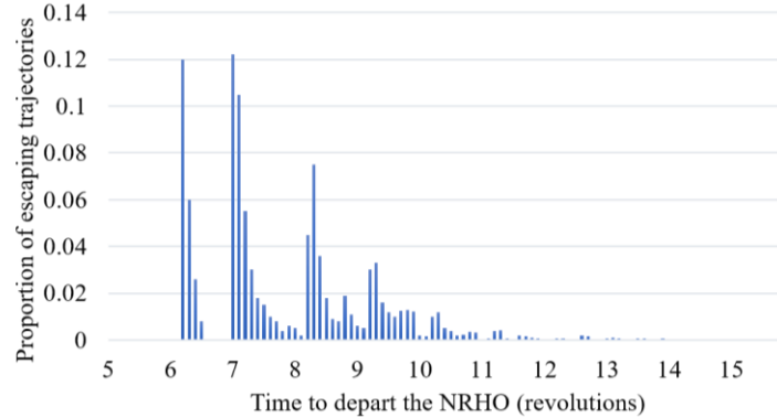
Figure 8. Histogram of time to depart the NRHO for deployment in all directions from TA = 150^\circ ( EA = 84^\circ ) in the CR3BP.
