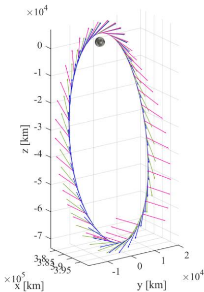
Figure 9. Stretching directions for a 1.5 (green) and 6.5 (pink) revolution time horizon, and the velocity direction (blue) plotted around the NRHO.
