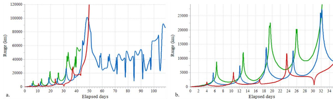
Figure 2. Gateway-cubesat range over time for three deployment cases in the ephemeris model. Full view (a) and zoomed view (b).
