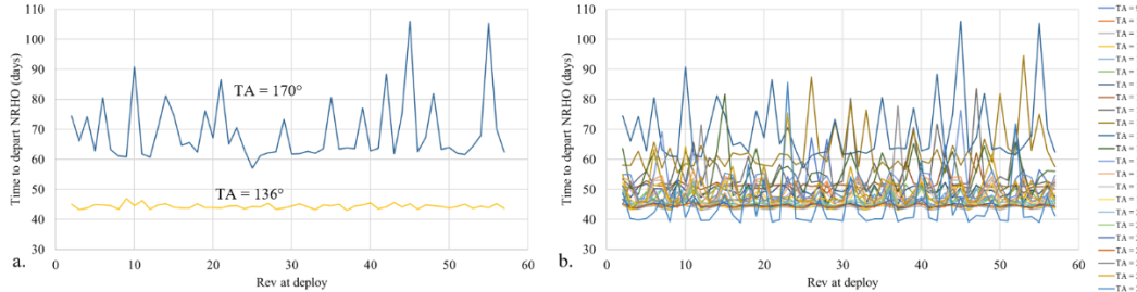
Figure 15. Time to depart the NRHO for 56 revolutions along the NRHO. Two deployment locations (a) and 30 deployment locations (b) with a 1.1 m/s \Delta v in the 1.5-revolution most-stretching direction.
