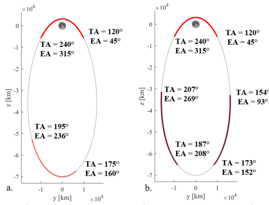
Figure 11. Keep-out regions for deployment in the most-stretching directions after a 1.5 revolution time horizon (a) and a 6.5 revolution time horizon (b).
