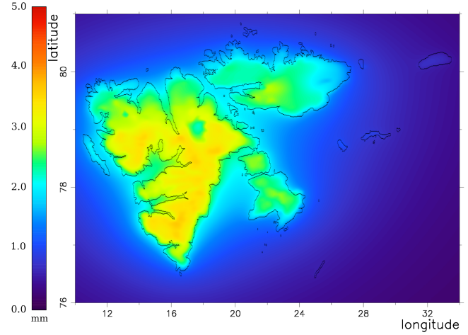
Figure 2. Crustal deformations due to glacier and snow loading according to the CMB model. The panels are: the rate of change (left) and annual signal (right). Important: the CMB model does not account for mass loss due to frontal ablation and calving.
