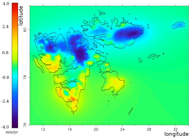
Figure 2. Crustal deformations due to glacier and snow loading according to the CMB model. The panels are: the rate of change (left) and annual signal (right). Important: the CMB model does not account for mass loss due to frontal ablation and calving.
