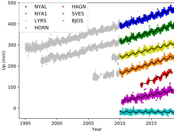
Figure 3. GNSS vertical time-series for the Gamit-NMA solutions. The color coded time span is the data period used in this study. The black curves are the model function fitted to this period. The HORN station was moved to a new location in 2009. The time series are shifted with respect to each other to improve readability.
