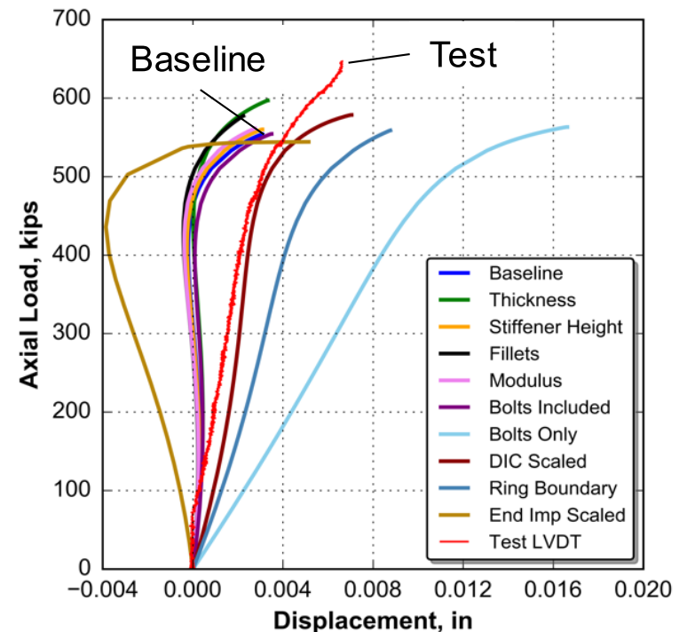
Load vs. weld land radial displacement response
