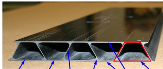
Long span Short span Web Noodle Flute Facesheets
