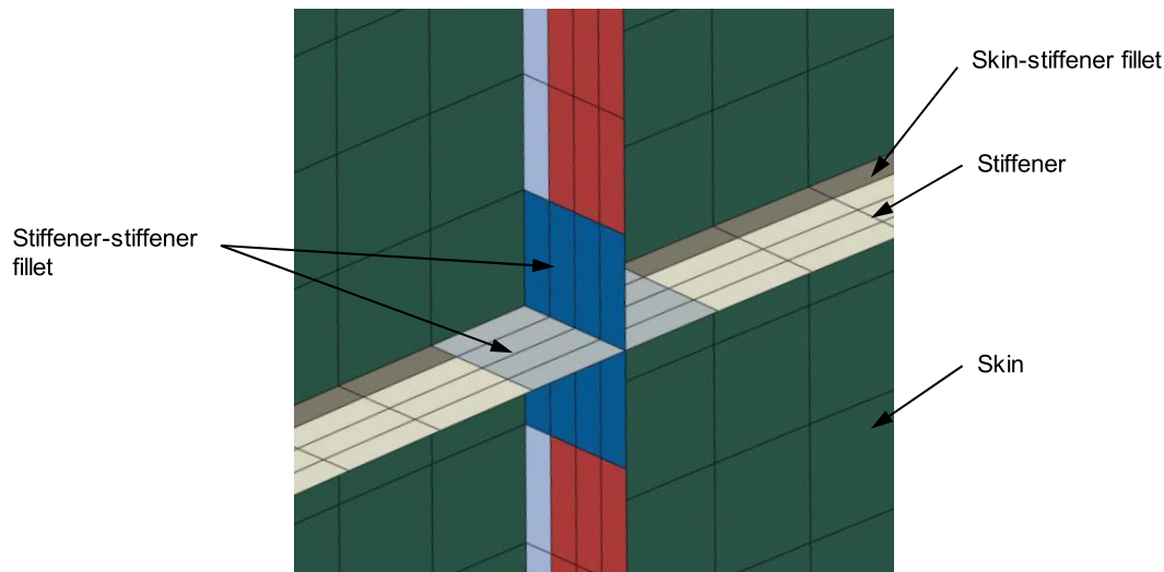
Shell model
