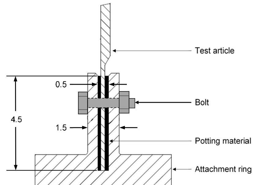
attachment ring cross-section
