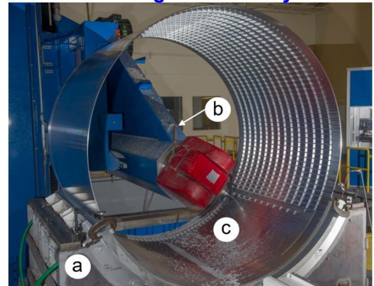
Machining seamless cylinder
