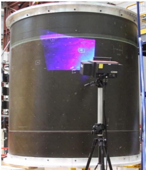
As-manufactured state (structured light scanning)
