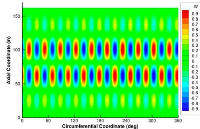
(a) Without weld lands.
