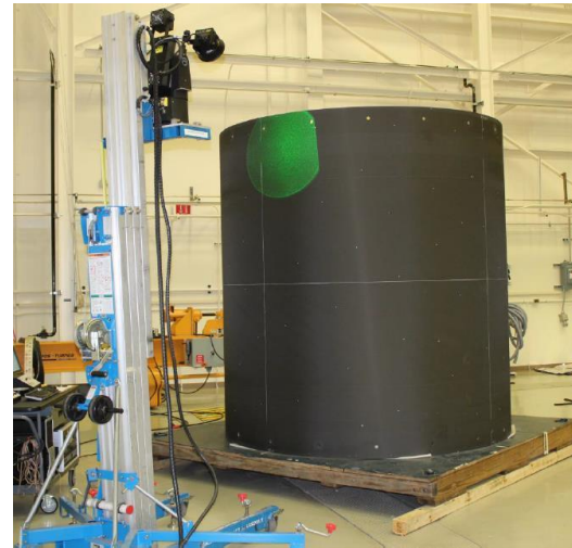
Thermal shearography
