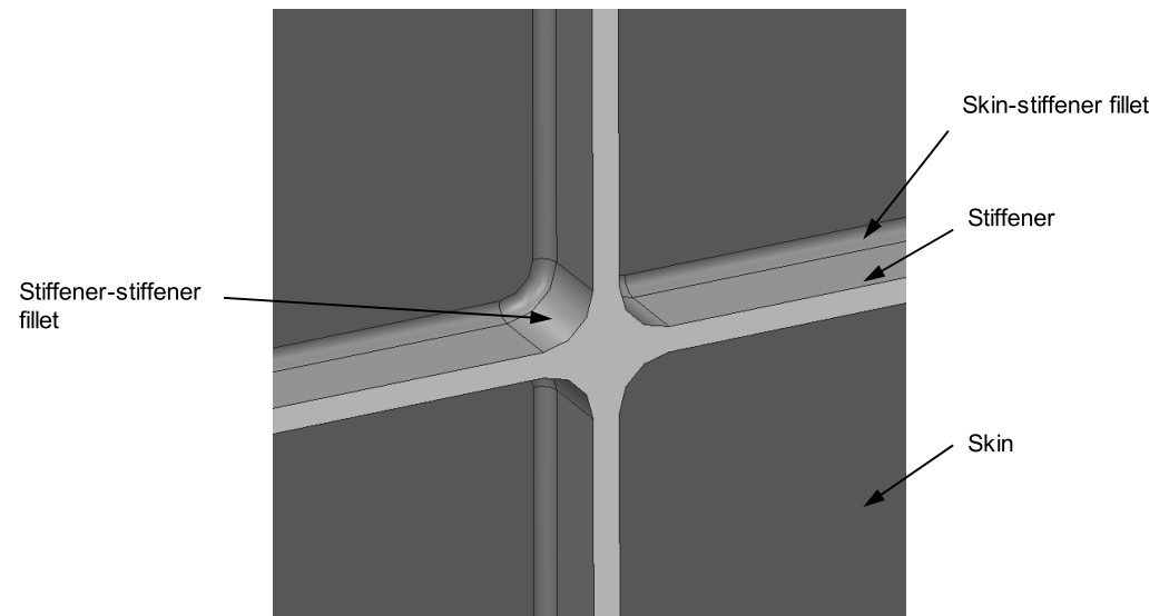
Solid model
