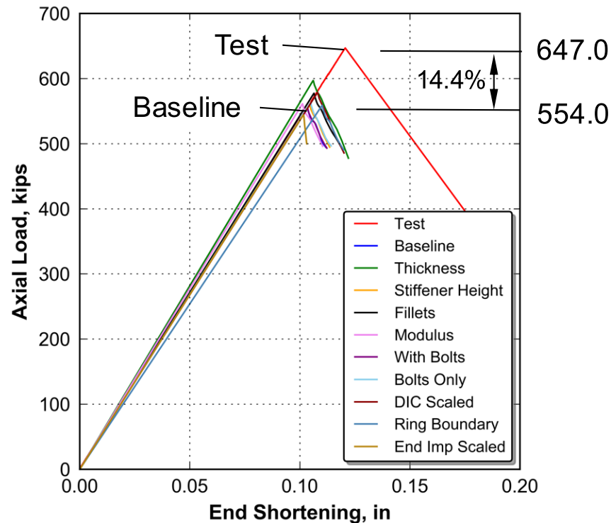
Load vs. end-shortening response
