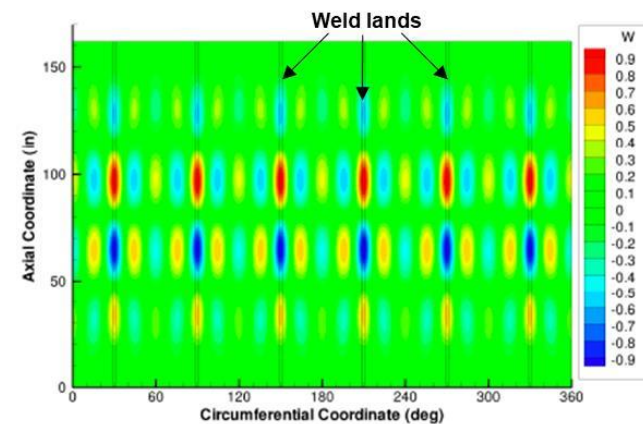
(b) With axial weld lands.
