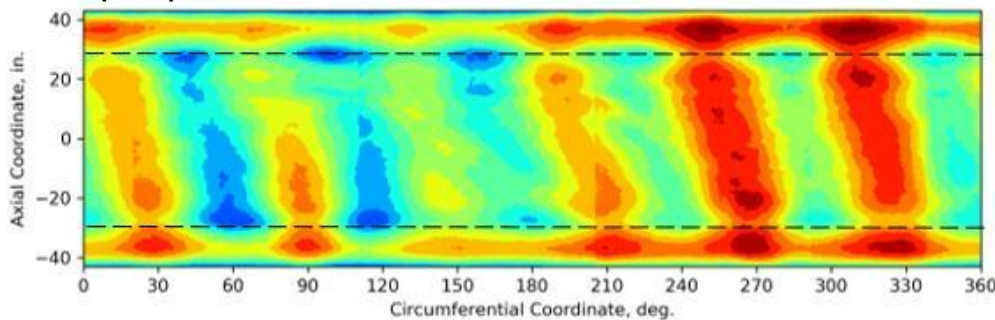
Test (DIC)
