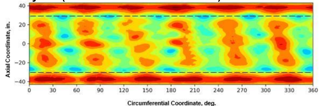
Analysis (As-installed state at tare load)
