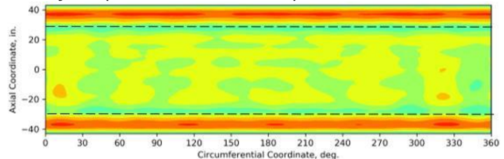
Analysis (As-installed state at tare load)
