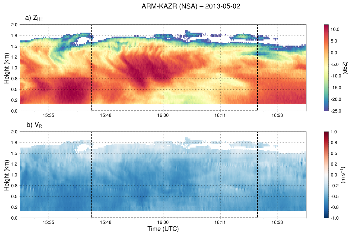
FIG. 6. KAZR time-height observations of a) Z and b) MDV between 15:30 UTC and 16:30 UTC at the ARM NSA site on 2 May 2013. The dashed black outline indicates the averaging region for the mean profiles shown in Fig. 7.
