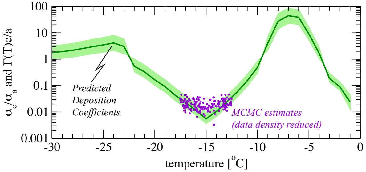
FIG. 11. Ratio of deposition coefficients for the c- and a-axes of crystals extracted from wind tunnel measurements of ice crystal growth at liquid saturation and constant temperature (green solid curve) and the uncertainty range (green shade) from (Harrington et al. 2019). Purple points are \Gamma \times \phi from the MCMC parameter PDF. For clarity, only a subset of the points from the PDF are shown and these are scattered randomly over the temperature range of the observed cloud layer (-12 to -18 ^{\circ}\text{C} .)
