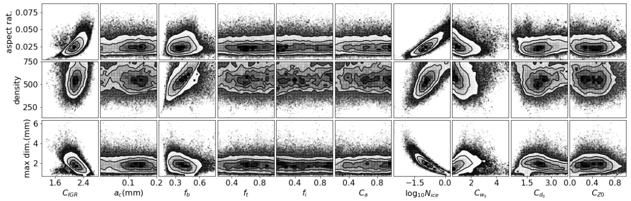
FIG. 12. Joint posterior PDF of parameters and microphysical quantities: aspect ratio, density, and number-weighted maximum diameter, respectively, from top to bottom. The shading and contours are as described for Fig. 10.
