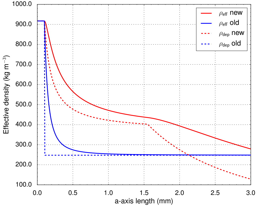
FIG. 1. Plot of deposition density (dashed lines) and effective density (solid lines) for a crystal at sizes of a = 0.01 to a = 3.0 using the deposition density model developed herein (red) and the deposition density model of Jensen and Harrington (2015), with a_c = 0.1 mm and \rho_{\text{dep}} \approx 250 kg m -3 . The crystal structure quantities for the deposition density shown here are a_c = 0.1 mm, f_b = 0.4 , f_i = 0.5 , and f_t = 0.3 .
