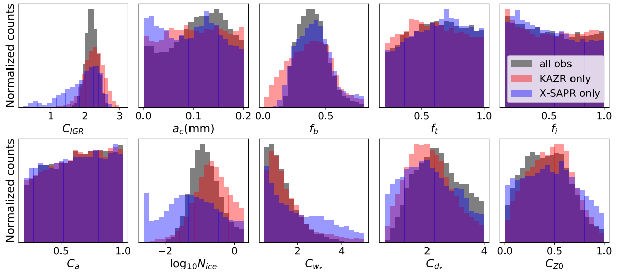
FIG. 17. Marginal PDFs of parameters for experiments using both KAZR and X-SAPR as constraints (grey), KAZR-only as a constraint (red), and X-SAPR-only as a constraint (blue).
