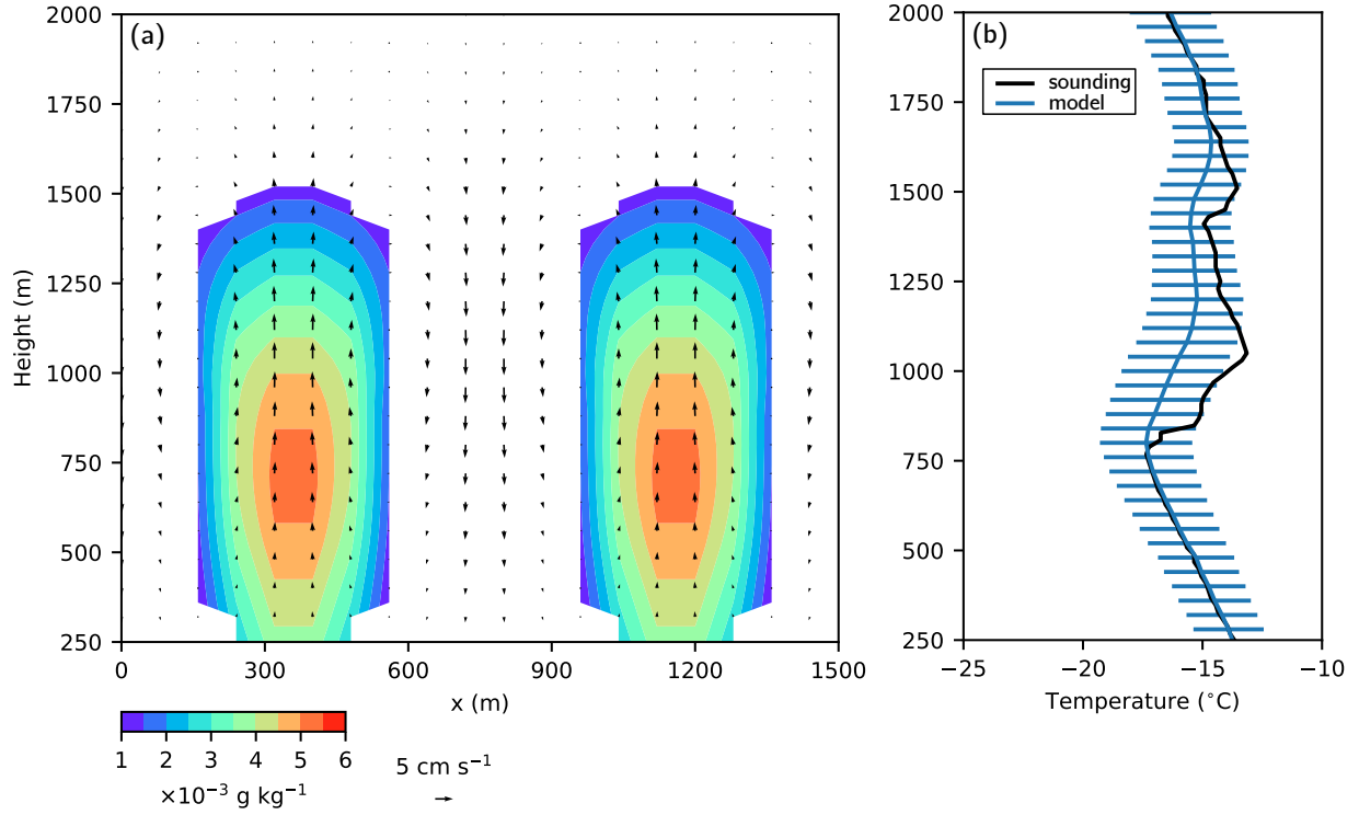
FIG. 4. Plot of a) mean wind vectors and mean ice mass mixing ratio (shaded contours) and b) simulated mean temperature profiles (blue; observed sounding from 17:30 UTC in black), with bars indicating the 1-\sigma ranges from 100 simulations using unique samples of the parameters drawn from the posterior MCMC distribution. The temperature profiles correspond to vertical profiles at x = 320 \text{ m} .
