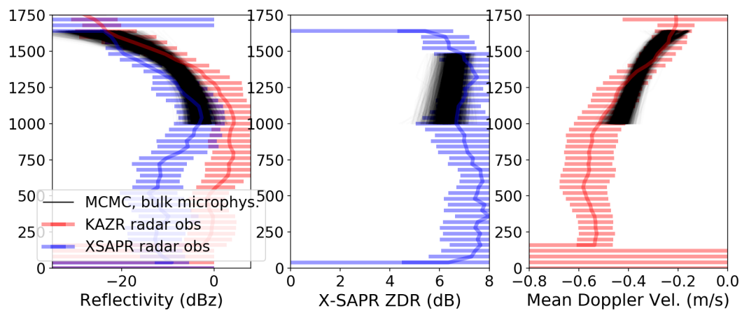
FIG. 7. KAZR observations (red, with 1- \sigma errors), X-SAPR observations (blue, with 1- \sigma errors) and forward-simulated observations (black) drawn from posterior distribution of model solutions.
