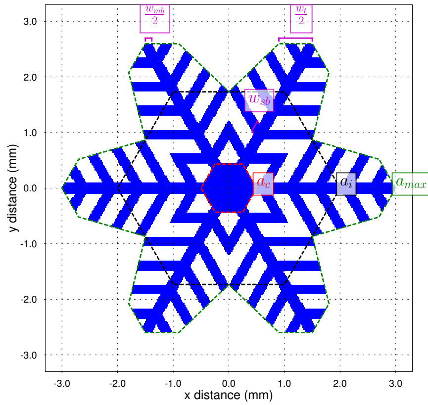
Fig. A1. Plot of crystal regions. Adapted from SK19.
