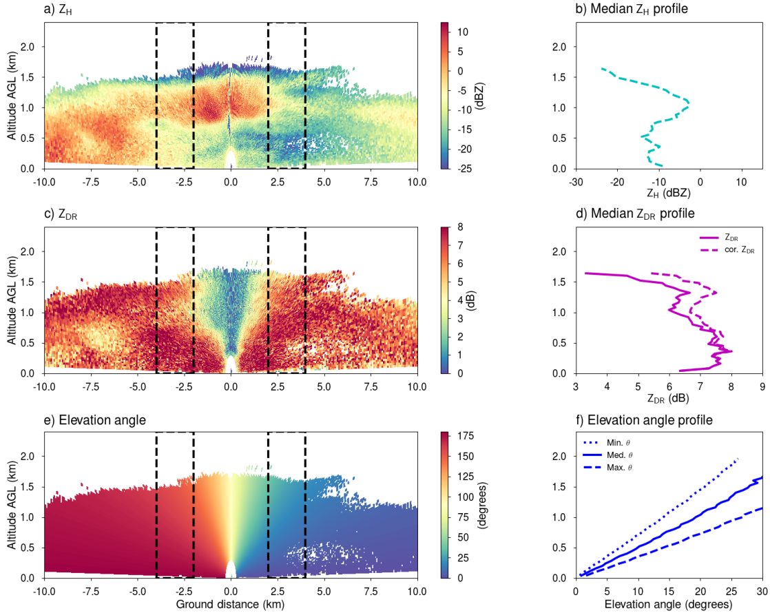
FIG. 5. 7°-azimuth HRHI observations of a) Z , c) Z_{DR} , and e) the corresponding elevation angles from the X-SAPR radar at the ARM NSA site on 2 May 2013 at 15:54 UTC. The median profiles are for Z , Z_{DR} , and elevation angle are plotted in panels b), d), and f), respectively, where the values are binned within the observational domains indicated by the black outlines in the HRHI panels at each height. Panel d) includes the median Z_{DR} (solid line) and the corrected median Z_{DR} (dashed line) based on the median elevation angle at each height. Specifically, the median Z_{DR} is divided by the cosine squared of the median elevation angle at each height. The bounds of the elevation angles at each height within the observational domains are shown plotted as the dashed lines in panel f).
