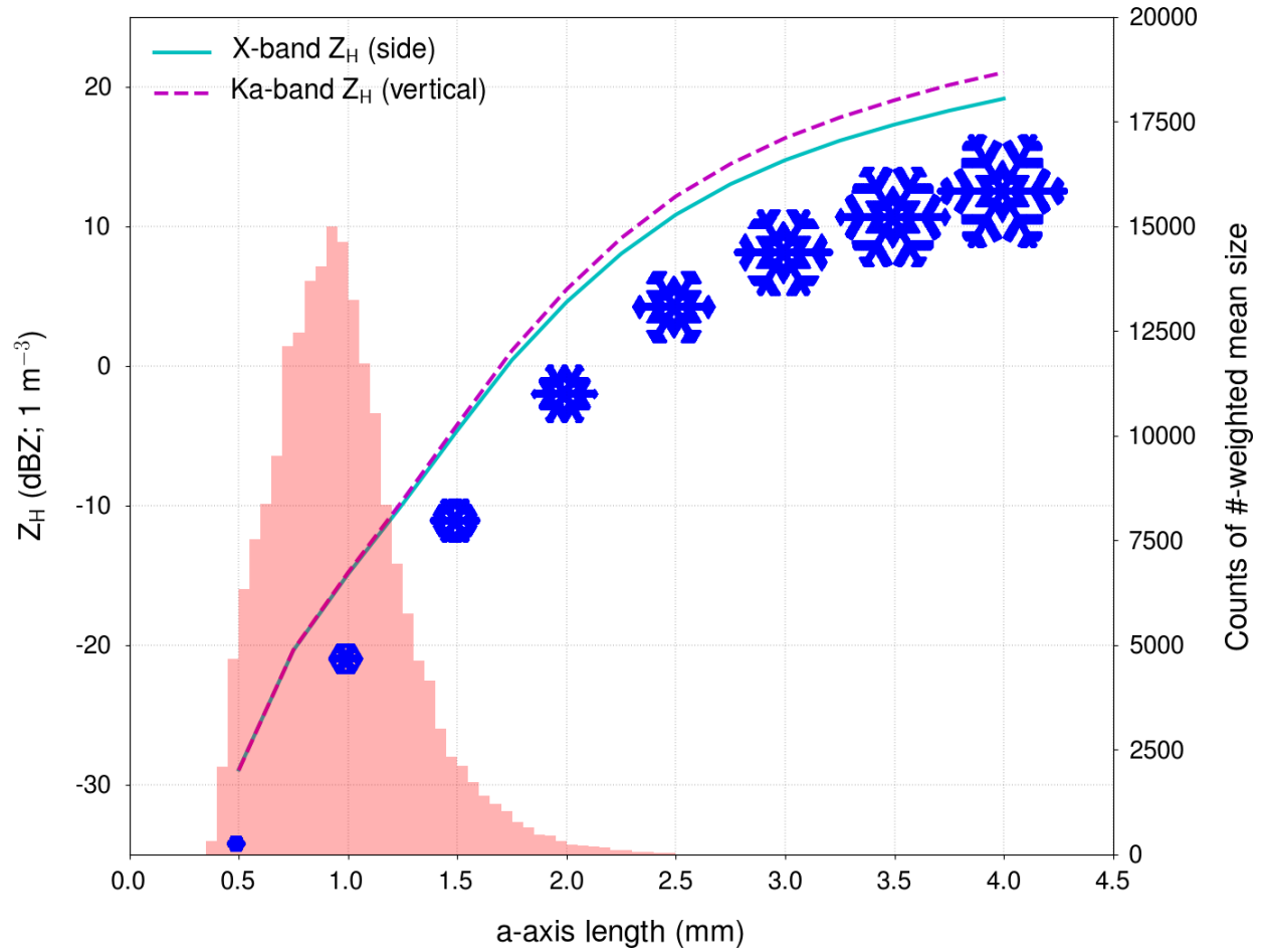
FIG. 8. Comparison of Z given 1 \text{ m}^{-3} crystals growing from a = 0.5 \text{ mm} to a = 4.0 \text{ mm} for X band at side incidence (solid cyan line; corresponding to X-SAPR) and Ka band at vertical incidence (dashed magenta line; corresponding to KAZR). The 2D ice crystal structures used in the Amsterdam Discrete Dipole Approximation (ADDA; Yurkin and Hoekstra 2011) calculations are plotted in blue. An overlay of the histogram of number-weighted mean a-axis lengths from the MCMC simulations is plotted in red.
