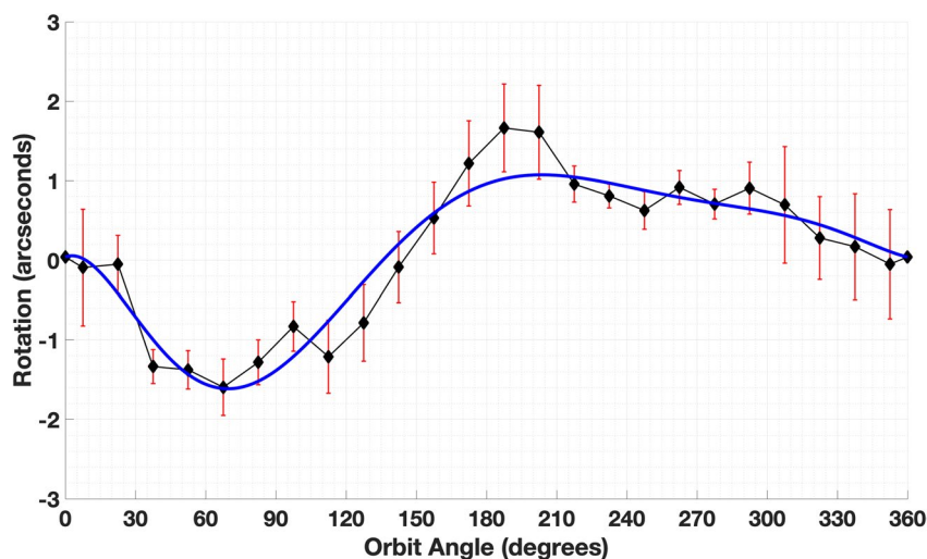
Figure 7. Calibrated pitch orbital variation for CAL Period 19. Orbit angle is the angle between the satellite position vector and the sun vector projected in the orbit plane where for this analysis 0^\circ is orbit 6 a.m., 90^\circ is orbit noon, 180^\circ is orbit 6 p.m., and 270^\circ is orbit midnight. The blue line is the functional fit used to calibrate the pointing. It should be noted the ICESat-2 ANC products have a different orbit angle convention with 0^\circ being midnight. ICESat-2, Ice Cloud and Land Elevation Satellite.
