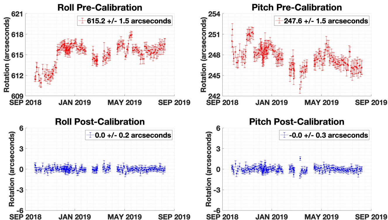
Figure 8. ICESat-2 time varying pointing error pre and post-calibration and correction. The bars represent the standard deviation of the orbital variation per calibration. ICESat-2, Ice Cloud and Land Elevation Satellite.
