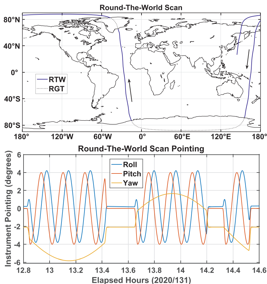
Figure 2. Example of noninterfering ICESat-2 “round”-the-world scans (RTWS). Geographic path of scan maneuver (top), and spacecraft roll and pitch time series (bottom). Time periods where roll and pitch are near zero are during nominal RGT pointing over ice sheets. An Ocean Scan (OS) samples the same ocean tracks as RTWSs but is limited to 20 min confined within \pm 40^\circ latitude centered on the equator over the Pacific ocean. OS, Ocean Scan; RGT, reference ground track; RTWS, “round”-the-world scans.
