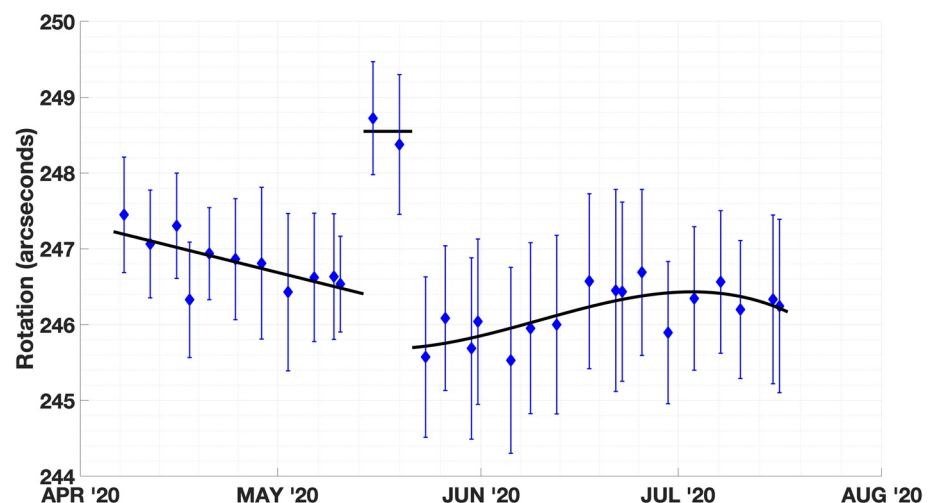
Figure 6. Pitch pointing bias trend calibration for CAL Periods 17–19. Blue markers represent individual bias calibrations. Bars represent the standard deviation of the orbit angle variation observed by the individual 24-h calibration. The black line is the functional fit of the bias trend. The discontinuities occur at the CAL Period boundaries and are due to the yaw flip and AMCS setpoint change. 1 arcsecond of pointing error is approximately 2.4 m of geolocation error on the Earth's surface. AMCS, Alignment Monitoring and Control System.
