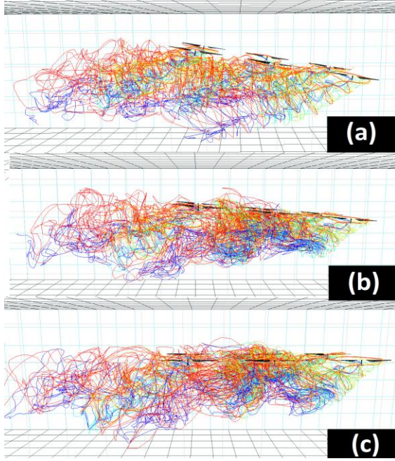
Figure 34. Simulated wake interactions for the six-rotor - Short configuration: (a) -10 deg (b) -5 deg, and (c) 0 deg pitch angle at forward flight of 20 ft/s.
