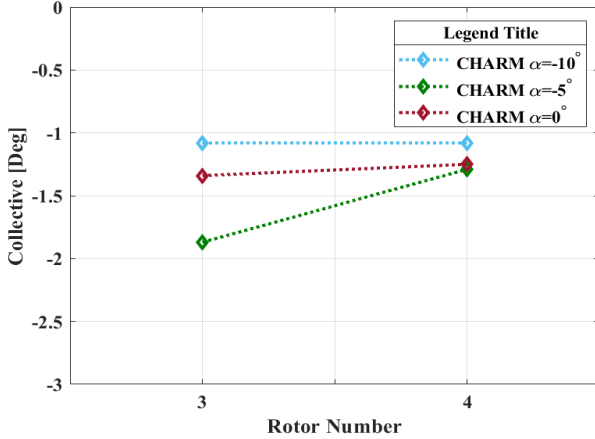
Figure 15. The collective values for individual rotors at pitch angle of -10, -5, and 0 deg, for two-rotors in the wind tunnel in forward flight of 20 ft/s.
