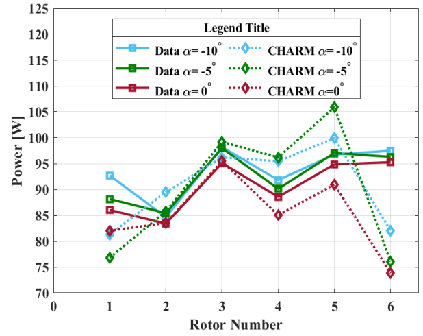
Figure 31. Measured and computed power values for individual rotors at 20 ft/s and pitch angle of -10, -5, and 0 deg for six-rotors, Short configuration.
