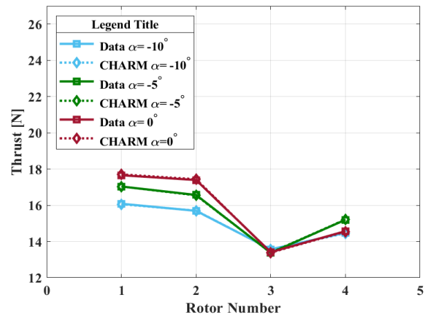
Figure 20. Measured and computed thrust values for individual rotors at 20 ft/s and pitch angle of -10, -5, and 0 deg for four-rotors.
