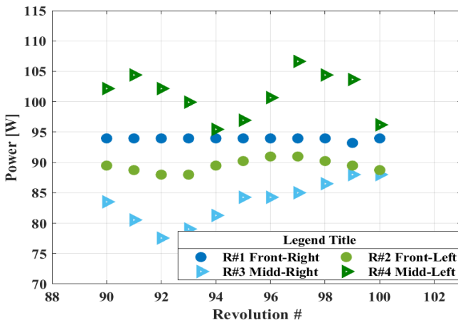
Figure 27. CHARM power variation over last 10 rotor revolutions (total 100 revolutions) with wind tunnel walls: pitch angle of 0 deg; 20 ft/s; for four-rotor case.
