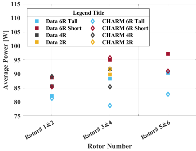
Figure 44. The average power of front, middle and back rotors at different MTB configuration at tunnel speed of 20 ft/s and -10 deg pitch angle.
