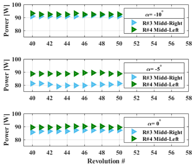
Figure 18. CHARM power variation over last 10 rotor revolutions: pitch angle of -10, -5, and 0 deg; 20 ft/s; Rotors 3 and 4.
