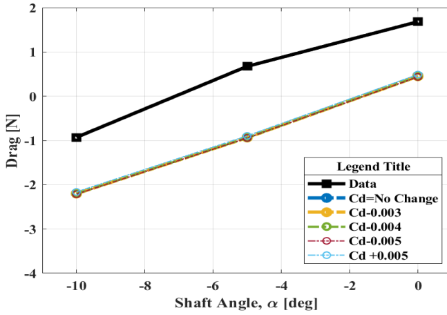
Figure 11. Effect of different \Delta c_d on CHARM drag predictions. Single rotor (Rotor #2) cases in the wind tunnel for forward speed of 20 ft/s.
