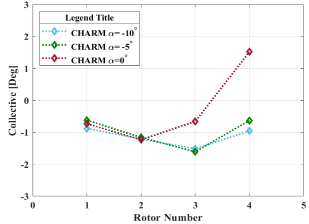
Figure 19. The collective values for individual rotors at 20ft/s and pitch angle of -10, -5, and 0 deg, for four-rotors.
