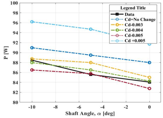
Figure 9. The comparison of the data power versus the CHARM with different \Delta c_d - single rotor cases in the wind tunnel at 20 ft/s.
