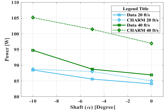
Figure 14. Predicted rotor power values after applying \Delta c_d = -0.003 to the airfoil tables. Single rotor cases in the wind tunnel for forward speeds of 20 and 40 ft/s.
