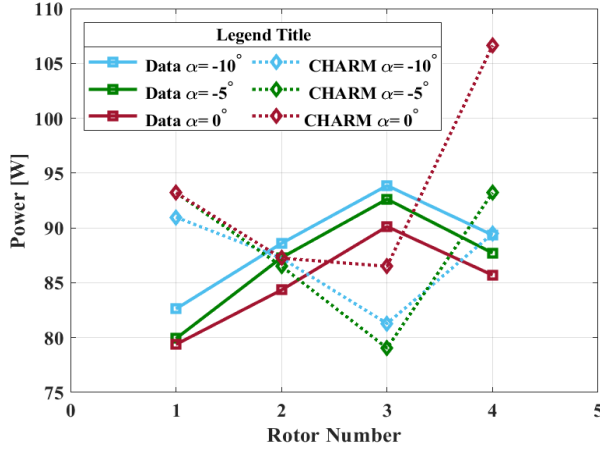
Figure 21. Measured and computed power values for individual rotors at 20 ft/s and pitch angle of -10, -5, and 0 deg for four-rotors.
