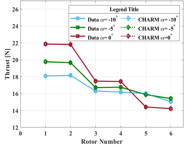
Figure 32. Measured and computed thrust values for individual rotors at c and pitch angle of -10, -5, and 0 deg for six-rotors, Short configuration.
