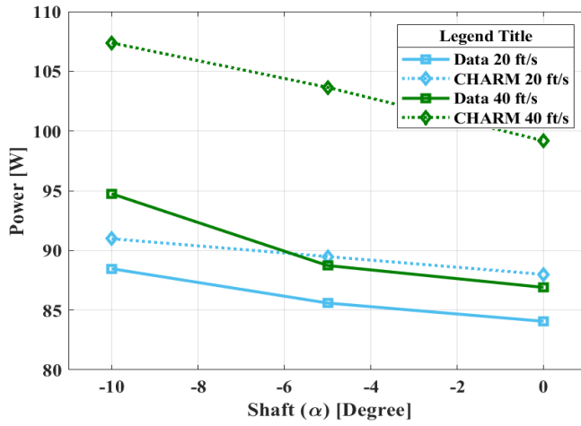
Figure 8. The rotor power values for single rotor cases at wind tunnel in forward flight at 20 and 40 ft/s.
