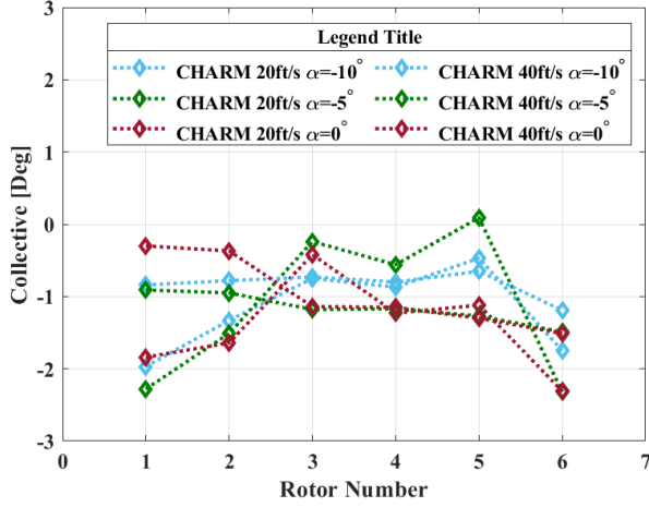
Figure 29. The collective values for individual rotors at pitch angle of -10, -5, and 0 deg, for six-rotors, Short configuration in forward flight of 20 ft/s and 40 ft/s.
