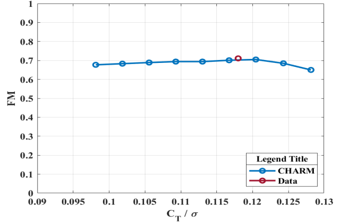
Figure 5. Single rotor in hover – Figure of Merit vs C_T/\sigma .
