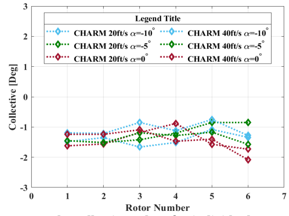
Figure 35. The collective values for individual rotors at pitch angle of -10, -5, and 0 deg, for six-rotors, Tall configuration in forward flight of 20 ft/s and 40 ft/s.
