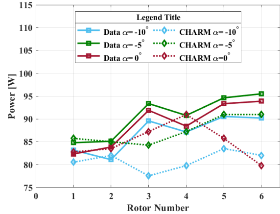
Figure 37. Measured and computed power values for individual rotors at 20 ft/s and pitch angle of -10, -5, and 0 deg for six-rotors, Tall configuration.
