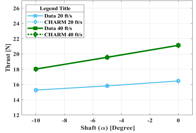
Figure 13. Predicted rotor thrust values after applying \Delta c_d = -0.003 to the airfoil tables. Single rotor cases in the wind tunnel for forward speeds of 20 and 40 ft/s.
