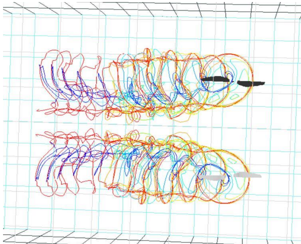
Figure B1. Two-rotor cases at forward flight 20 ft/s in wind tunnel with pitch-10 degrees.
