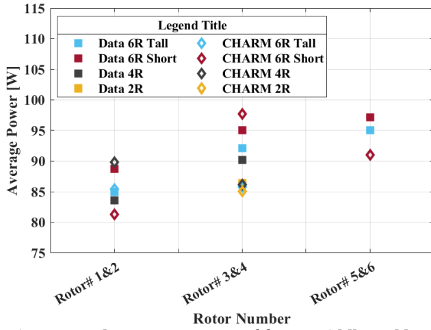
Figure 45. The average power of front, middle and back rotors at different MTB configuration at tunnel speed of 20 ft/s and -5 deg pitch angle.
