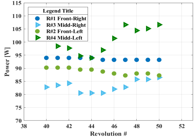
Figure 23. CHARM power variation over last 10 rotor revolutions (total 50 revolutions) with wind tunnel walls: pitch angle of 0 deg; 20 ft/s; Rotors 1, 2, 3 and 4.
