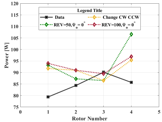
Figure 28. The power prediction for Rotor #4: pitch angle of 0 deg; 20 ft/s; for four-rotor case.
