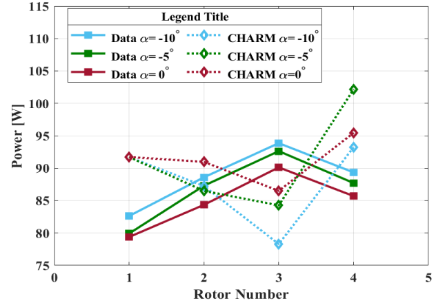
Figure 22. Measured and computed power values for four-rotor case after changing the rotor rotation direction in CHARM at 20 ft/s and pitch angle of -10, -5, and 0 deg.
