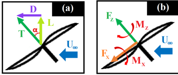
Figure 4. Aerodynamic forces and moments on a rotor disk tilted aft: (a) forces, (b) forces and moments.
