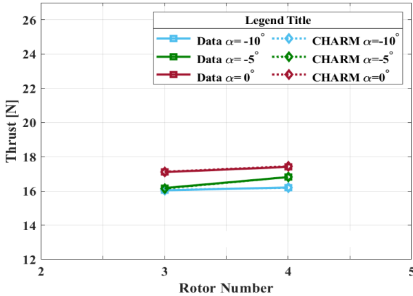
Figure 16. Measured and computed thrust values for individual at pitch angle of -10, -5, and 0 deg, for two-rotor case in the wind tunnel at speed of 20 ft/s.
