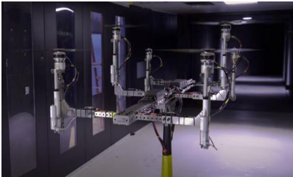
Figure 1. Multirotor Test Bed (MTB) in the 7- by 10-Foot Wind Tunnel at Ames Research Center.
