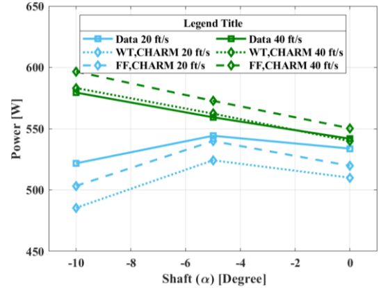
Figure 41. Power comparison between the data, wind tunnel (WT) prediction and the free field (FF) prediction for six-rotor cases in the Tall configuration.
