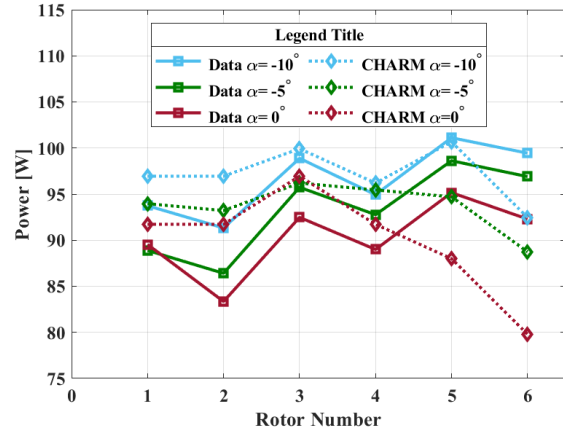
Figure 39. Measured and computed power values for individual rotors at 40 ft/s and pitch angle of -10, -5, and 0 deg for six-rotors, Tall configuration.
