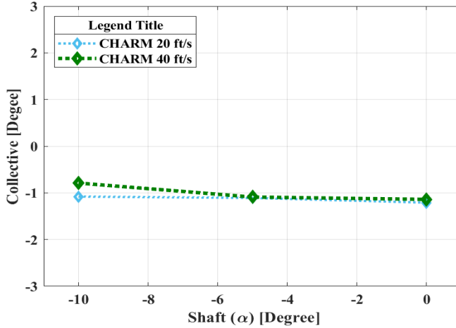
Figure 12. Predicted rotor collective values after applying \Delta c_d = -0.003 to the airfoil tables. Single rotor (Rotor #2) cases in the wind tunnel for forward speeds of 20 ft/s and 40 ft/s.
