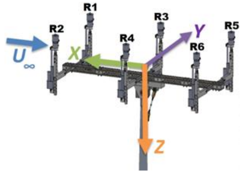
Figure 3. CHARM coordinate system for the MTB.
