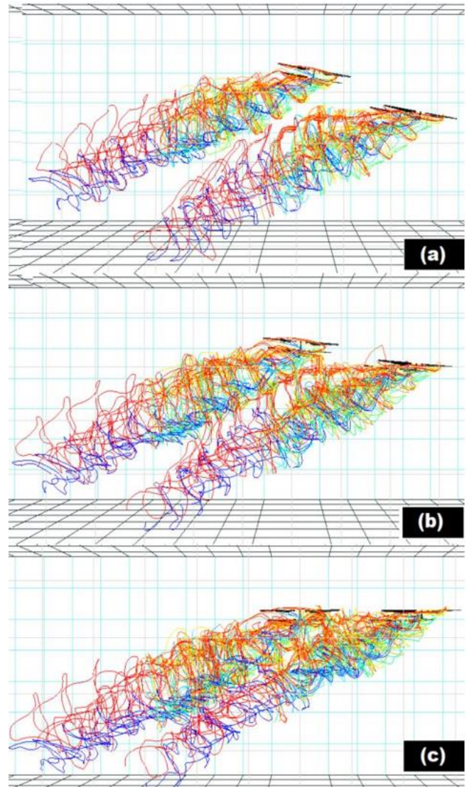
Figure B3. Four-rotor cases at forward flight 20 ft/s in wind tunnel - side view - pitch angle (a) -10 degrees (b) -5 degrees (c) 0 degrees.
