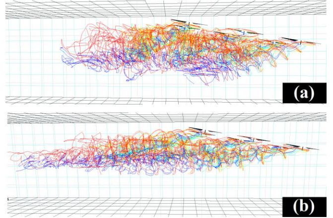
Figure 40. Six-rotor, Tall configuration: wake interactions at -10 deg pitch angle (a) 20 ft/s, (b) 40 ft/s.
