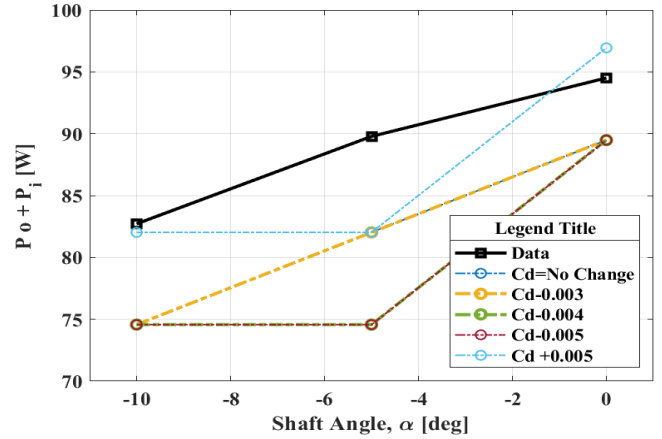
Figure 10. The comparison of the data P_i + P_o versus the CHARM with different \Delta c_d - single rotor cases in the wind tunnel in forward flight at 20 ft/s.
