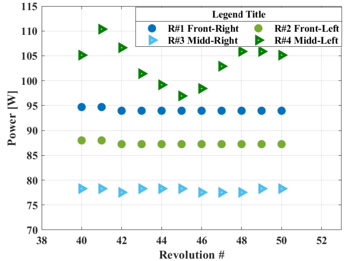
Figure D2. CHARM power variation over last 10 rotor revolutions (total 50 revolutions) with wind tunnel walls: pitch angle of -5 deg; 20 ft/s; four-rotor case.
