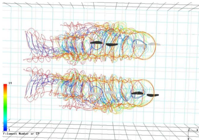
Figure 26. Four-rotor cases at forward flight 20 ft/s in wind tunnel with pitch -10 degrees.
