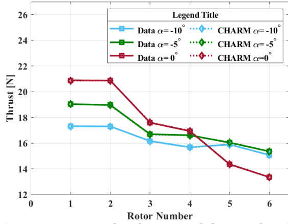
Figure 38. Measured and computed thrust values for individual rotors at 40 ft/s and pitch angle of -10, -5, and 0 deg for six-rotors, Tall configuration.
