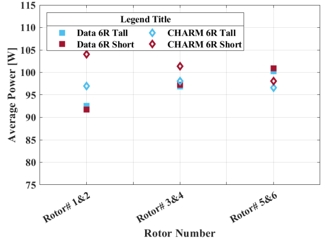
Figure 47. The average power of front, middle and back rotors at different MTB configuration at tunnel speed of 40 ft/s and -10 deg pitch angle.
