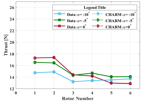
Figure 36. Measured and computed thrust values for individual rotors at 20 ft/s and pitch angle of -10, -5, and 0 deg for six-rotors, Tall configuration.
