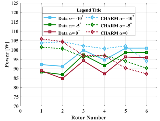
Figure 33. Measured and computed power values for individual rotors at 40 ft/s and pitch angle of -10, -5, and 0 deg for six-rotors, Short configuration.
