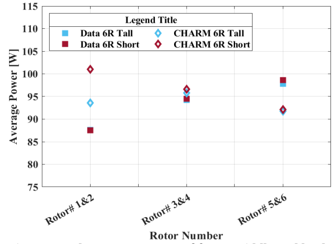
Figure 48. The average power of front, middle and back rotors at different MTB configuration at tunnel speed of 40 ft/s and -5 deg pitch angle.
