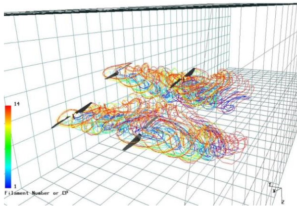
Figure B2. Flow visualization of rotors numbers 1-4 in the short rotor configuration, at the -10 degrees pitch angle, and with a wind tunnel speed of 20 ft/s.
