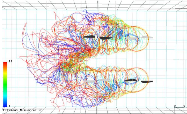
Figure 25. Four-rotor cases at forward flight 20 ft/s in wind tunnel with pitch 0 degrees.
