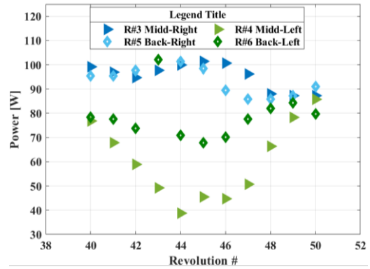
Figure 43. The power values for the last 10 revolution of the six-rotor case at Tall configuration and 0 deg pitch angle at the wind tunnel speed of 20 ft/s.
