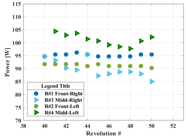
Figure 24. CHARM power variation over last 10 rotor revolutions (total 50 revolutions) without wind tunnel walls: pitch angle of 0 deg; 20 ft/s; Rotors 1, 2, 3 and 4.
