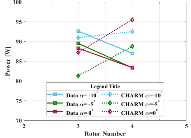
Figure 17. Measured and computed power values for individual at pitch angle of -10, -5, and 0 deg, for two-rotor case in the wind tunnel at speed of 20 ft/s.
