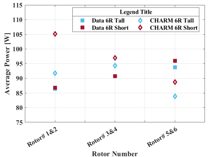
Figure 49. The average power of front, middle and back rotors at different MTB configuration at tunnel speed of 40 ft/s and 0 deg pitch angle.
