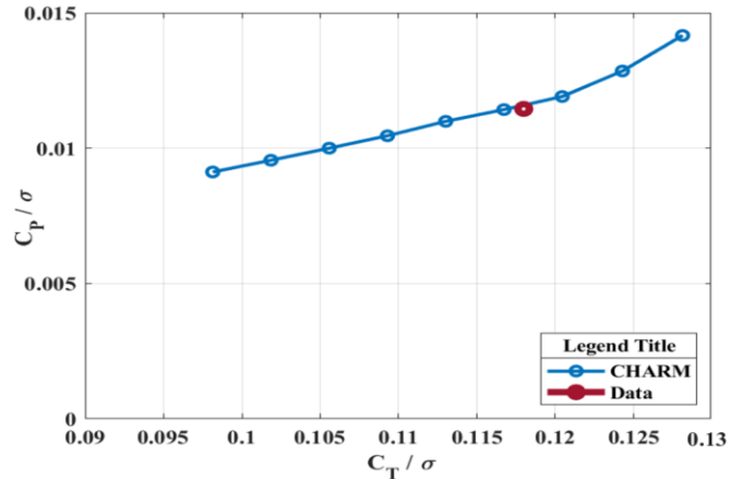
Figure 6. Single rotor in hover – C_p/\sigma vs C_T/\sigma .
