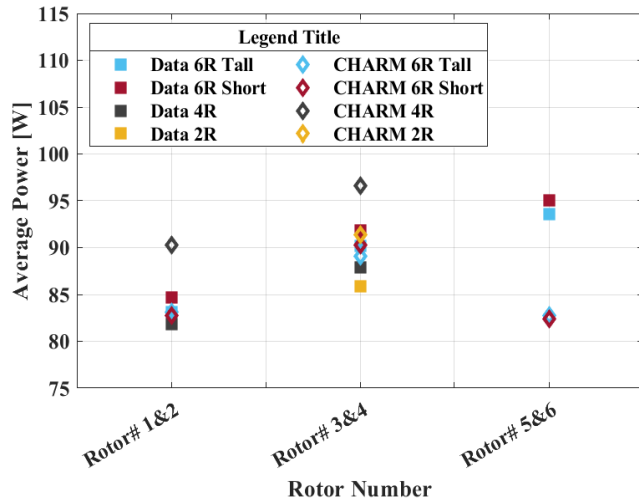
Figure 46. The average power of front, middle and back rotors at different MTB configuration at tunnel speed of 20 ft/s and 0 deg pitch angle.
