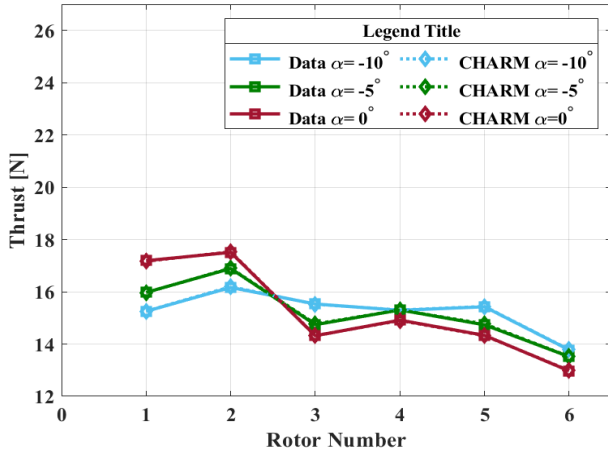
Figure 30. Measured and computed thrust values for individual rotors at 20 ft/s and pitch angle of -10, -5, and 0 deg for six-rotors, Short configuration.
