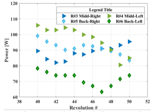
Figure 42. The power values for the last 10 revolution of the six-rotor case at Short configuration and 0 deg pitch angle at the wind tunnel speed of 20 ft/s.
