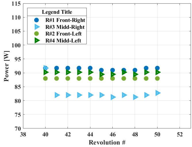
Figure D1. CHARM power variation over last 10 rotor revolutions (total 50 revolutions) with wind tunnel walls: pitch angle of -10 deg; 20 ft/s; four-rotor case.
