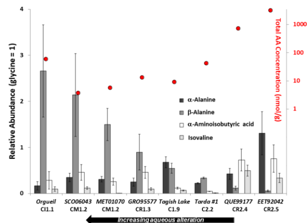
Figure 1. Total amino acid concentrations and relative amino acid abundances in the C2 ungrouped Tagish Lake and Tarda meteorites and several CI, CM, and CR chondrites. The arrow represents increasing aqueous alteration as inferred from the meteorite petrologic type assignments based on the amount of bulk H in OH and H 2 O [9].
