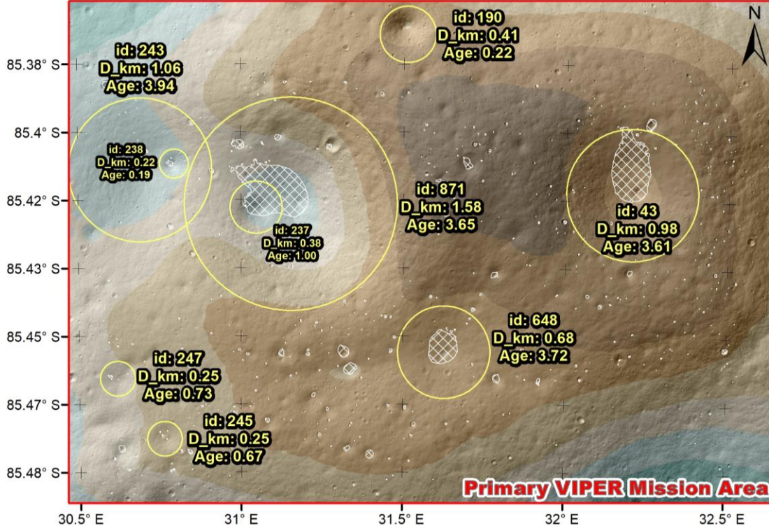
Figure 1. Nine of the largest craters in the currently mission area with degradation-derived age estimates. Hashed regions are PSRs (note there is a PSR in the crater with id 190 as well). The three craters (Fig. 2) with the largest PSRs on the Nobile plateau are all interpreted as Imbrian based on their degradation state. The largest crater, id 871, has a younger crater, id 237, that formed on its interior floor and subsequently altered the shape of its PSR. All smaller PSRs (<500 m) are younger (<~1 Ga), as expected.
