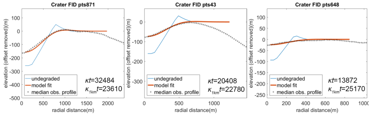
Figure 2. Diffusive fits to the craters with the three largest PSRs in the VIPER mission area. The \kappa t values are model fits, with \kappa_{1km} t values reporting the equivalent degradation state renormalizing to a constant 1-km scale (see eq. 2). (Blue: model fresh crater profile; Orange: model diffused crater profile; Crosses: Median observed crater topography.)
