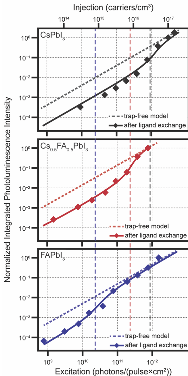
Figure 4. Normalized integrated photoluminescence intensity (data points) versus excitation fluence with model results (lines) for CsPbI 3 (black), Cs 0.5 FA 0.5 PbI 3 (red), and FAPbI 3 (blue) PQD films. The trap density derived from the model results are plotted as vertical dashed lines.
