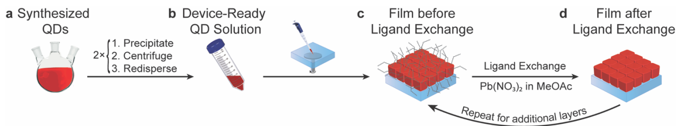
Figure 1. Preparation of \text{CsPbI}_3 quantum dots and films. (a) As-synthesized QDs were isolated from excess precursors by precipitation and centrifugation to prepare (b) device-ready QDs. The device-ready QDs were deposited via spincoating to form (c) films with a high density of long-chain ligands. Ligand exchange with \text{Pb}(\text{NO}_3)_2 in MeOAc formed a (d) film of device-ready QDs with increased charge carrier mobility.
