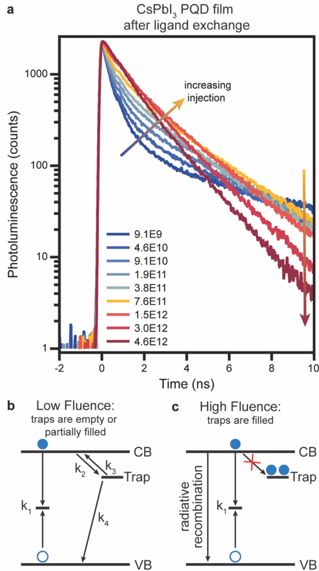
Figure 3. (a) TRPL data for CsPbI 3 PQD films after ligand exchange with varying 470 nm excitation
