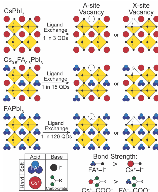
Figure 5. Trap formation in CsPbI 3 , Cs 0.5 FA 0.5 PbI 3 , and FAPbI 3 QDs, labeled with the average number of QDs with a trap for each QD composition. The relative hardness of formamidinium, iodide, cesium and carboxylate ions is labeled, leading to the relative bond strengths.
