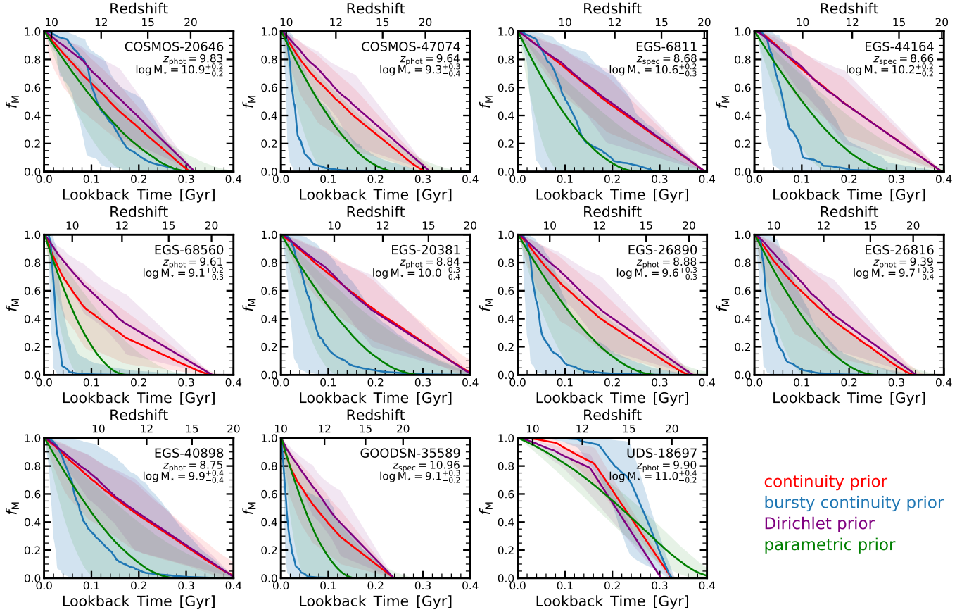
Figure 12. Star-formation histories (SFHs) obtained from Prospector assuming different priors. The SFHs are plotted as a fraction of stellar mass formed. The adopted priors include the continuity prior (red), bursty continuity prior (blue), Dirichlet prior (purple) and parametric prior. These priors are discussed in Section 3.2. The lines and shaded regions show the median and 16-84th percentile of the SFH posterior, respectively. In most cases (exception is the most massive galaxy UDS-18697), the bursty continuity prior leads to more recent star formation than the continuity and Dirichlet priors, which both roughly follow a constant SFH. The parametric prior lies in between those extrema. The data does not prefer any of those priors: Bayes factor for all models with respect to each other roughly 1, highlighting that the adopted prior heavily effects the resulting posterior SFH.
