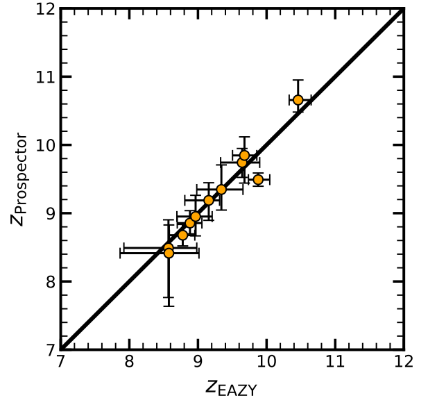
Figure 5. A comparison of the Prospector-based photometric redshifts to the EAZY-based photometric redshifts from F21. The points with the errorbars indicate the median and 16-84th percentiles for the redshift posterior after marginalizing over all other SED parameters. We find good agreement between the Prospector-based and EAZY-based photometric redshifts.
