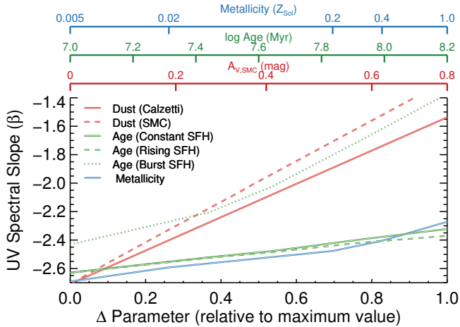
Figure 6. The dependence of the UV spectral slope \beta on individual galaxy physical properties. The horizontal axis shows the fractional change (e.g., \Delta ) in a given parameter relative to the maximal value considered (with the actual values given by the upper horizontal axis). The red, green and blue curves show the change in \beta for changing dust attenuation, stellar population age, and stellar metallicity, respectively (with the other two parameters held fixed, using fiducial fixed values of A_V = 0.2 mag, age = 50 Myr, and Z = 0.2 Z_\odot , a constant SFH, and a Calzetti attenuation curve). While rising metallicity and age can affect \beta , changes in dust attenuation are much more significant, thus using \beta to study dust attenuation is warranted. This is especially true at these early epochs where the maximal stellar age is limited by the short period since the onset of star formation ( \sim 200 - 300 Myr).
