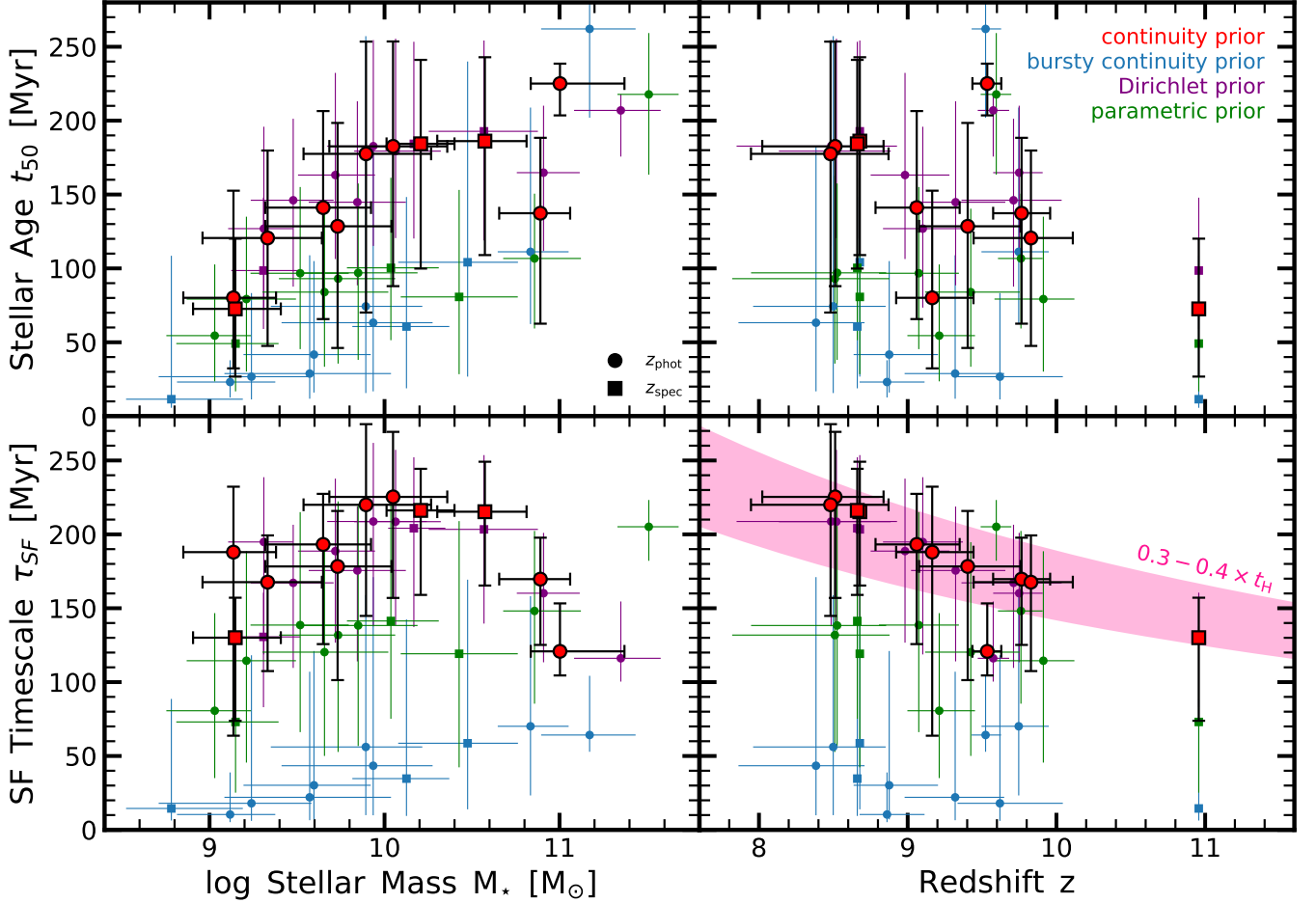
Figure 13. Stellar age t_{50} (top panels) and star-formation timescale \tau_{\text{SF}} (bottom panels) as a function of stellar mass M_* (left panels) and redshift z (right panels) of our z = 9 - 11 galaxies. The star-formation timescale \tau_{\text{SF}} is defined by time it took to increase the stellar mass from 20% to 80%, i.e., it is a measure of how quickly a galaxy formed its stellar mass. The pink shaded region in the bottom right panel indicates 30 – 40% of the age of the universe at a given redshift z . The red symbols show the fiducial continuity prior, while the smaller blue, purple and green symbols indicate the results for the bursty continuity prior, the Dirichlet prior, and the parametric prior. The squares mark the galaxies with spectroscopic redshifts, while the circles show the galaxies with photometric redshifts. The exact values of t_{50} and \tau_{\text{SF}} depend heavily on the assumed SFH prior: for the bursty continuity prior implies younger ages and shorter star-formation timescales, while for the fiducial continuity and Dirichlet prior \tau_{\text{SF}} older ages and longer \tau_{\text{SF}} . Independent of the SFH prior, we find older ages for more massive galaxies and longer star-formation timescales for the lower-redshift galaxies.
