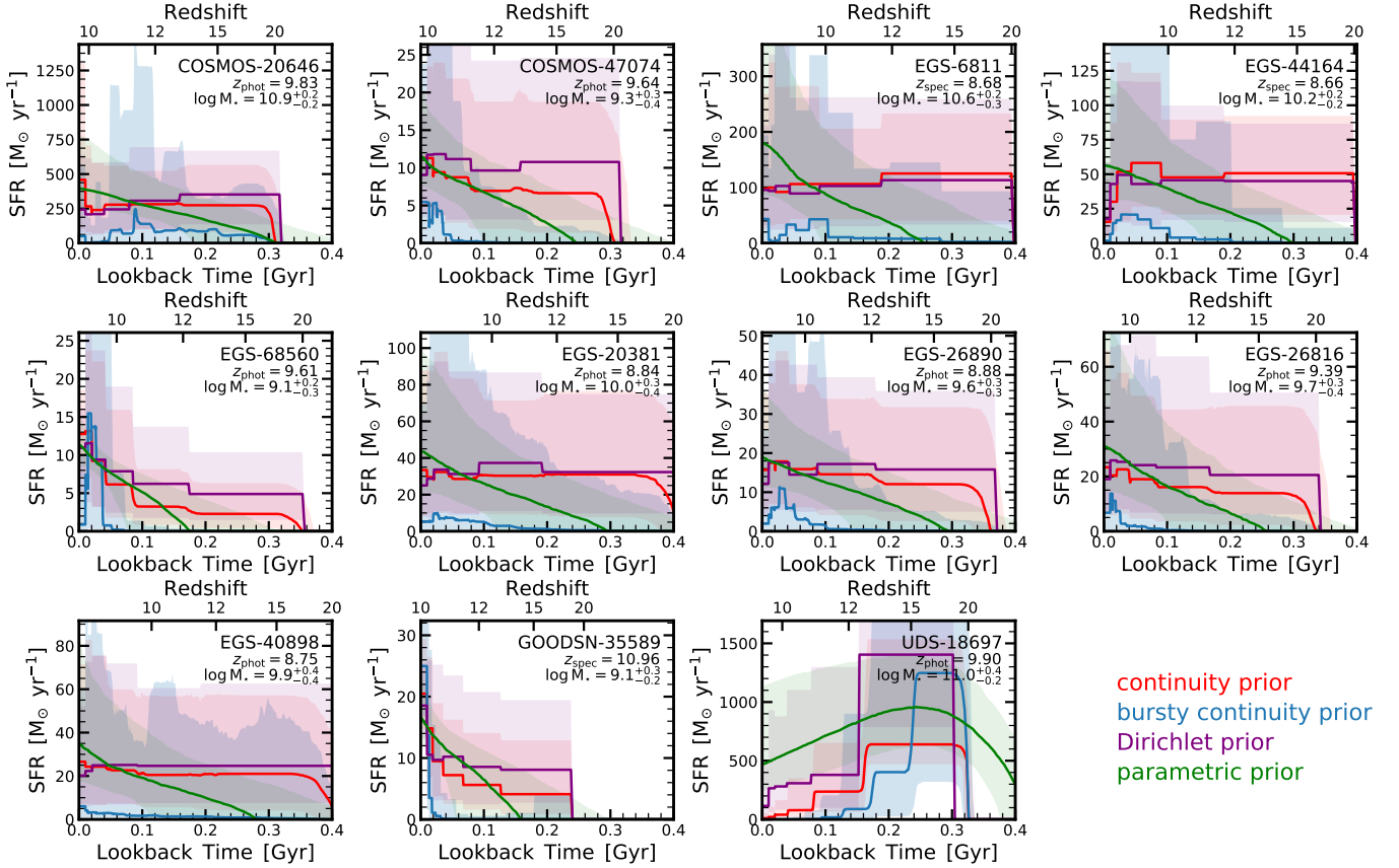
Figure 20. Star-formation histories (SFHs) obtained from Prospector assuming different priors. The adopted priors include the continuity prior (red), bursty continuity prior (blue), Dirichlet prior (purple) and parametric prior. These priors are discussed in Section 3.2. The lines and shaded regions show the median and 16–84th percentile of the SFH posterior, respectively. The continuity and Dirichlet prior typically lead to a rather constant SFH, the parametric prior (delayed-tau parametrization) to an increasing SFH, and the bursty continuity prior to a bursty SFH, which biases the median SFH low (see text). The key point of this figure is that the adopted prior heavily effects the resulting posterior SFH.
