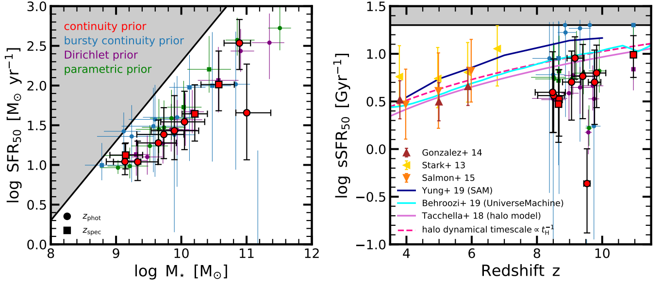
Figure 10. Star-formation rate (SFR) and stellar mass ( M_{*} ) properties of our z = 9 - 11 galaxies. The left and right panels show our galaxies in the \text{SFR}_{50} - M_{*} plane and the \text{sSFR}_{50} - z plane, respectively. The \text{SFR}_{50} and \text{sSFR}_{50} are averaged over the past 50 Myr. The red symbols show the fiducial continuity prior, while the smaller blue, purple and green symbols indicate the results for the bursty continuity prior, the Dirichlet prior, and the parametric prior. The squares mark the galaxies with spectroscopic redshifts, while the circles show the galaxies with photometric redshifts. The gray shaded regions indicate the forbidden parameter spaces, where \text{SFR}_{50} would be too high given the averaging timescale of 50 Myr and the stellar mass M_{*} (see Eqs. 2 and 3). In the right panel, we compare, at fixed stellar mass of \log(M_{*}/M_{\odot}) = 9 - 10 , our measurements to observations by González et al. (2014), Stark et al. (2013) and Salmon et al. (2015) and to the models of Yung et al. (2019b), Behroozi et al. (2019) and Tacchella et al. (2018a), where the two latter ones are both consistent with the evolution of the dynamical timescale of halos.
