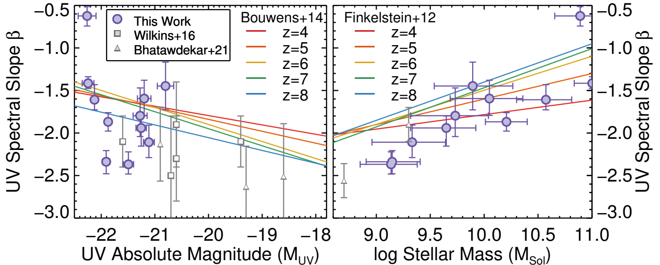
Figure 7. The measured UV spectral slope \beta for our sample of 11 z = 9 - 10 galaxies (Section 4.1.2), versus their derived UV absolute magnitude (left) and stellar mass (right). We show previously published results for predominantly fainter galaxies as small symbols. In the left panel the colored lines show the measured correlations between \beta and M_{UV} at z = 4 - 8 from Bouwens et al. (2014), while with similar lines in the right panel we show the measured correlations between \beta and the stellar mass at z = 4 - 8 from Finkelstein et al. (2012), converting from Salpeter to a Chabrier IMF. Our sample of z = 9 - 10 galaxies appears to exhibit a strong correlation with stellar mass (Pearson r = 0.85 ) and little-to-no correlation with M_{UV} (Pearson r = -0.32 ).
