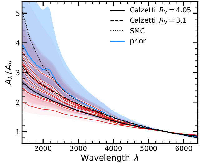
Figure 3. Our fitted attenuation law for all 11 galaxies in our sample in comparison with the Calzetti et al. (2000) attenuation curve and a SMC-like (Pei 1992) attenuation curve. The SMC curve is shown as dotted line, while the Calzetti et al. (2000) curve with R_V = 3.1 and R_V = 4.05 are plotted as dashed and solid lines, respectively. The blue solid line marks the median of the prior, while the associated shaded region indicates the 16-84th percentile of the prior. The individual solid lines and shaded regions in red show the median and 16-84th percentiles of our inferred posteriors. We find significant variations from galaxy to galaxy and the posteriors are rather broad.
