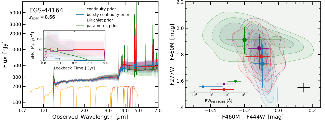
Figure 17. Distinguishability of different star-formation histories (SFHs). We plot in the left panel the posterior SED of EGS-44164 resulting from the four different SFH priors: continuity prior (red), bursty continuity prior (blue), Dirichlet prior (purple), and parametric prior (green). The inset show the posteriors of the SFHs. At bottom, the orange and red lines indicate widely used JWST /NIRCam wide (F090W, F115W, F150W, F200W, F277W, F356W, F444W) and medium (F335M, F410M, F430M, F460M) bands, respectively. By construction, the SEDs look very similar in the rest-frame UV, while there are some noticeable features around the Balmer break and in the emission line strengths. The right panel shows the JWST F277W–F460M versus F460M–F444W color-color diagram and the H\beta + [O\text{ III}] equivalent width ( EW_{H\beta+[O\text{ III}]} ) distribution. These medium-band colors are sensitive to emission lines since – for example in this case – the H\beta emission line straddles the F460M filter. The errorbars at the bottom right illustrate the 5\sigma uncertainty for \sim 15 msec exposures (see text for details).
