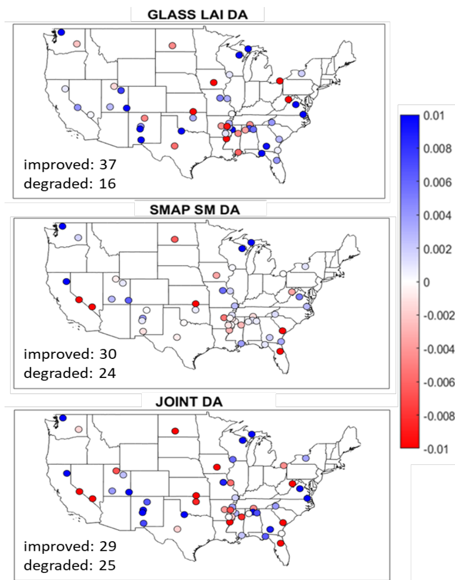
Figure 8: Difference in ACC between different DAs and OL with respect to ISMN for SSM over CONUS during 2016-2018. Blue (red) color indicates improvement (degradation) after the application of DA. The number of stations presenting an improvement/degradation thanks to DA are reported on each map.
