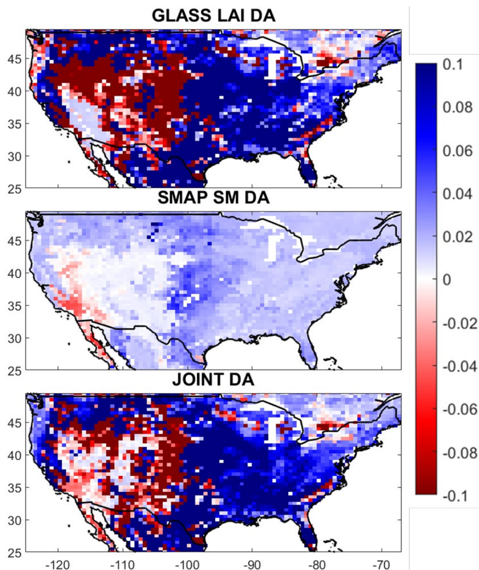
Figure 5: NIC of NCRMSE between DA and OL NEE with respect to FLUXCOM NEE during 2016-2018. Blue (red) color indicates improvement (degradation) after the application of DA.
