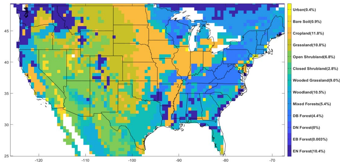
Figure 1: Land surface classification over the study region by MODIS in the Noah-MP model. The percentage area for each class is shown in the legend (EN: Evergreen Needleleaf; EB: Evergreen Broadleaf; DN=Deciduous Needleleaf; DB: Deciduous Broadleaf)
