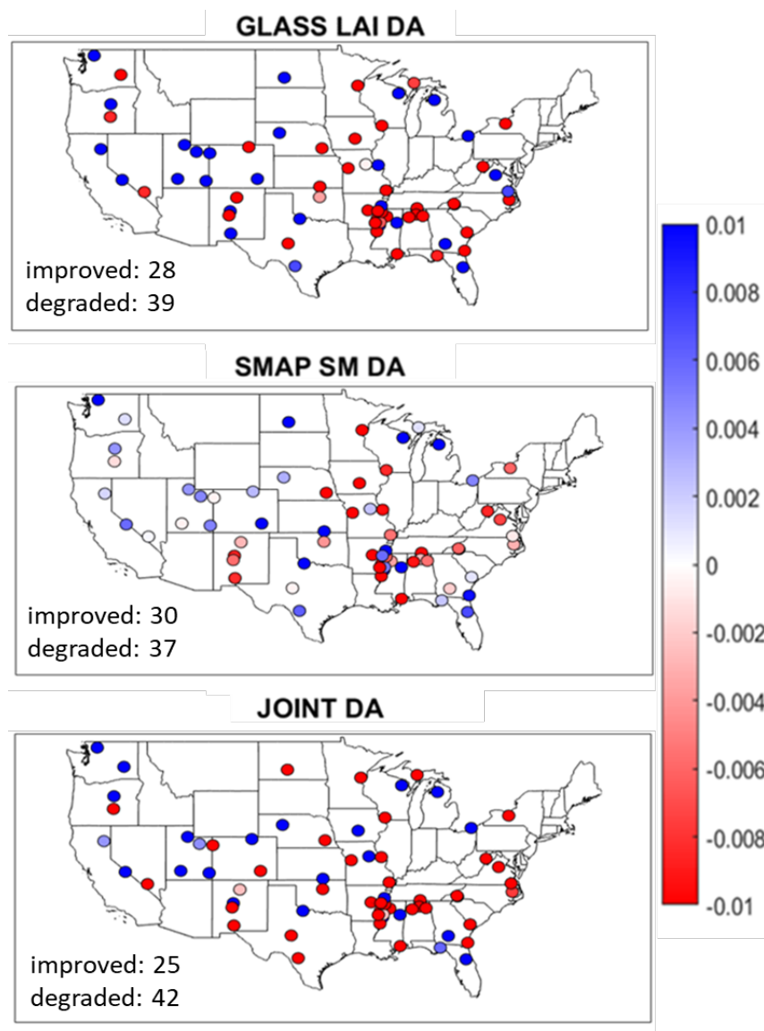
Figure 10: Same as Figure 8, but for RZSM.
