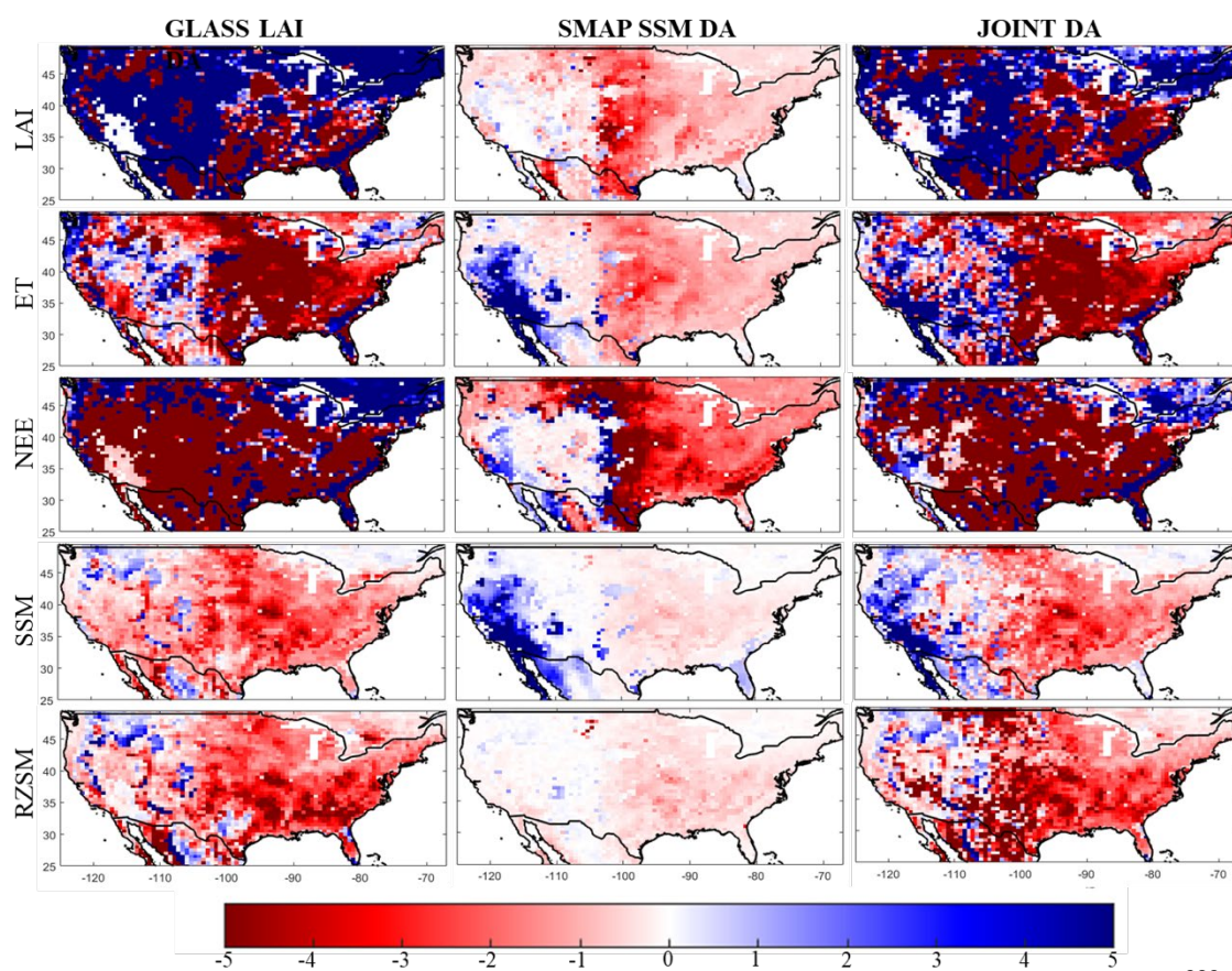
Figure 2. Percentage difference in the estimation of LAI, ET, NEE, SSM, and RZSM between DA and OL: GLASS LAI DA (left panels), SMAP SM DA (central panels), and joint DA (right panels). Red color shows a decrease in the variable estimation after the application of DA, whereas blue color shows an increase after DA.
