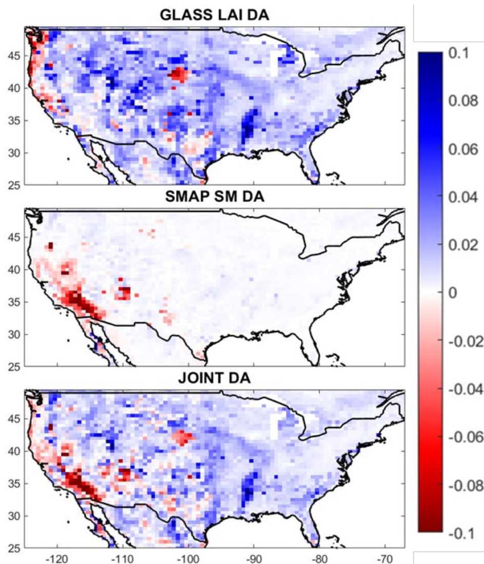
Figure 4: Difference of ACC between DA and OL ET with respect to GLEAM ET during 2016-2018. Blue (red) color indicates improvement (degradation) after DA.
