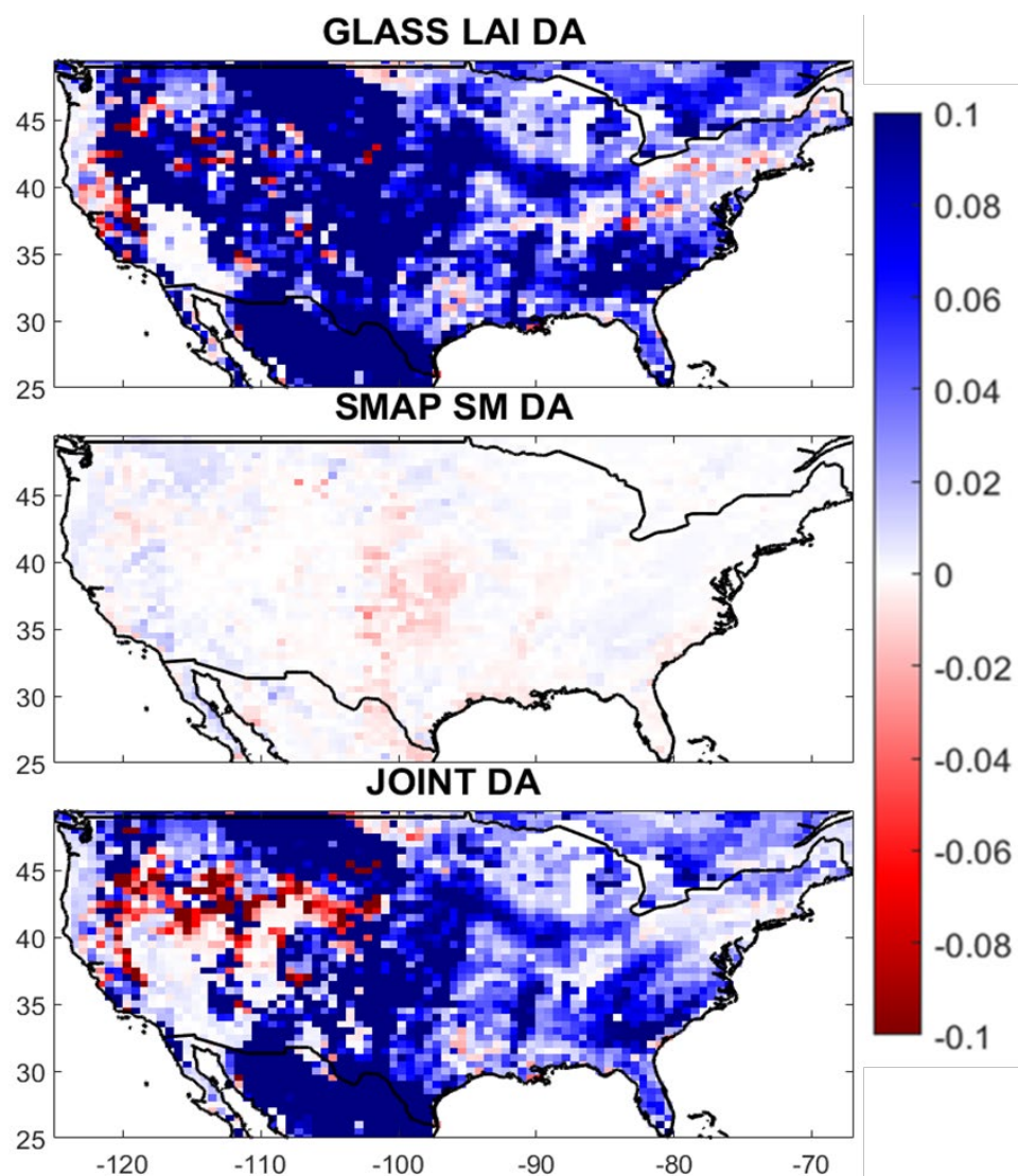
Figure 6: Difference in ACC between DA and OL NEE with respect to FLUXCOM NEE during 2016-2018. Blue (red) color indicates improvement (degradation) after the application of DA.
