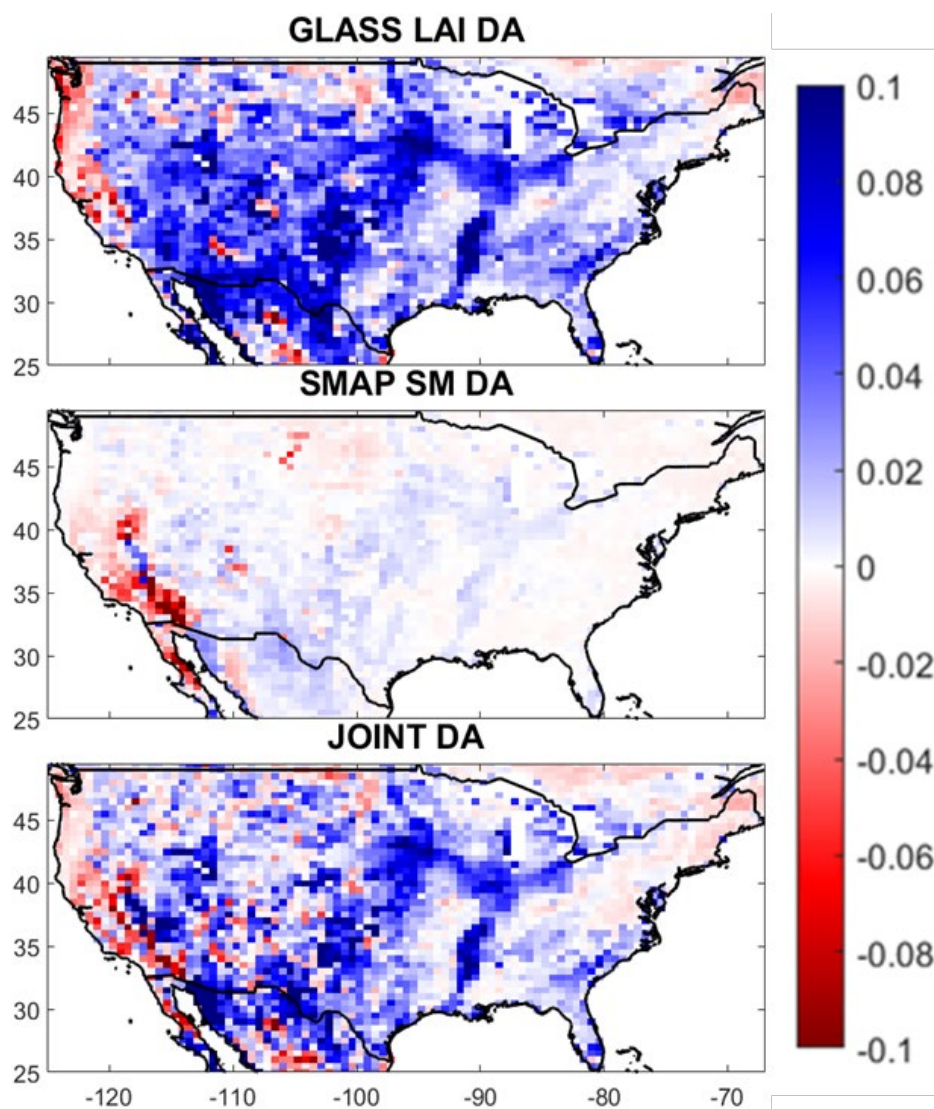
Figure 3: NIC of NCRMSE between DA and OL ET with respect to GLEAM ET during 2016-2018. Blue (red) color indicates improvement (degradation) after the application of DA.
