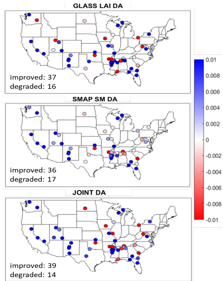
Figure 7: NIC of NCRMSE between different DAs and OL with respect to ISMN for SSM over CONUS during 2016-2018. Blue (red) color indicates improvement (degradation) after the application DA. The number of stations presenting an improvement/degradation thanks to DA are reported on each map.
