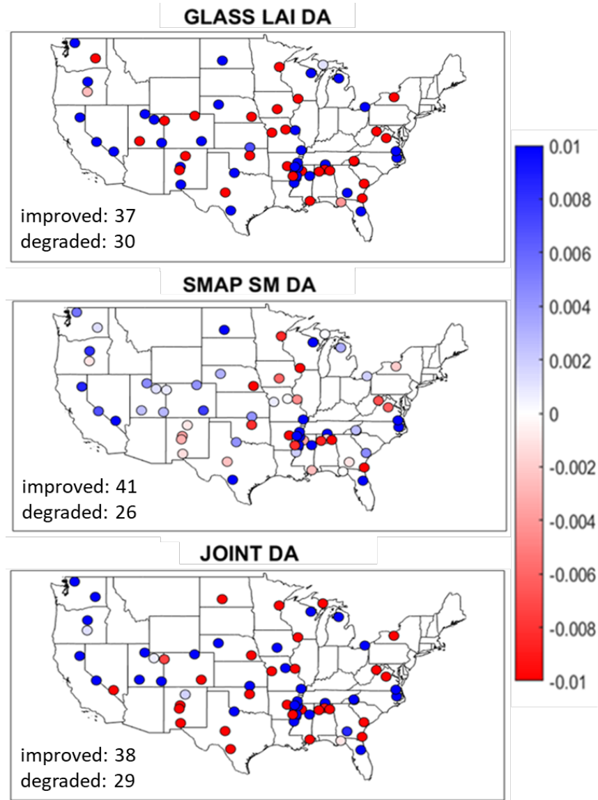
Figure 9: Same as Figure 7, but for RZSM.
