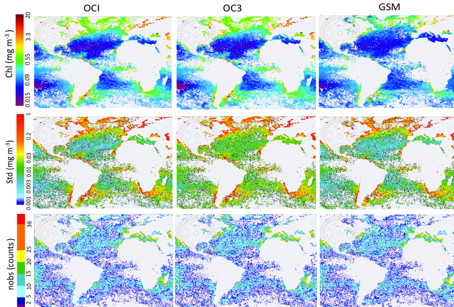
Fig. 4. Global image of SeaWiFS 14-day OCI-, OC3-, GSM-derived mean Chl , standard deviation, and number of observations ( nobs ). Satellite imagery analysis provides a means of assessing algorithm behavior and consistency in time and space. The satellite imagery can be used to evaluate algorithm spatial extent of valid retrievals, temporal (e.g., day-to-day or week-to-week) consistency in retrievals, and spatiotemporal distributions of error metrics from compiled satellite pixels. nobs can be used to compare the spatial coverage consistency of the algorithms. These analyses may also be informative where decision support activities prioritize consistent and broad satellite coverage.
