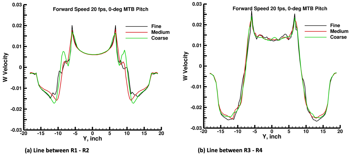
Figure 9. Spatial sensitivity analysis with various grids, 6-Rotor, Tunnel Speed = 20 fps, MTB Pitch = 0 deg. (a). W-velocity profile at a lateral location in at the front two rotors. (b). W-velocity profile at a lateral location in at the middle two rotors.
