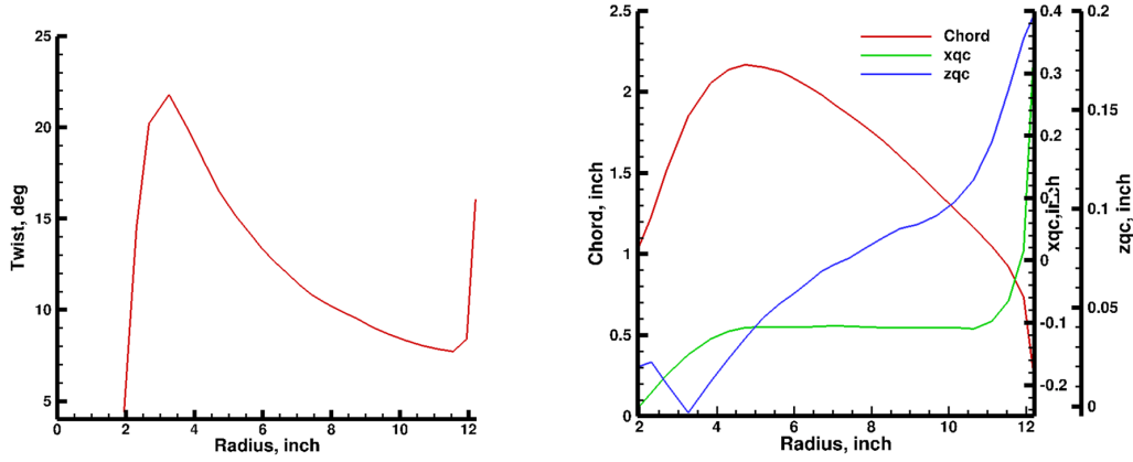
Figure 4. Geometric properties: Blade Twist, Chord, and Quarter-chord distribution
