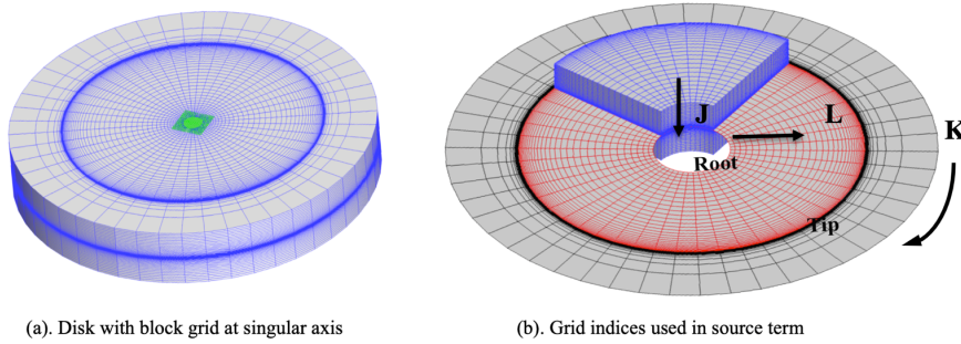
Figure 6. Grid used in the rotor disk model.
