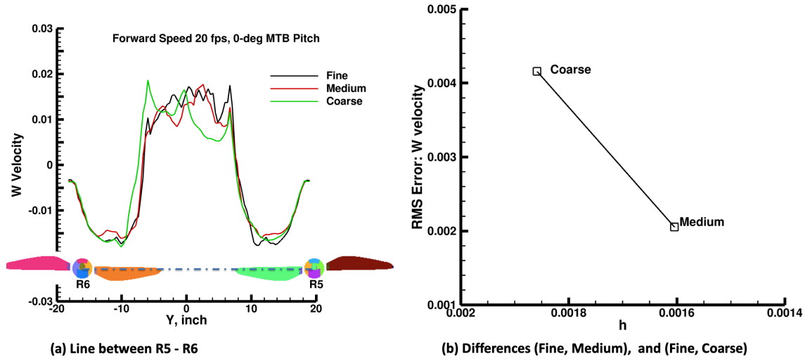
Figure 8. Spatial sensitivity analysis with various grids, 6-Rotor, Tunnel Speed = 20 fps, MTB Pitch = 0 deg. (a). W-velocity profile at a lateral location in at the aftmost rotors. (b). RMS difference between fine mesh and other two meshes.
