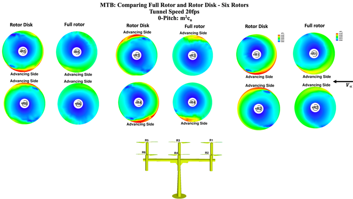
Figure 12. MTB: M^2 C_n on the disk plane. Comparing Full Rotor versus Rotor Disk Model solution for six rotors.
