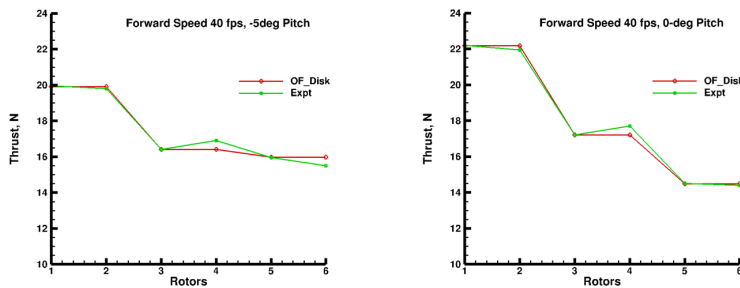
Figure 13. MTB 6 rotors: Comparing Rotor-Disk model trimmed solution to the experiment.
