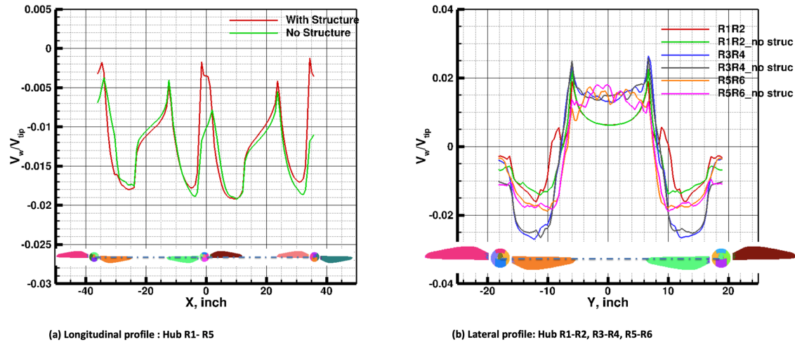
Figure 17. Velocity profiles showing the effect of support structures and body inside the tunnel. MTB 6-rotor, tunnel speed 5fps, 0-deg MTB pitch.
