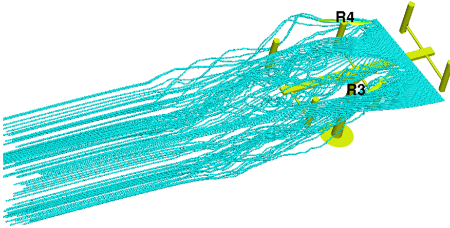
Figure 20. MTB 2 rotors: Comparing Rotor-Disk solution to the experiment. 20 fps, 0-deg MTB Pitch assembly.
