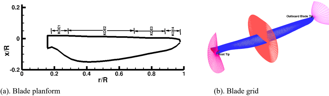
Figure 5. (a). Schematic of blade planform. (b). Blade grid
