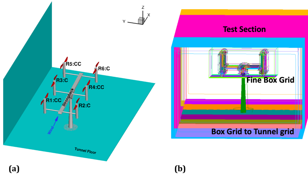
Figure 3. (a). Computational domain showing rotor numbering and configuration. C-clockwise, CC-counterclockwise rotor. (b). Right picture shows volume mesh that transitioned to the wall grid.
