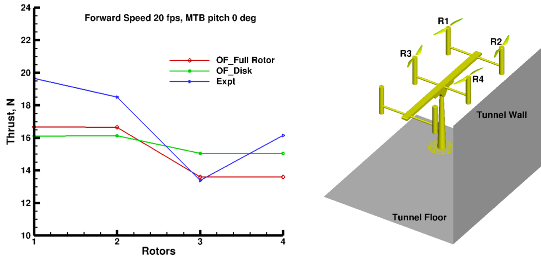
Figure 19. MTB 4 rotors: Comparing Rotor-Disk Solution to the experiment. 20 fps, 0-deg MTB Pitch assembly.
