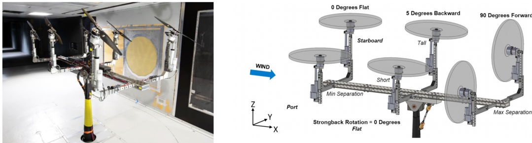
Figure 2. The left MTB in the U.S. Army’s 7-by 10-Foot Wind Tunnel at NASA Ames Research Center 1,2 . Picture on the right shows the tall and short configuration of the rotor support arms.
