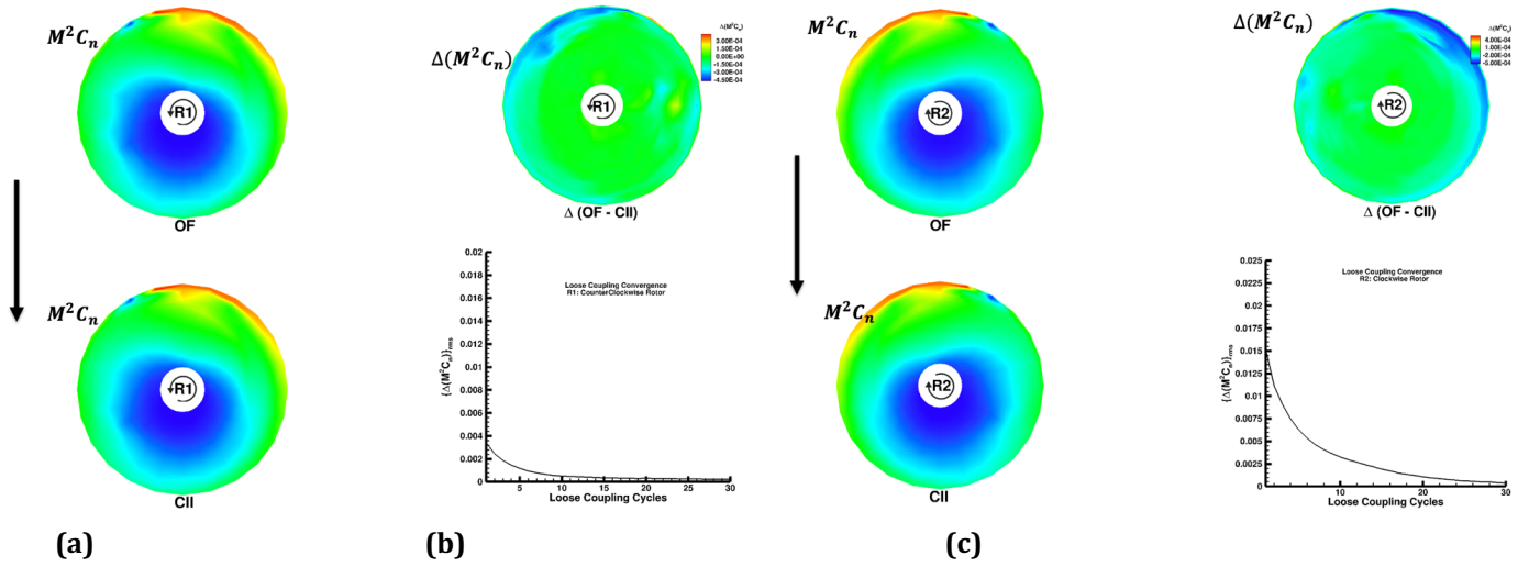
Figure 14. Loose Coupling (LC) Convergence for R1 and R2: \{\Delta(M^2 C_n)\}_{rms} \in (LC)\{OF \text{ and } CII \text{ on CAMRAD Data point}\} . Left two figures in (a) and (b) show the normal load at the CAMRAD collocated points. Right two figures show the delta load convergence between OVERFLOW and CAMRAD II.
