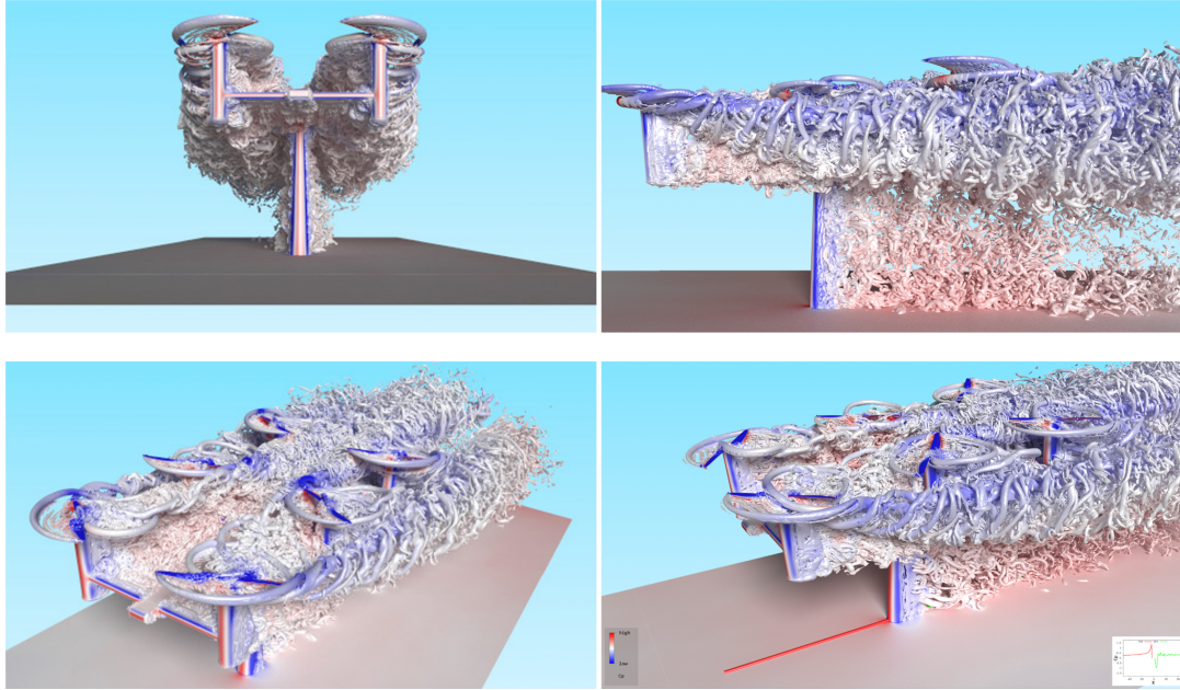
Figure 7. Vortices visualized with Q-criteria colored by pressure coefficient, C_p for MTB 6 rotors in Forward Flight, 40 fps, -5 deg pitch assembly. Looking at the flow with different perspectives.
