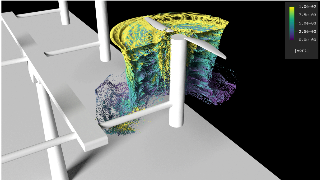
Figure 21. Isolated Rotor (Rotor 2) in Hover. Cut-away view of the vortex wake.
