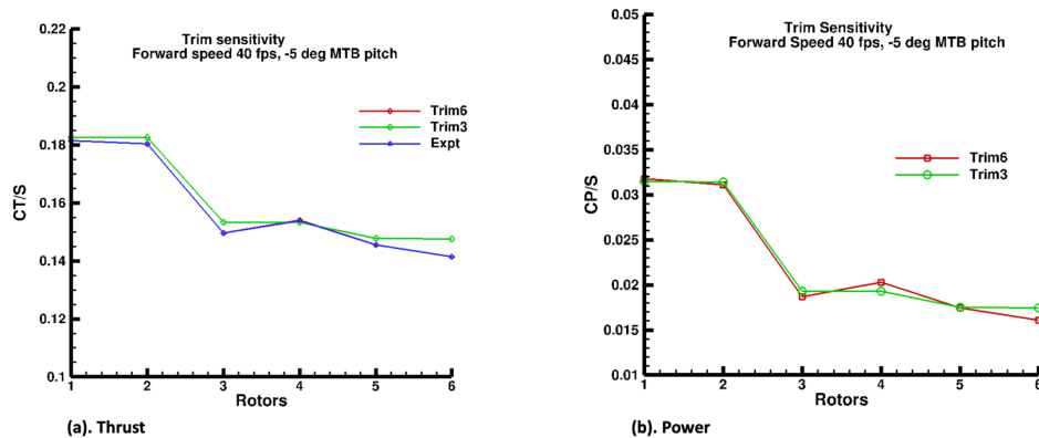
Figure 11. Trim sensitivity analysis with two methods, all 6-Rotors, and three longitudinal rotors on one side (right or Y- side), Tunnel Speed = 40 ft/s, MTB Pitch = -5 deg.
