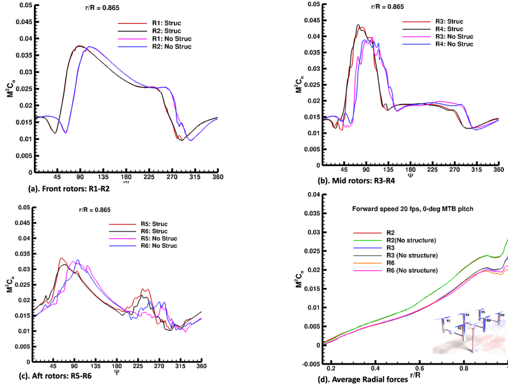
Figure 16. Sectional normal force coefficient showing the effect of support structures and body inside the tunnel.
