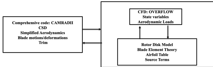
Figure 1. Schematic for CFD/CSD coupling for rotor disk model
