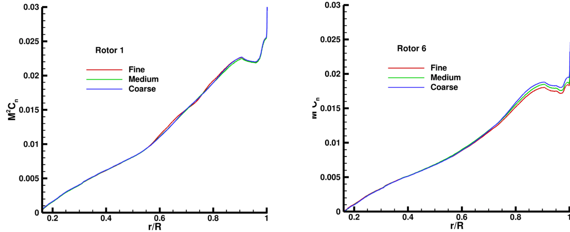
Figure 10. Spatial sensitivity analysis with various grids, 6-Rotor, Tunnel Speed = 20 fps, MTB Pitch = 0 deg. Sectional loads (a). at a representative front rotor, (b). at an aftmost rotor.
