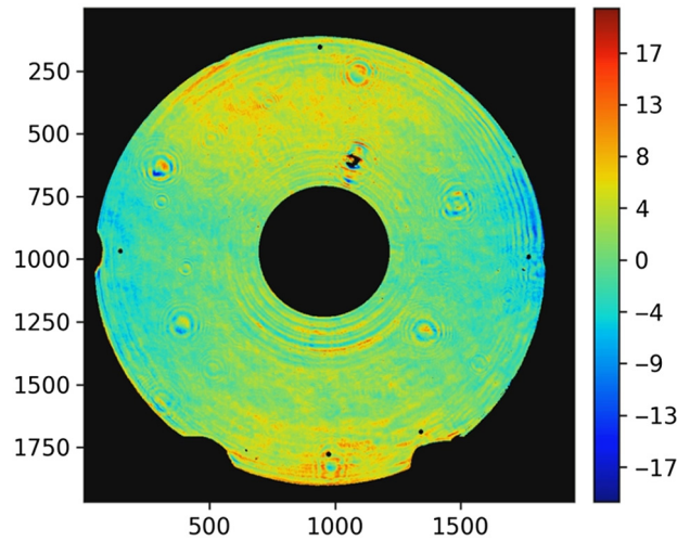
Fig. 43 Video 2 showing imposed coma surface figure shape (Video 2, MOV, 4.6 MB https://doi.org/10.1117/1.JATIS.8.2.024001.2 ).
