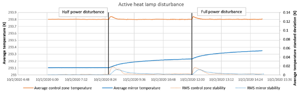
Fig. 37 Mirror response to thermal change with active control.
