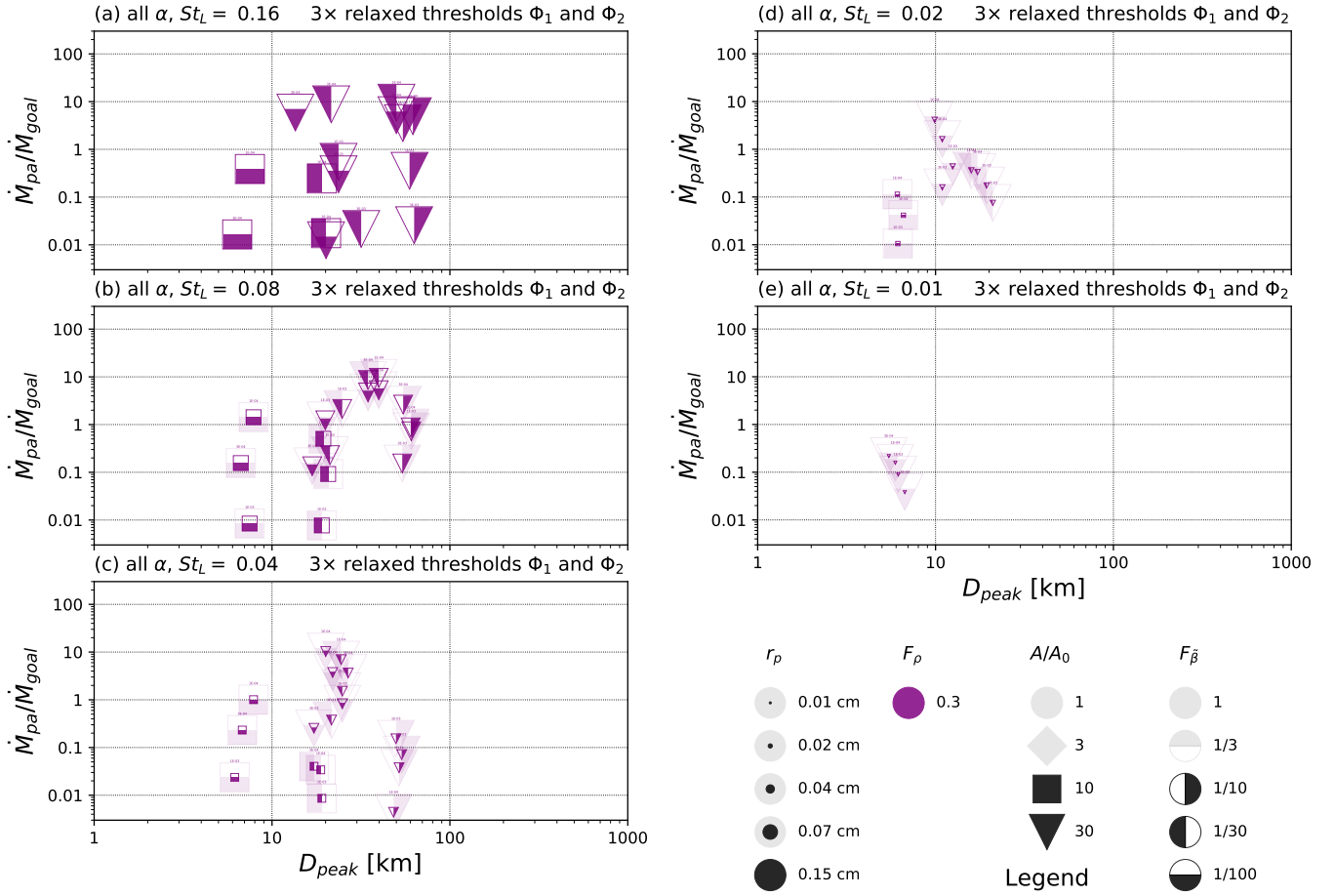
Figure 8. Outer nebula results for a gas density lower than the MMSN ( F_p = 0.3 ), for an extended range of solids-to-gas ratios ( A/A_o \in [1, 30] ) and relaxed thresholds. Each panel shows results for different Stokes numbers, and where St_L = 0.01 is the smallest Stokes number that produced planetesimals in the plot range. As before, symbol shapes and fill styles denote factors for solids enhancement and pressure gradient parameter, respectively, and the value of \alpha for each case is printed above each datapoint in small font best seen under magnification. The symbol size again scales with the particle size as indicated in the legend, but note that the size range is very different from the other outer nebula figures (Figures 6 and 7).
