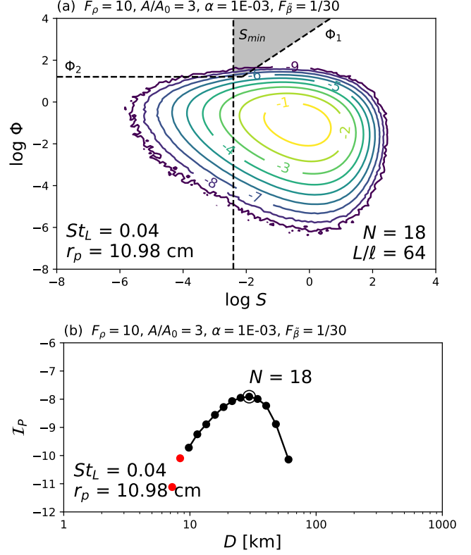
Figure 2. (a) Contours of joint PDF P(\Phi, S, \ell) for mass loading factor \Phi and normalized enstrophy S for Stokes number St_L = 0.04 at cascade level N = 18 and nebula gas parameters as indicated above the plot (see Table 1 for a description of the symbols). The thresholds \Phi_1 , \Phi_2 and S_{min} (Section 2.3.3) are shown by dashed lines. The planetesimal-forming region of the parameter space is shaded in gray. (b) The Initial Mass Function (IMF) for this case, computed by integrating the probabilities above the thresholds – each dot is the result at a single value of N . The peak in this particular case (marked with a circle) is reached at cascade level N = 18 , and corresponds to a planetesimal diameter of 29.5 km. Black symbols indicate that \Phi is below the mass loading limit while red symbols show where the results are questionable because the mass loading limit of \Phi_{limit} = 100 has been surpassed.
