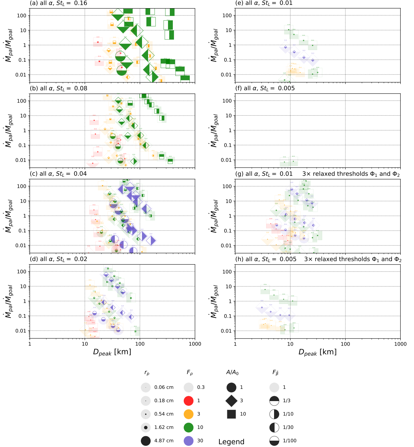
Figure 7. Model results for the outer nebula where similar to Figure 5 Stokes numbers are plotted in separate panels for nominal thresholds (panels (a)–(f)) and relaxed thresholds (panels (g), (h)). Again, colors, symbol shapes and fill styles denote factors for gas density enhancement, solids enhancement and pressure gradient parameter, respectively. The value of \alpha for each case is printed above each datapoint in small font best seen under magnification. Particle sizes above 5 cm have been omitted for legibility. The smallest planetesimal-producing Stokes number is St_L = 0.005 , both for nominal and relaxed thresholds.
