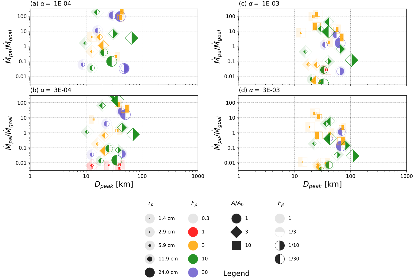
Figure 3. Model results for the inner nebula, showing the peak of the planetesimal IMF, D_{peak} , and the rate of formation, \dot{M}_{pa} , relative to the expected rate, \dot{M}_{goal} , for a wide range of nebula parameters and particle sizes. Thresholds use their nominal, non-“relaxed” values. The panels show results for different values of \alpha , while (within each panel) colors, symbol shapes and fill styles denote gas density enhancement factor, F_\rho , solids enhancement factor, A/A_0 , and the scale factor for the headwind parameter, F_{\beta} . The size of the symbols scales with the particle radius r_p . The smallest and largest particle sizes that resulted in planetesimals are shown in the legend, together with some representative values in between. The legend symbols for F_\rho , A/A_0 and F_{\beta} show all parameter values that were computed and included in the figure if they produced planetesimals in the range. Those parameters that did not produce results in the plot range have been greyed out.
