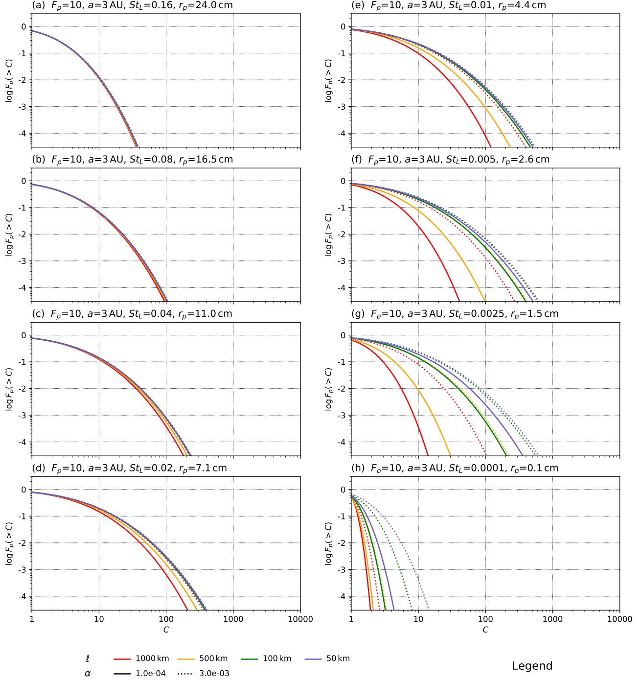
Figure 10. Cumulative fraction F_p(>C) of particles lying in a region where the concentration is larger than some value C . In this context, concentration refers to the ratio of the local density (averaged on some length scale \ell ) to its global average, and does not account for any other enhancement effects such as settling towards the midplane, or various kinds of radial enhancement. Results from our cascade model are shown for different Stokes numbers (panels (a)–(h)) with Stokes number and corresponding particle sizes noted above each panel, for a range of length scales \ell within each panel, and two different values of \alpha . All results are for a F_p = 10 nebula gas at 3 AU.
