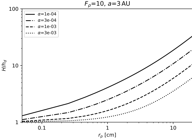
Figure 11. Ratio between gas density scale height H and solids density scale height h_d as functions of particle radius r_p . Particles settle towards the midplane depending on their Stokes number and the turbulent intensity \alpha , leading to a scale height that is smaller than that of the gas (Equation 9). The values shown are for a nebula with a gas density 10\times that of a MMSN, at a distance of 3 AU.
