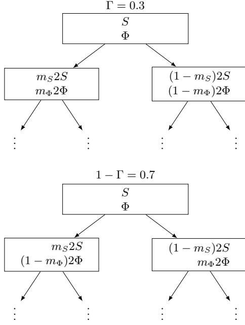
Figure 1. Diagram depicting the partition of normalized enstrophy S and mass loading factor \Phi from one cascade level to the next. The multipliers m_S and m_\Phi are assumed to be greater than or equal to 0.5. With a probability of \Gamma = 0.3 , the subvolume with the larger fraction of S also has a larger fraction of \Phi (upper figure), while the reverse is true with a probability of 1 - \Gamma = 0.7 (lower figure).
