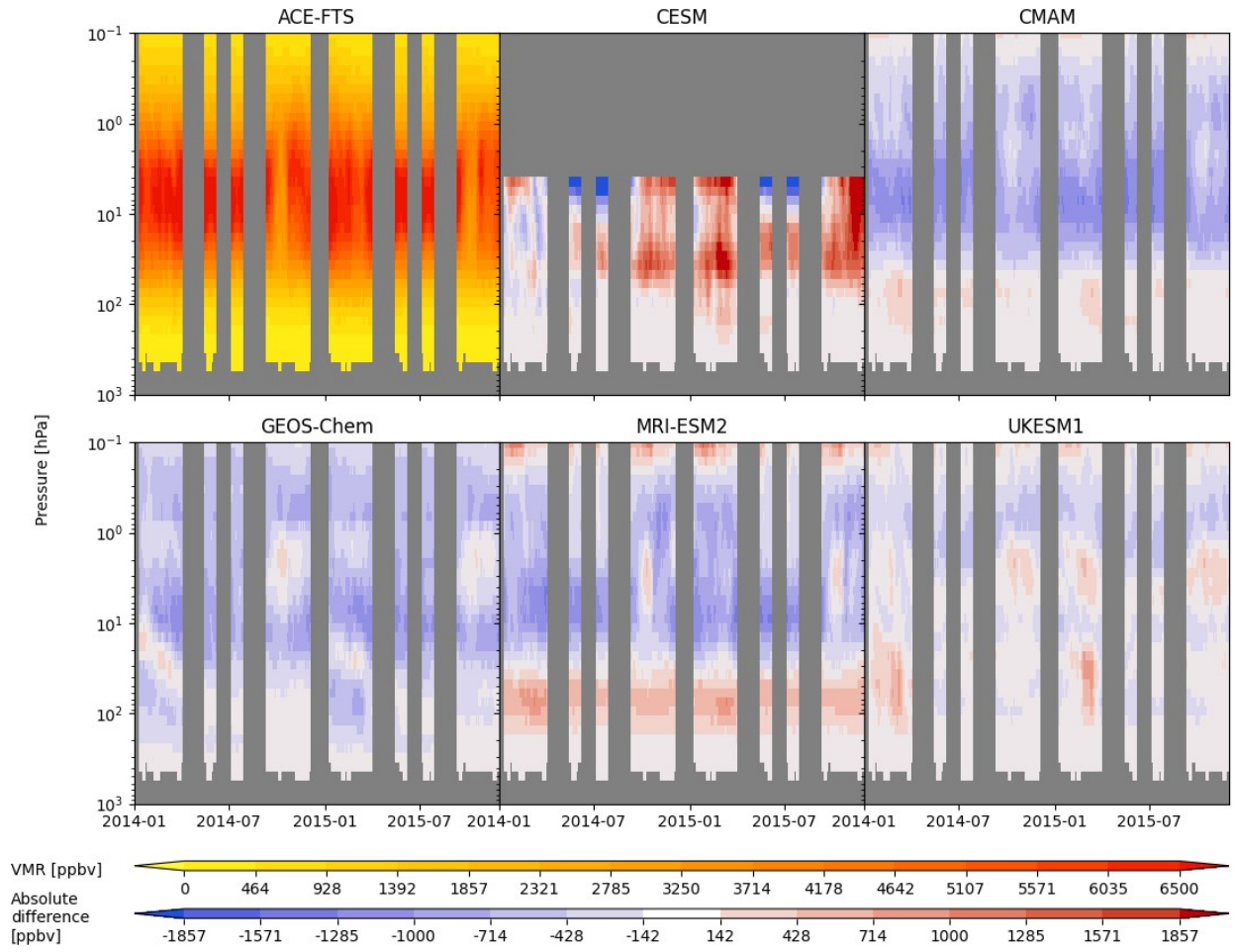
Fig S3. (top left) ACE-FTS measurements of Arctic (>60°N) O 3 vs month (in ppbv, top colour bar) and (rest of panels) model biases for 2014-15 (model minus measurement, also in ppbv, lower colour bar). Results for 2008-9 are similar and not shown.
