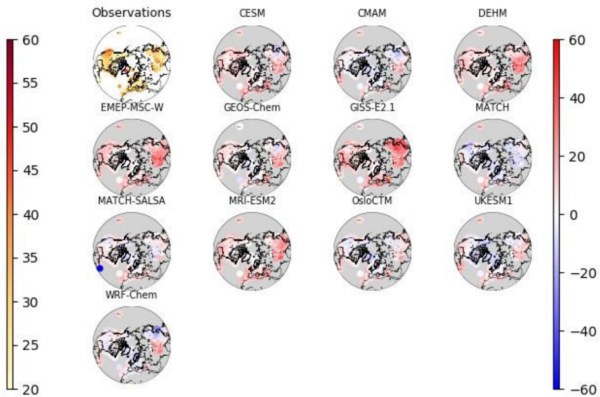
Fig S2. Annual mean O 3 volume mixing ratios (ppbv, left colour bar) at surface measurement sites, and model bias (model minus measurement in ppbv, right colour bar) for 2014-15. Results from 2008-9 are similar and not shown.
