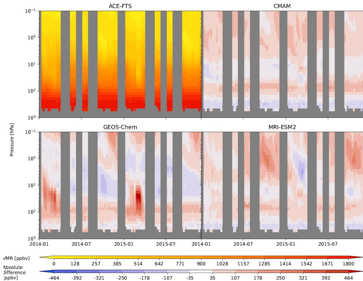
Fig S1. (top left) ACE-FTS measurements of Arctic CH 4 vs month (in ppbv, top colour bar) and (rest of panels) model biases for 2014-15 (model minus measurement, also in ppbv, lower colour bar). Results for 2008-9 are similar and not shown.
