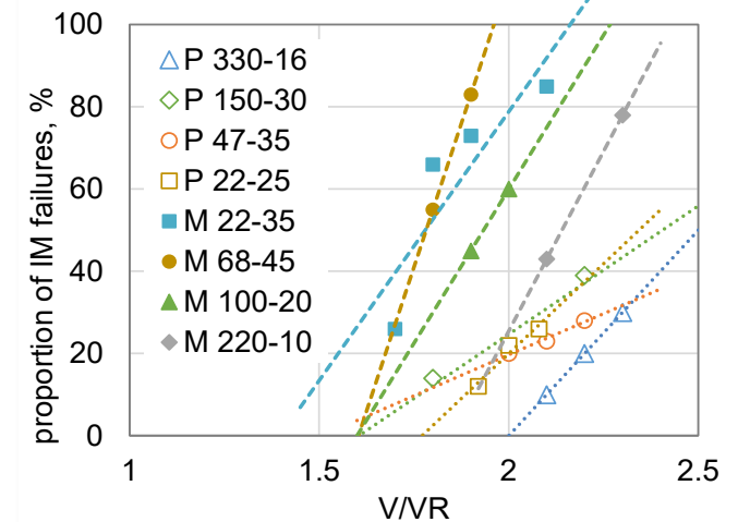
IM failures during HALT
