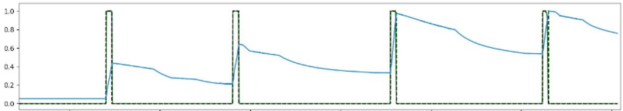
Fig. 7 Calorimeter time-series segmentation: plot showing segmentation of calorimeter insertions.
