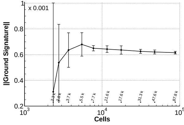
(a) Ground signature, Eq. 31
