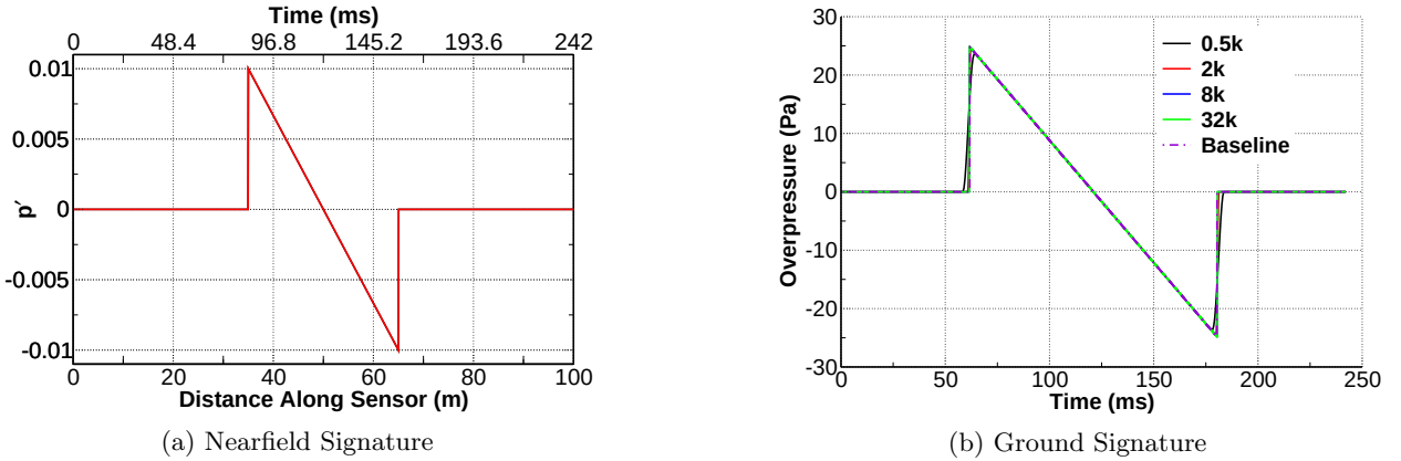
Figure 3: Initial N-wave (left) and convergence of ground signature with uniform refinement (right).
