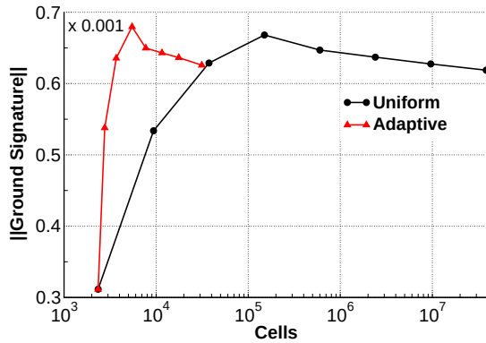
(a) Ground signature, Eq. 31
