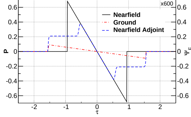
Figure 4: Nearfield and ground N-waves, and the nearfield adjoint for the ground-signature output. The adjoint solution is scaled by a factor of 600 to allow comparison with features of the waveforms.
