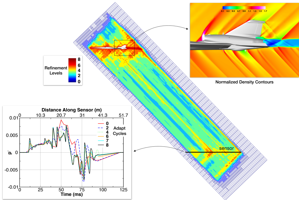
Figure 21: Nearfield details for the X-59 configuration. Lower-left frame shows evolution of the pressure signature driven by the C-SEL output. Middle frame shows the final mesh with cells colored by refinement level (dark reds represent smallest cells). Top-right is a close-up of the aft region of the aircraft, showing high resolution of the shock-plume interactions that propagate to the sensor.
