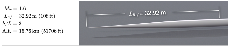
Figure 13: Geometry and conditions for the Axie test case
