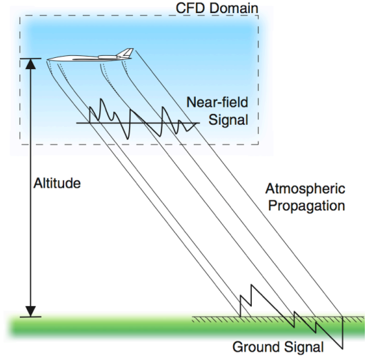
Figure 1: Sonic-boom domain decomposition
