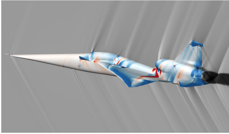
Figure 19: X-59 aircraft model and near-body flow ( M_\infty = 1.4 and \alpha = 2.09^\circ ). Aircraft surface is colored by C_p (red denotes pressures above freestream, blue below). Gray scale is used to visualize the near-body shocks via density variations on a plane through the aircraft's centerline.
