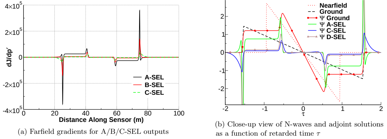
Figure 7: Characteristics of gradients and adjoint solutions, \Psi , for the ground signature and selected metrics.
