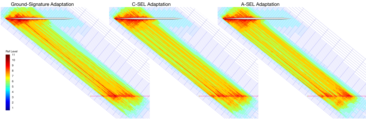
Figure 16: Final meshes colored by refinement level for simulations driven by farfield outputs: ground signature, C-SEL and A-SEL. Meshes have 76.2 M, 75.9 M, and 76.1 M cells, respectively.
