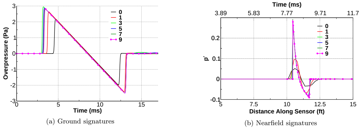
Figure 8: Convergence of ground and nearfield signatures as a function of refinement in the nearfield domain for the ground signature output of the NACA 0003 test case. Every other adaptation cycle is plotted.
