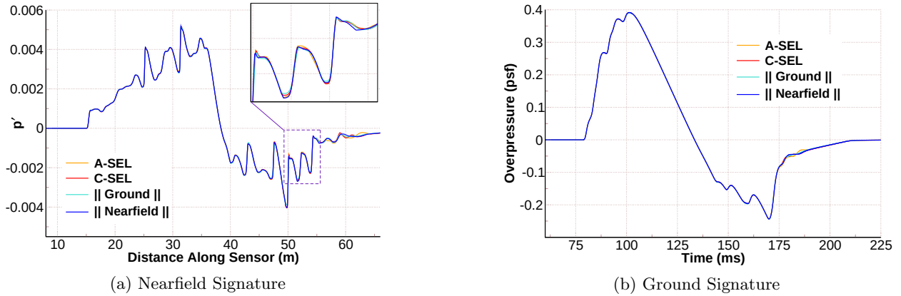
Figure 14: Signatures obtained with J_A (A-SEL), J_C (C-SEL), J_G (Ground) and J_N (Nearfield) outputs.
