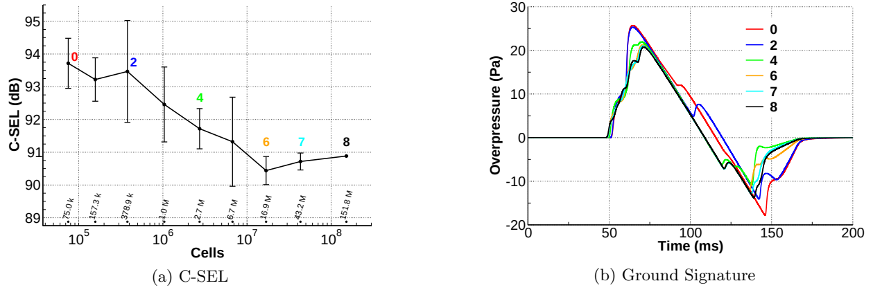
Figure 20: Convergence of C-SEL and ground signature for the X-59 geometry
