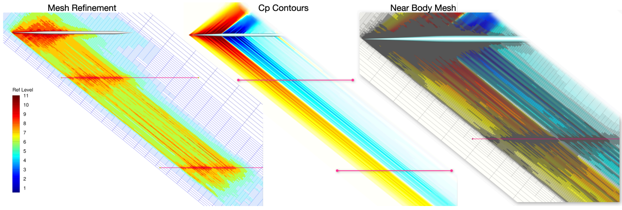
Figure 15: Final mesh containing 75.5 M cells and C_p distribution (red indicates high pressure and blue indicates low pressure) for the Axie body with adaptation driven by nearfield line sensors.
