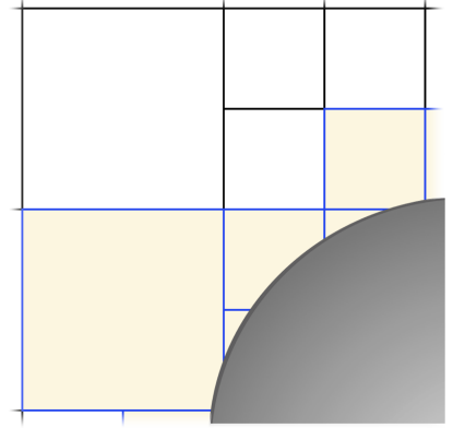
Figure 2: Multilevel Cartesian mesh with a cut-cell boundary (highlighted)
