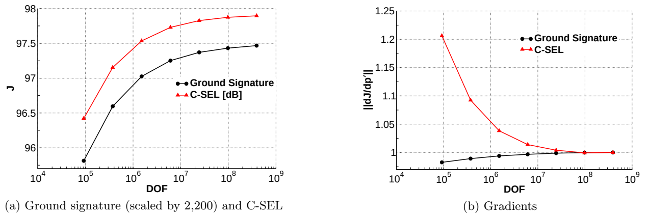
Figure 6: Convergence of output functionals (left) and normalized gradient norms (right) with uniform refinement from 501 to 32,001 nodes and constant CFL.
