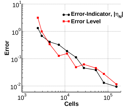
Figure 9: Convergence of farfield outputs as a function of adaptive refinement of the nearfield mesh. Error bars in plots on left indicate level of discretization error shown as red lines in plots on right.
