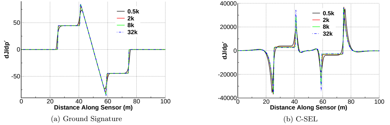
Figure 5: Convergence of \Psi_F (also \partial J/\partial p' ) along the nearfield sensor with uniform refinement from 501 to 32,001 nodes and constant CFL.
