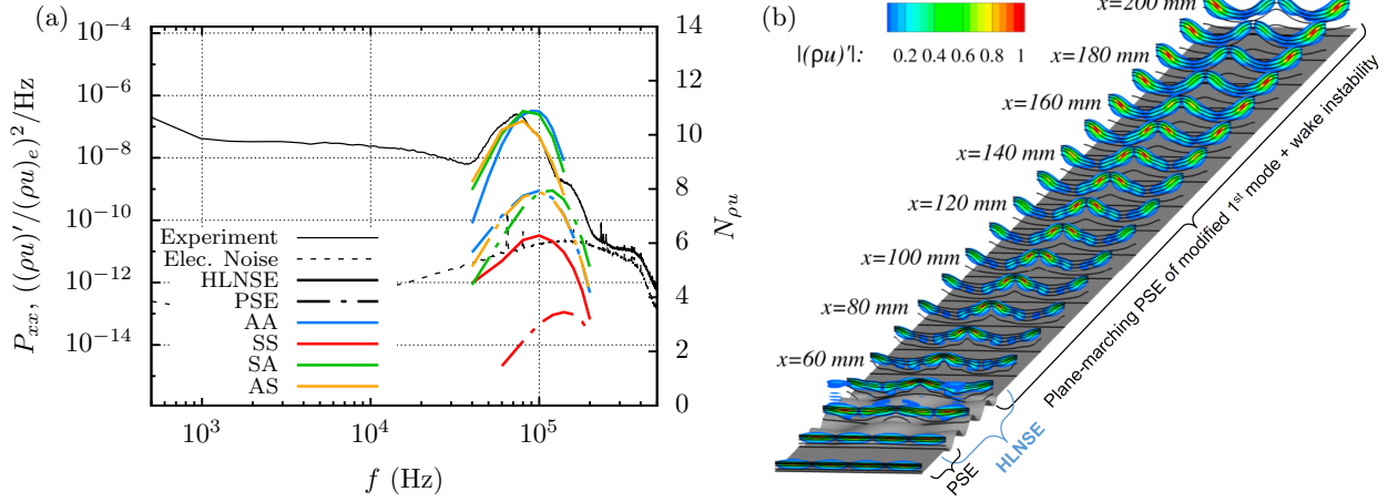
Figure 1: (a) Comparison of power spectra to most-amplified disturbances at x = 153.8 mm distance from the leading edge. The HLNSE results refer to the disturbance evolution calculated with a combination of plane-marching PSE and HLNSE, while the PSE results refer to the plane-marching PSE analysis of the roughness wake disturbances. (b) Disturbance streamwise mass flux contours and basic state isolines of AA disturbance with 80 kHz over the flat plate with a roughness patch. Adapted from Ref. [20].
