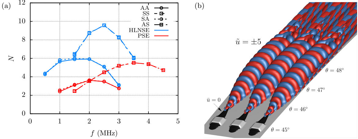
Figure 2: (a) Comparison of N-factor spectra of fundamental and subharmonic, symmetric and antisymmetric disturbances at \theta = 48^\circ from the axis. The HLNSE label refers to inflow-resolvent HLNSE results and the PSE label refers to the plane-marching PSE analysis of the roughness wake disturbances. Adapted from Ref. [32].
