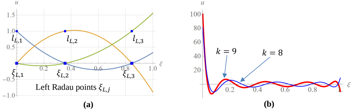
Fig. 2.2 (a) The left Radau points \xi_{L,j} (blue square dots) and the corresponding Lagrange polynomials l_{L,j} , j = 1, 2, 3 for k = 2 . (b) The approximate Dirac delta function \gamma = (k + 1)^2 l_{L,1} for k = 8 (blue thin curve) and k = 9 (red thick curve).
