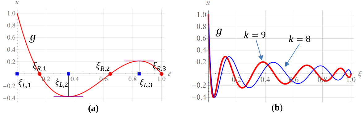
Fig. 2.3 (a) The cubic correction function g for the case k = 2 ; g vanishes at the three right Radau points (red circular dots) and has local extrema at two of the three left Radau points (blue square dots). (b) The correction functions of degree k + 1 for k = 9 (thick red curve) and k = 8 (thin blue curve).
