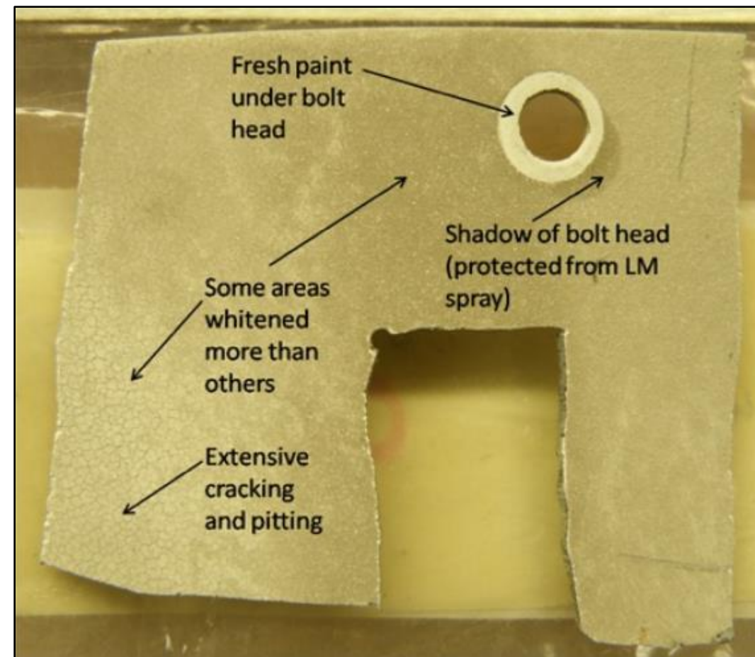
Impact damage to the Surveyor 3 coupon returned by Apollo 12 due to PSI ejecta from the LM descent engine. More concentrated ejecta produce more significant damage. Credit: UCF/NASA.
