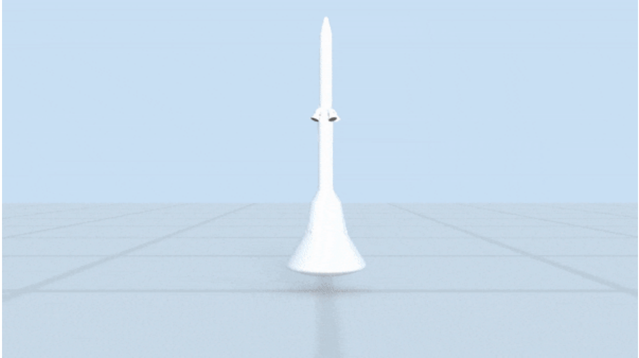
Figure 14: Animation of the accelerating PA-1 simulation showing passive particles seeded at the nozzle and convected with the volumetric data generated. Particles are colored by velocity magnitude where white is high and dark orange is low velocity. The vehicle is shown in white, and the ground is shown as a light gray grid to clarify the perspective and relative motion of the vehicle. Credit: Timothy Sandstrom
