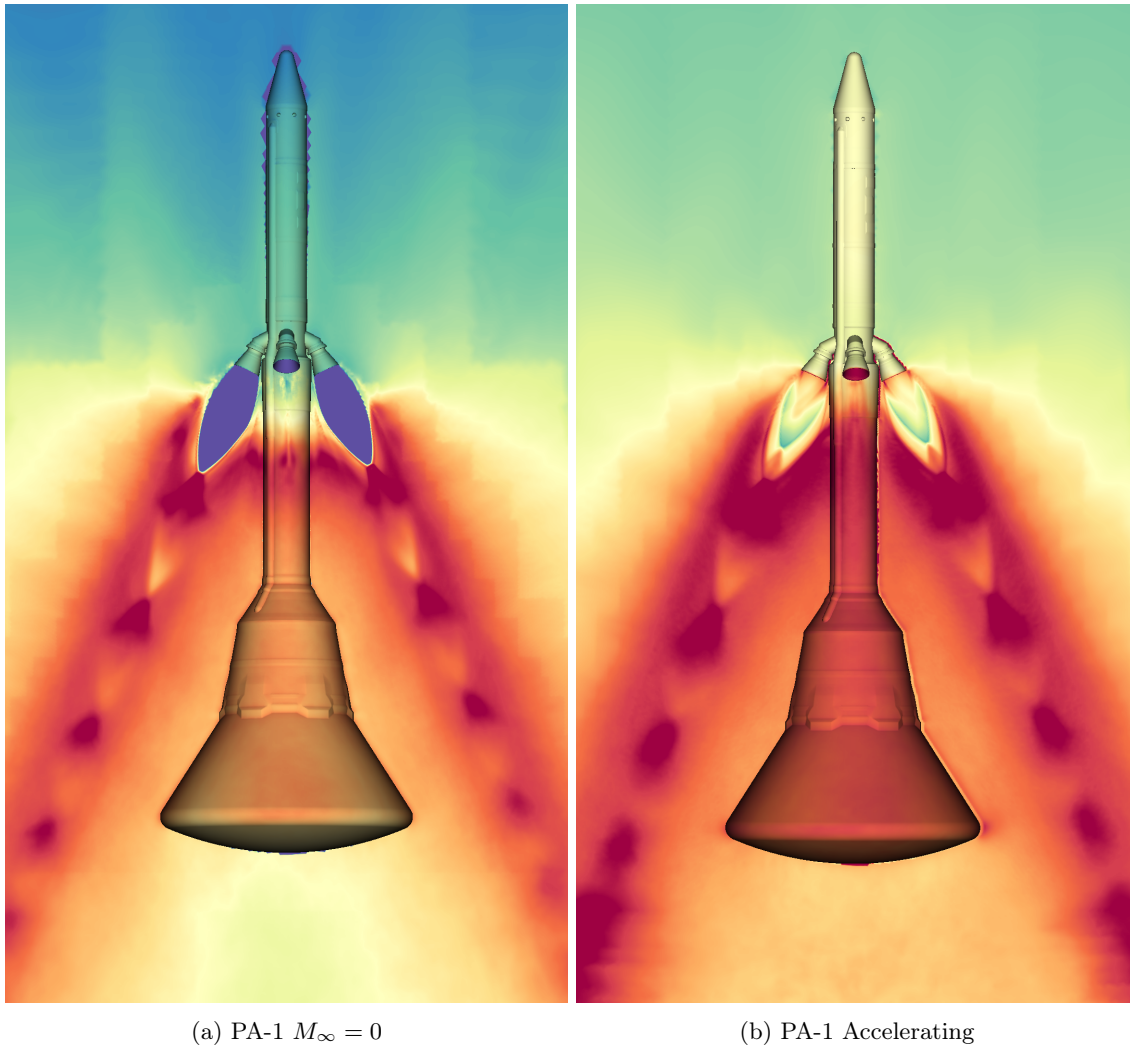
Figure 16: Post-processed CFD results for the static and accelerating PA-1 case showing overall sound pressure level (OASPL) on vehicle surface and cut plane through nozzles; blue is low and red is high.
