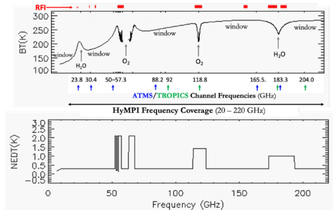
Figure 2. Top: An illustrative example of a HyMPI spectral coverage (black curve). Bottom part illustrates HyMPI's noise characteristics. To ensure continuity to the Program Of Record (POR), HyMPI includes all ATMS (blue arrows) and TROPICS channels (green arrows) at their native spectral resolution, a feature made possible by the PICASIC's unique modular design. This technology also enables to increase spectral resolution up to 500 KHz to detect and remove Radio Frequency Interference (RFI), whose spectral allocations are indicated by the red bars in the top figure.
