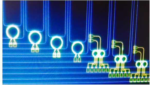
Figure 1. Photonic Integrated Circuits are like electronic circuits, but in this case the signal carrier is optical (photons). Optical waveguides (blue lines) carry the propagation of the optical signal. Metal conductors (yellow lines) are used to induce electro-optic effects on the waveguides to tune the filter response. Photonic integrated technology carries the unique advantage of reducing instrument size, weight and power and cost (SWaP-C). Photonic integrated technology also offers high compatibility with existing electronic technology.
