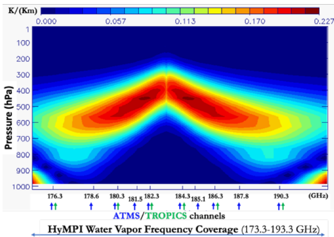
Figure 3. HyMPI’s brightness temperature sensitivity to variations of temperature (top) and water vapor (bottom). 1K temperature (5% water vapor) perturbations in each 1 km-pressure layer of the atmospheric profile have been applied to measure the response in brightness temperature at each frequency of HyMPI’s oxygen (water vapor) bands. For comparison purposes, ATMS and TROPICS spectral channel frequencies are highlighted by blue and green arrows, respectively.
