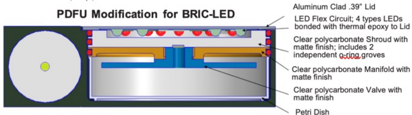
Canister Assembly.
