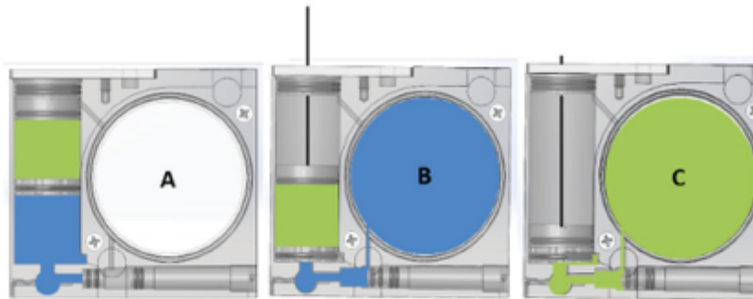
Fig. 2. Injection of Fluids into PDFU Pertri Dishes. A. Liquids 1 & 2 contained within the PDFU reservoir prior to actuation. B. Actuator piston partially depressed to deliver Liquid 1. C. Completion of actuation allows Liquid 2 to be delivered.
