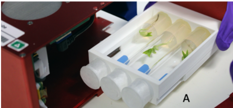
(A) 2U CubeLab growth chamber installation. (B) Malting CubeLab investigation with fluid and thermal control subsystems. (C) On-Orbit plant growth image.
