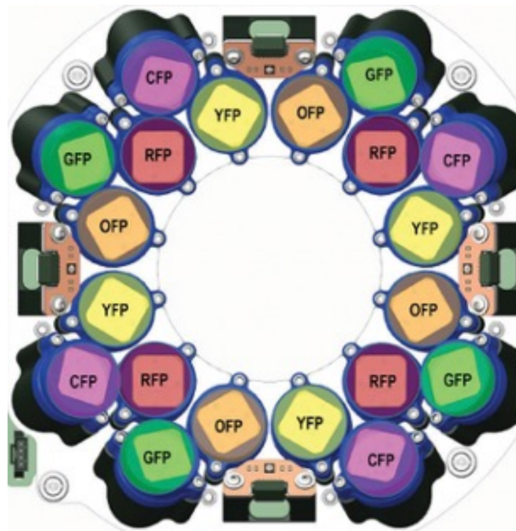
ELS and Carousel Subsystems within the Spectrum Growth Chamber. Insets are images of Arabidopsis plants expressing GFP and RFP fluorescence.
