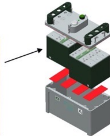
Canister Assembly.
