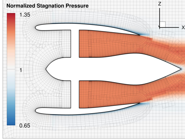
Figure 5: The CFD model uses subsonic outflow BCs for the fan face and subsonic inflow BCs for the fan exit. The mass, momentum, and energy conservation across the fan are satisfied by adjusting the BC values on the fan face and exit.
