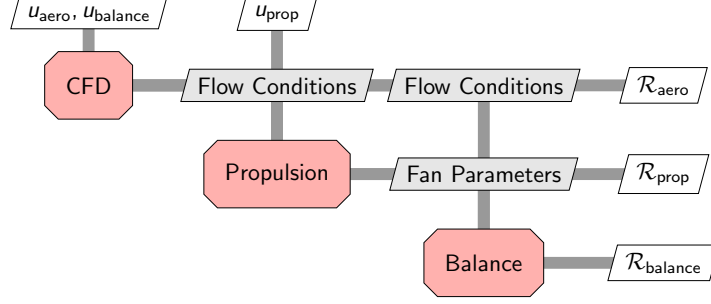
Figure 4: XDSM diagram of the podded fan aeropropulsive model [13].
