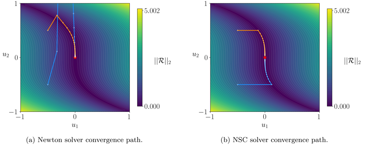
Figure 2: L2 norm of the residual vector and the nonlinear convergence history of the second test problem (Eq. 16) with the Newton and NSC solvers. The solution at (0,0) is highlighted with a red star.
