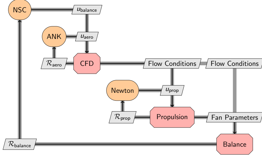
Figure 6: XDSM diagram of the nonlinear solver hierarchy.
