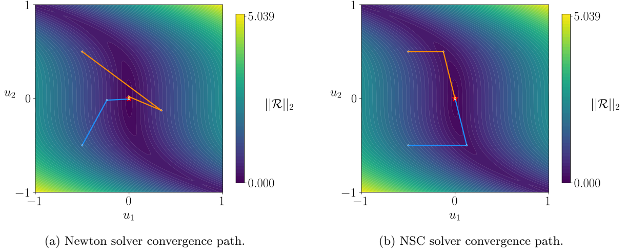
Figure 1: L2 norm of the residual vector and the nonlinear convergence history of the first test problem (Eq. 15) with the Newton and NSC solvers. The solution at (0,0) is highlighted with a red star.
