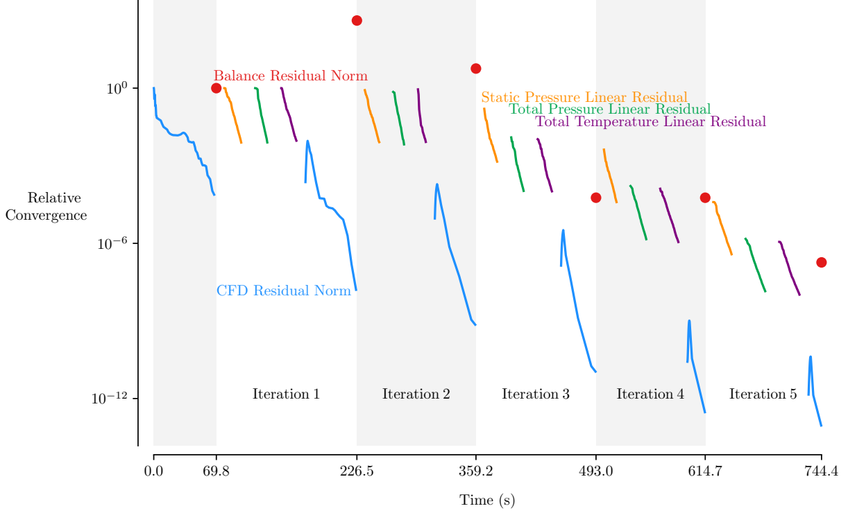
Figure 7: Relative convergence of various components of the NSC solver with respect to time from the initial CFD solution. The blue lines represent the nonlinear residual norm of the CFD model, while the orange, green, and purple lines show the linear residual for the three linear systems solved for the Schur update (Eq. 13). The red dots represent the residual norm of the balance equations.
