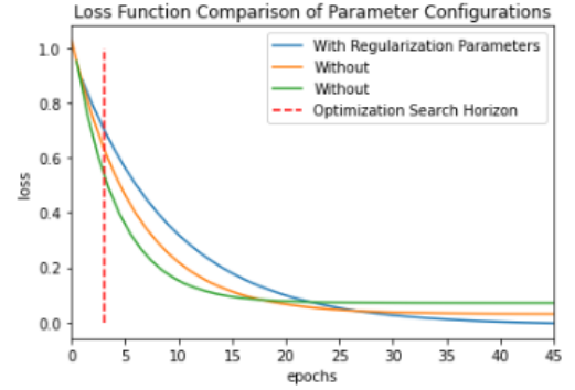
Fig. 5. Comparing the effect of regularization on the loss function.
