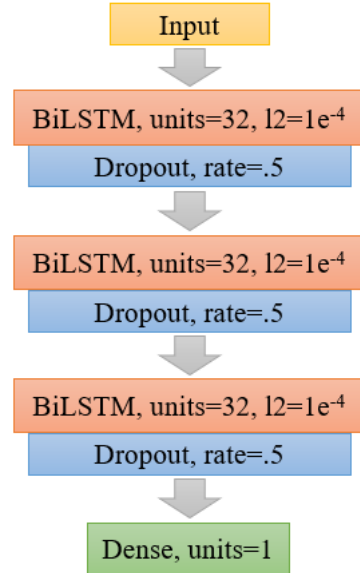
Fig. 6. Bi-LSTM Network for RUL Estimation
