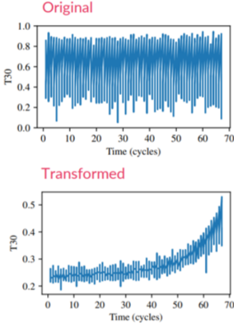
Fig. 4. Transformation of Raw Data into Prognosable Signals
