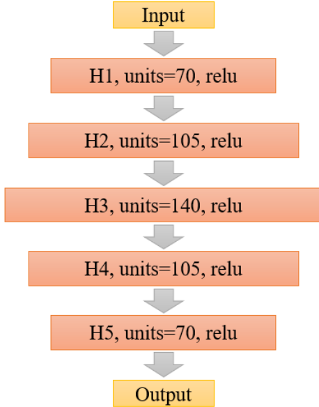
Fig. 3. Feedforward Network Architecture for Preprocessing Telemetry Data
