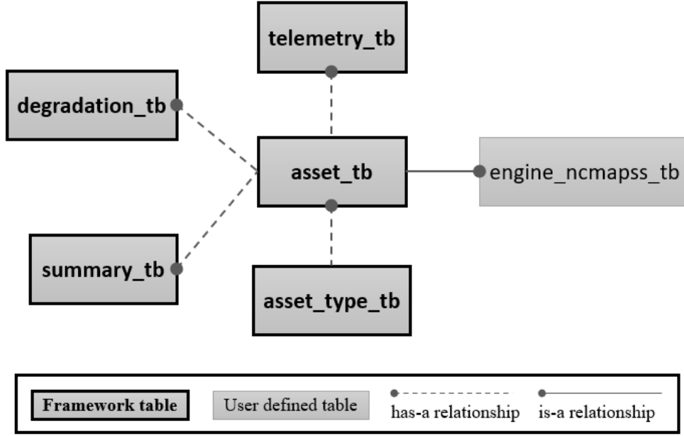
Fig. 2. Table Schema for N-CMAPSS Dataset
