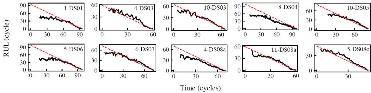
Fig. 7. Remaining Useful Life Estimation Test Results
