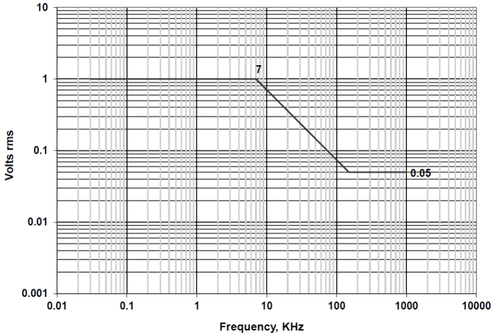
FIGURE 3.3.3-2: 28 VDC RIPPLE VOLTAGE SPECTRAL COMPONENTS
