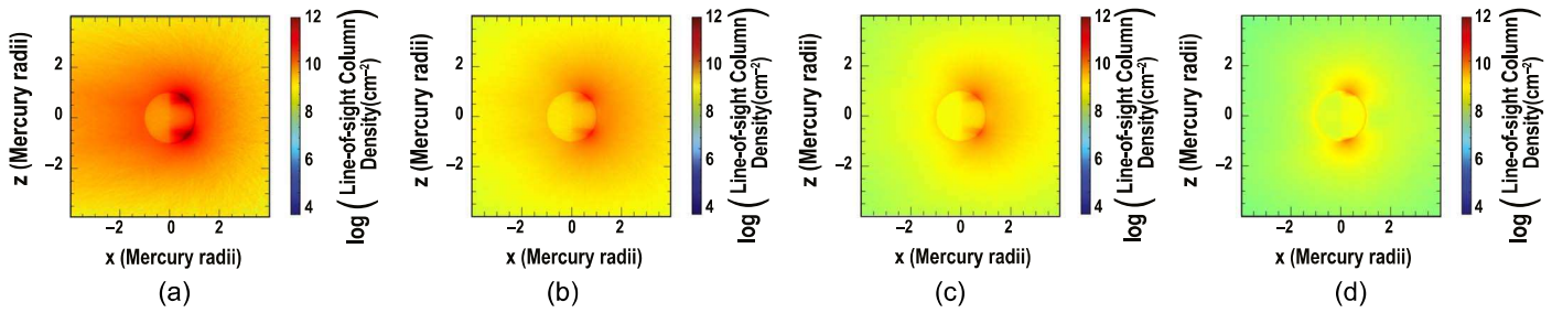
Figure 5. Comparison of the combination of IS (from both the northern and southern cusp) and IV, in which the simulation in Figure 4 for minimum IV flux has been added to IS exospheres for SBEs of (a) 0.27 eV, (b) 2.6 eV, (c) 4.4 eV, and (d) 7.9 eV. These illustrate where and to what extent the two processes can be distinguished.
