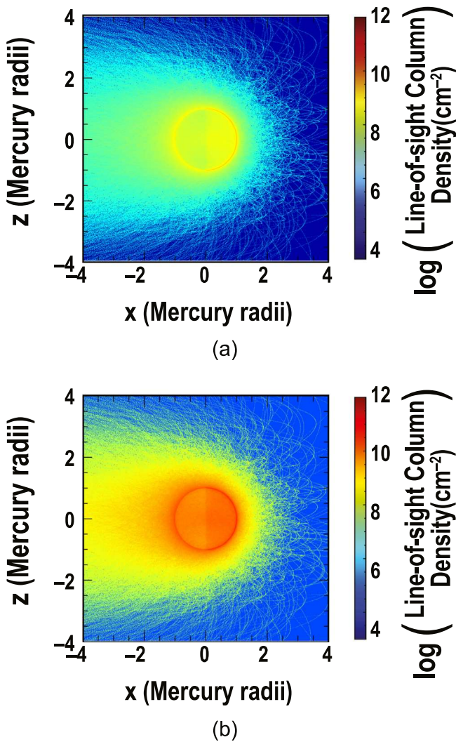
Figure 4. The IV-generated exosphere is simulated for the (a) lower limit and (b) upper limit from Mouawad et al. (2011). The image is seen from the dawn hemisphere centered on the terminator. The Sun is to the right and north is up.
