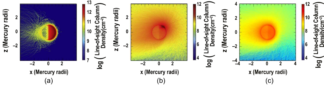
Figure 6. (a) PSD seen from the dawn equatorial terminator. (b) Maximum IV spot at dawn combined with IS at the northern cusp only and SBE = 0.27 eV. This provides an illustration of a single cusp being open to the solar wind. (c) Same as (b) but with SBE = 7.9 eV.
