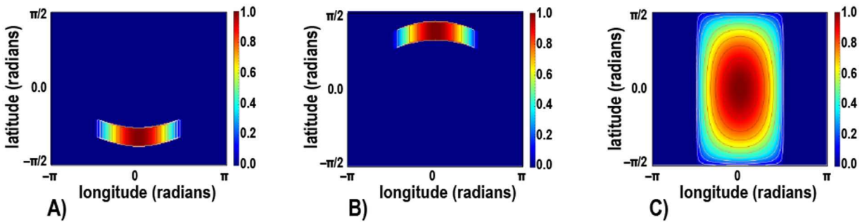
Figure 1. (a)–(b) Surface maps for IS in the south and north, respectively. The IS surface maps are based on measurements of the northern cusp by the MESSENGER FIPS instrument (Raines et al. 2014). They are only used as a reasonable basis for illustrating the differences resulting from the different SBE values, and are not necessarily reflective of actual open cusp areas at Mercury, especially in the southern hemisphere where similar measurements are not available. (c) Source map for PSD. The scaling is informed by fits to the MESSENGER MASCS data and diffusion-limited supply (Burger et al. 2010).
