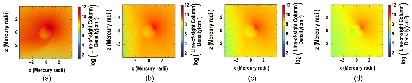
Figure 2. These simulations trace the gradual change in the exosphere derived from IS, from the northern cusp only, assuming SBEs of (a) 0.27 eV, (b) 2.6 eV, (c) 4.4 eV, and (d) 7.9 eV. The +x -axis is toward the Sun and +z is northward. Column density is the cumulative number of atoms \text{cm}^{-2} along the line of sight in the y -axis direction, which runs dawn–dusk and is perpendicular to the page.
