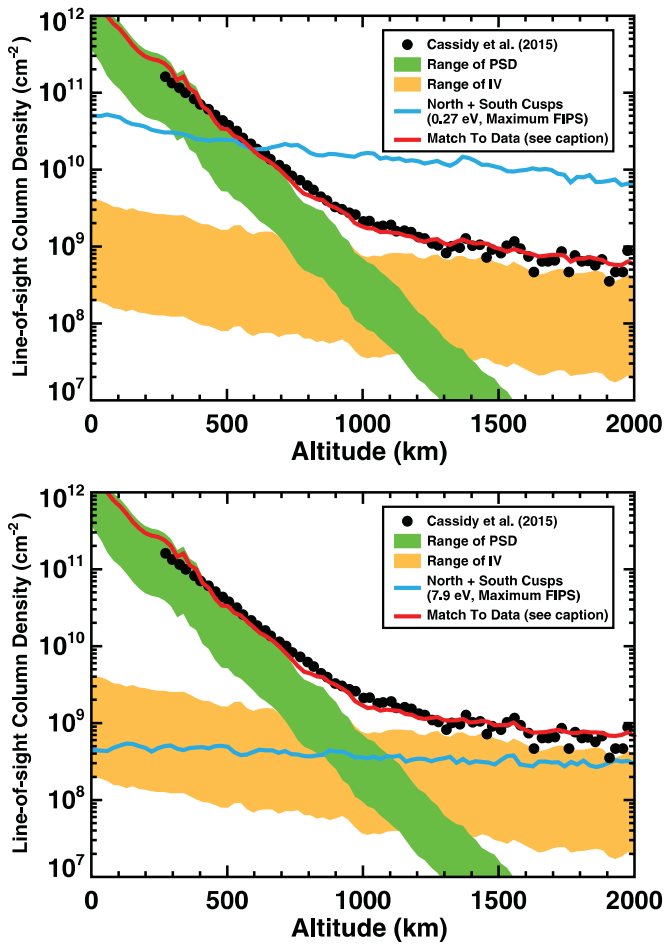
Figure 7. Comparisons of our models to MESSENGER data. The column density shown is an integrated line-of-sight value, not a zenith column. The data (black circles) are subsolar MESSENGER MASCS limb scan data at TAA 144° from Cassidy et al. (2015; upper-right panel of their Figure 6). The green regions indicate the range of PSD altitude profiles, with the lower edge corresponding to a PSD cross section of 1 \times 10^{-20} \text{ cm}^2 and f_{\text{Na}} = 0.02 (which we take as lower limits of both parameters), and the upper edge corresponding to the measured PSD cross section of 3 \times 10^{-20} \text{ cm}^2 and f_{\text{Na}} = 0.05 (we take as upper limits of both parameters). The orange regions indicate the range of IV altitude profiles, with the lower edge corresponding to the minimum IV case ( 1 \times 10^5 \text{ cm}^{-2} \text{ s}^{-1} ) and the upper edge to the maximum IV case ( 2.1 \times 10^6 \text{ cm}^{-2} \text{ s}^{-1} ) at 0.352 R_p of Mouawad et al. (2011). IV is always scaled as R_p^2 . The blue curves indicate the sum of the altitude profiles from IS in both the north and south cusps for SBE = 0.27 eV (a) and SBE = 7.9 eV (b) with an assumed flux equal to the MESSENGER FIPS-measured maximum ( 6.7 \times 10^8 \text{ ions cm}^{-2} \text{ s}^{-1} ; Raines et al. 2014). The red curves are example combinations of PSD, IV, and IS that match the data (see text for discussion). The red curve in (a) is the sum of PSD for the enhanced cross section and f_{\text{Na}} = 0.04 , IV for the maximum case, and 0.03 times the blue curve for the IS contribution (i.e., a flux of 2.0 \times 10^7 \text{ ions cm}^{-2} \text{ s}^{-1} ). The red curve in (b) is the sum of PSD for the enhanced cross section and f_{\text{Na}} = 0.04 , IV for the maximum case, and the blue curve for the IS contribution.
