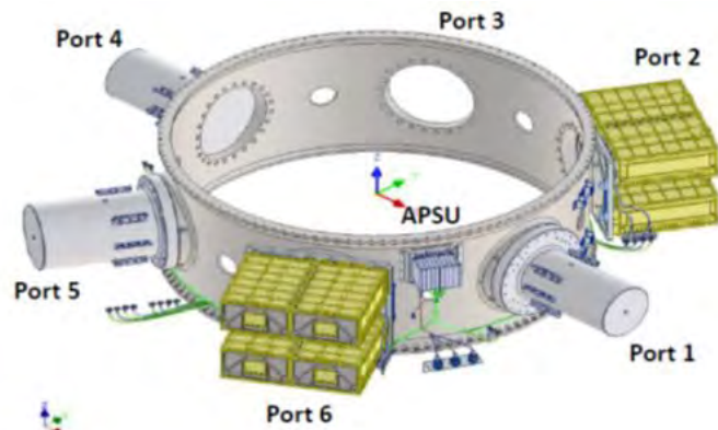
Figure 54: Landsat 9 Integration
