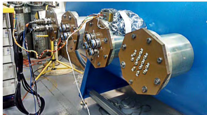
Figure 19. Thermal Vacuum Chamber Ports
