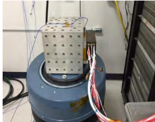
Figure 32: Vibration Test
