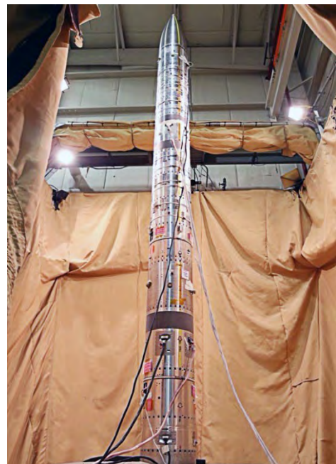
Figure 38: Spin Deployment Facility
