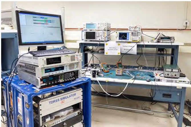
Figure 14: Microwave Lab Facility
