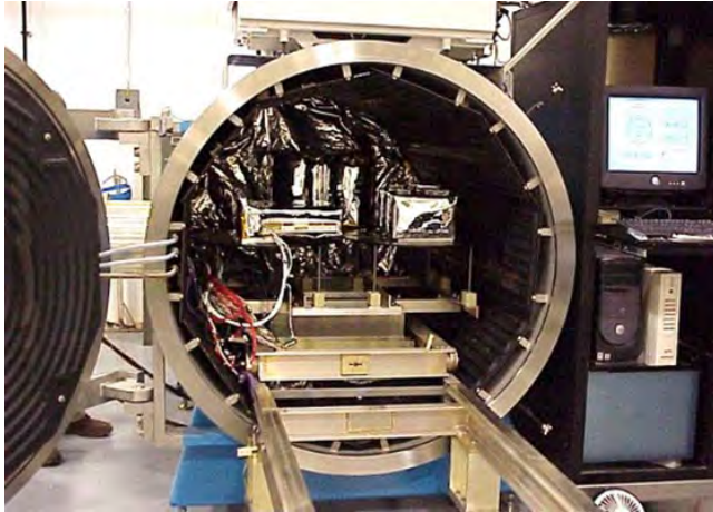
Figure 21. Thermal Vacuum Chamber used for small spacecraft, subsystems, and components
