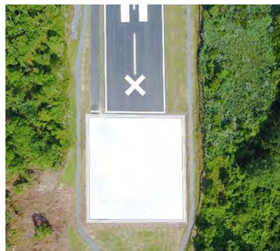
Figure 74: Concrete vertical takeoff and landing (VTOL) Pad rated to 5,000 psi
