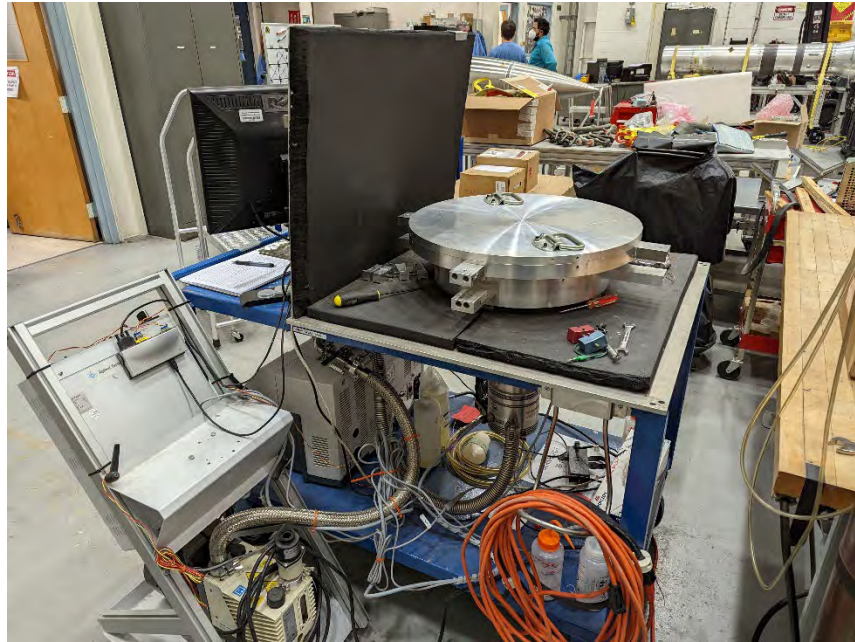
Figure 28: Vacuum Test Stand
