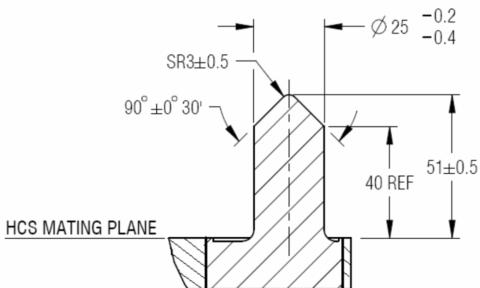
FIGURE 3.2.3.3-2 SECTION C-C
