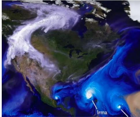
GEOS NWP
