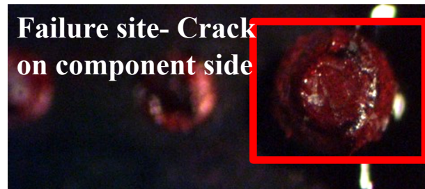
(b) Failure on component side
