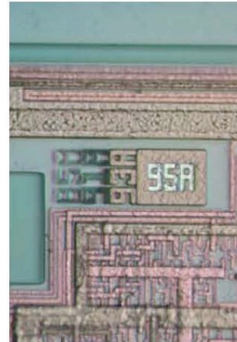
Optical images of a decapsulated part
