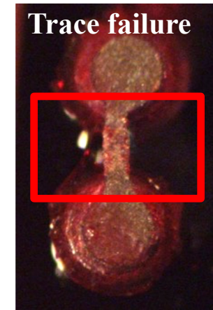
(b) Trace failure
