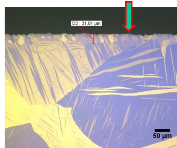
Abrasive wheel recrystallization depth ~ 30 micron
