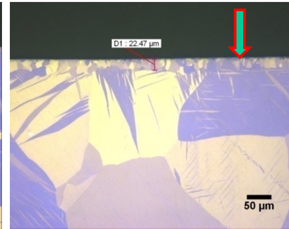
Precision blade recrystallization depth ~20 microns
