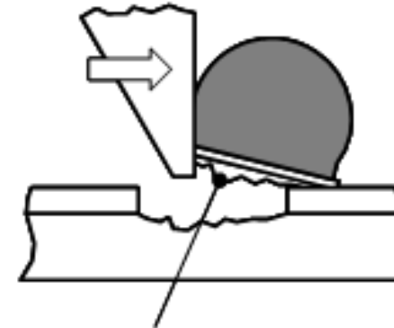
Lifted pad includes ruptured base material
