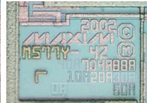
Optical images of a decapsulated part
