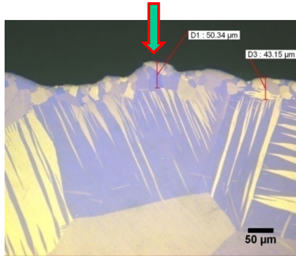
Band saw recrystallization depth ~50 microns
