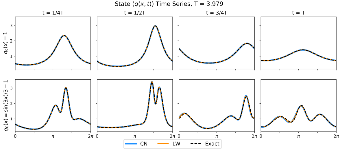
Figure B.1. Solutions to (B.1) for q_0(x) = 1 (top row) and q_0(x) = \sin(3x)/3 + 1 (bottom row) at four different times. The exact solution (black dashed) is shown along with finite-difference solutions using Crank-Nicolson (blue) and Lax-Wendroff (orange). The finite difference solutions are nearly indistinguishable from the exact solution.
