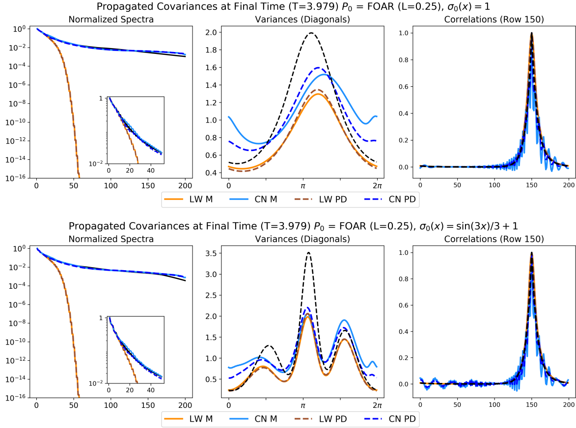
Figure 3.6. Same as Figure 3.5 for the FOAR correlation function with L = 0.25 .
