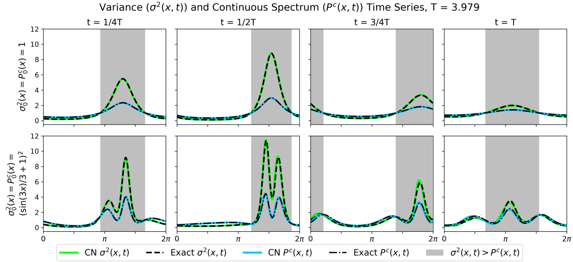
Figure 3.2. Top: Solutions to the one-dimensional variance equation (1.8) and continuous spectrum equation (1.9) at various times with velocity field (3.1), for unit initial condition (top row) and spatially-varying initial condition (bottom row) taken to be the square of (3.4). Time T = 3.979 corresponds to slightly after a full period. Exact solutions for each case are given in black dashed (variance) and black dot-dashed lines (continuous spectrum). Green curves denote the solution to the variance equation computed with Crank-Nicolson (abbreviated CN); blue curves are solutions to the continuous spectrum equation computed with Crank-Nicolson. Regions highlighted in grey correspond to regions where the exact solution to the variance equation is greater than the exact solution to the continuous spectrum equation, i.e. \sigma^2 > P^c ; unhighlighted regions correspond to regions where \sigma^2 < P^c .
