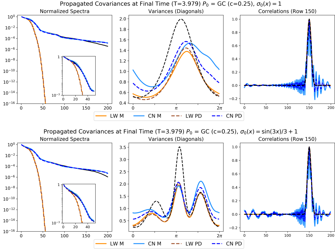
Figure 3.5. Same as Figure 3.3 for c = 0.25 .
