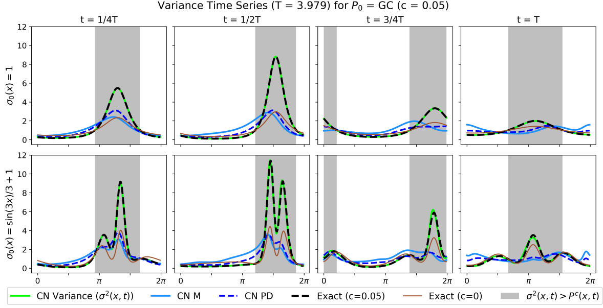
Figure 3.10. Variance time series for GC case with c = 0.05 . Top row: constant initial variance. Bottom row: spatially-varying initial variance. Diagonals extracted from the Crank-Nicolson traditional and polar decomposition propagation are shown (solid and dashed blue) as well as propagating the variance by solving the variance equation (one-dimensional version of (1.8)) independently using Crank-Nicolson (green). The exact solutions to the variance and continuous spectrum equations are shown in black dashed and solid brown and denoted as Exact ( c = 0.05 ) and Exact ( c = 0 ), respectively. Regions where the exact variance is larger (smaller) than the exact continuous spectrum are highlighted in grey (white).
