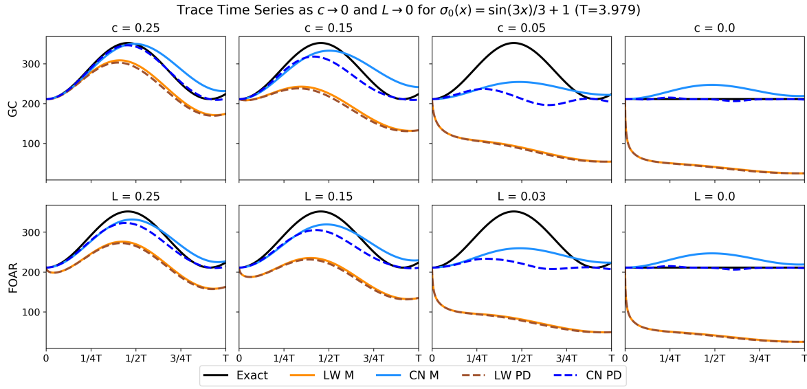
Figure 3.4. Trace time series for GC (top row) and FOAR (bottom row) for the spatially-varying initial variance (the square of (3.4)). Each panel corresponds to different values of c and L , decreasing from left to right towards c = L = 0 . Refer to Figure 3.3 for description of the curves. For the cases when c = L = 0 (rightmost panels), the exact solutions (solid black) are constant in time due to the fact that continuous spectrum solution P^c satisfies the continuity equation (1.9), hence its integral over space is constant.
