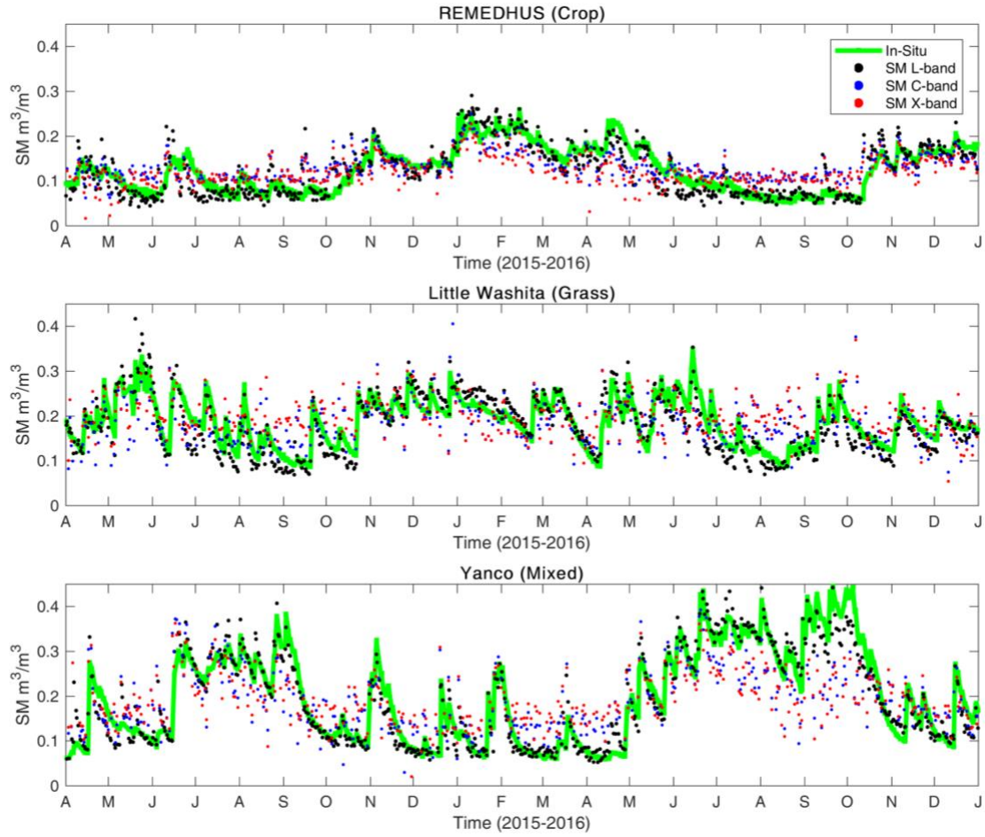
Figure 7. Soil moisture retrieval using the calibrated forward model parameters at L-band, C-band and X-band at V-pol together with soil moisture ‘truth’ from in situ monitoring stations at REMEDHUS, Little Washita and Yanco from April 2015 to December 2016.
