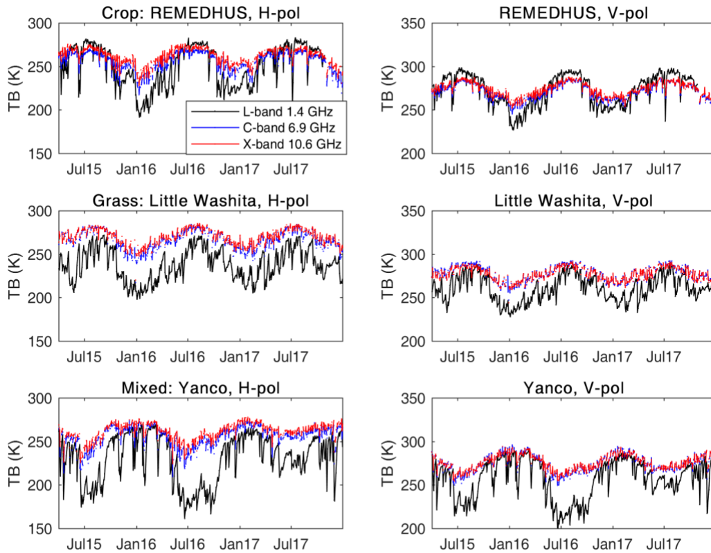
Figure 2. TB observations at H-pol and V-pol from SMAP (L-band, 1.4 GHz) and AMSR2 (C-band, 6.9 GHz and X-band, 10.6 GHz) at REMEDHUS, Little Washita and Yanco
