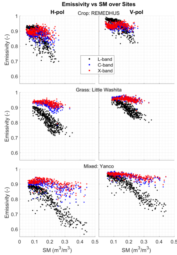
Figure 4. Scatter plots of surface emissivity ( TB/T_{SURF} ) against in situ soil moisture at L-, C- and X-band at H-pol and V-pol for REMEDHUS, Little Washita and Yanco.
