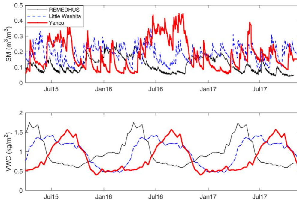
Figure 1. Time series of soil moisture from in situ monitoring stations (top) and vegetation water content retrieved from MODIS NDVI climatology (bottom) at REMEDHUS, Little Washita and Yanco from April 2015 to December 2017.
