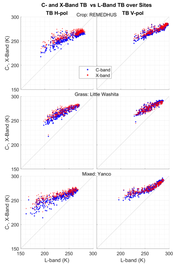
Figure 3. Scatter plots of TB observations at H-pol and V-pol from SMAP (L-band, 1.4 GHz) and AMSR2 (C-band, 6.9 GHz and X-band, 10.6 GHz) at REMEDHUS, Little Washita and Yanco.
