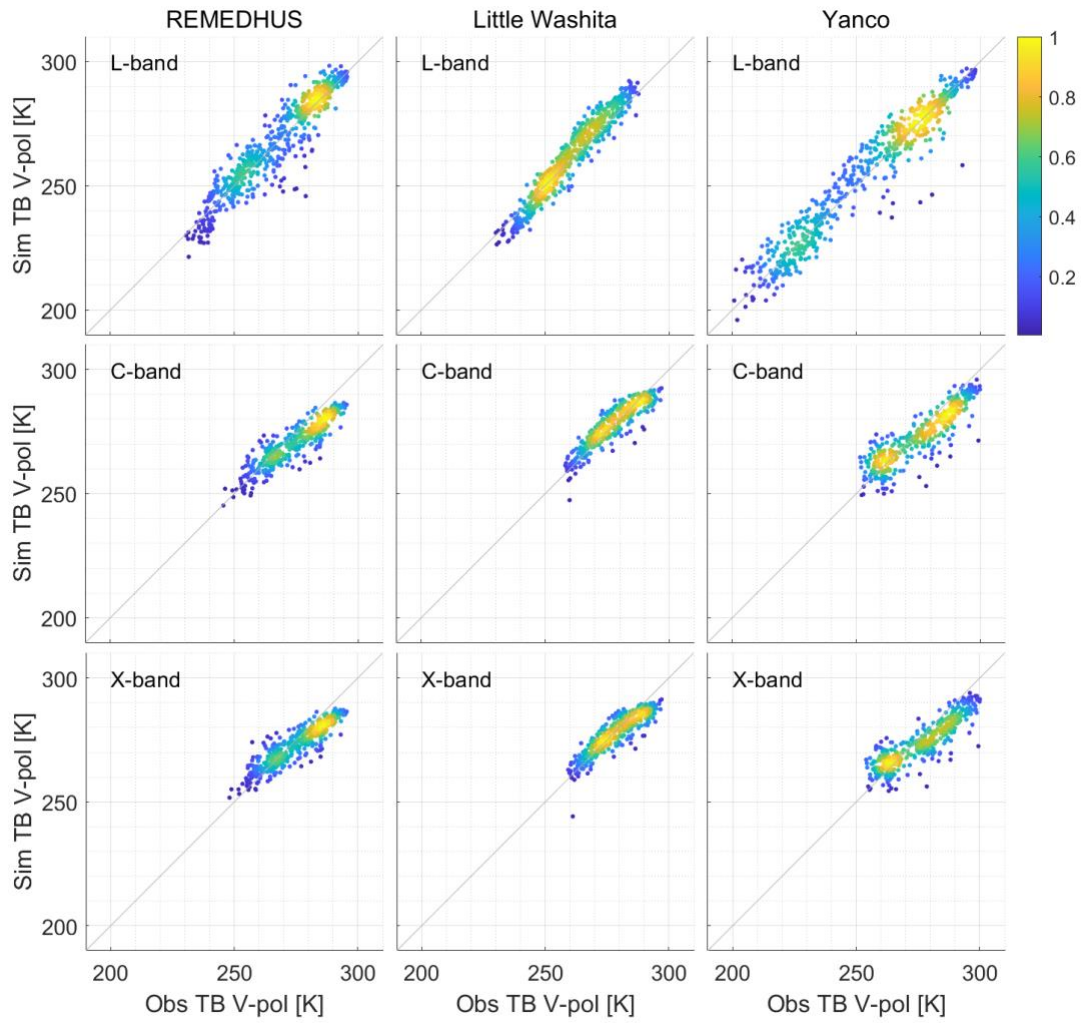
Figure 9. Scatter plots of simulated TB using calibrated parameters against observed TB at L-band, C-band and X-band at V-pol for REMEDHUS, Little Washita and Yanco for the period of 2015-2016. The colors reflect the normalized point density.
