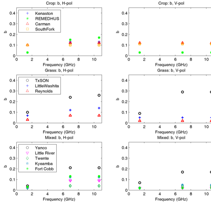
Figure 10. Calibrated vegetation parameter b for H-pol (left) and V-pol (right) for L-, C-, and X-band at core validation sites.
