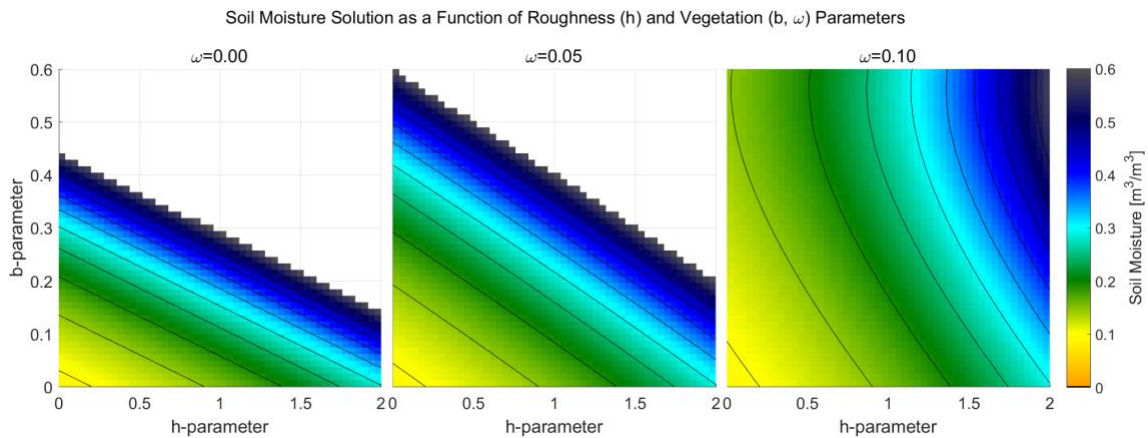
Figure 6. Soil moisture solutions as a function of h , b and \omega parameters for TB=270 K and VWC = 1.5 kg/m^2 .
