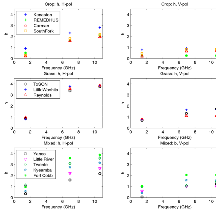
Figure 11. Calibrated roughness parameter h for H-pol (left) and V-pol (right) for L-, C-, and X-band at core validation sites.
