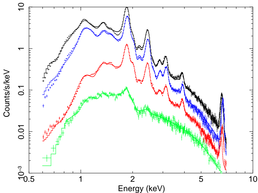
Figure 7. Four example spectra and best-fit models based on the automated fitting scripts. The colors correspond to those of the crossed squares in the C-statistic map in Fig. 6. The black line corresponds to the worst C-statistic. The fits are generally satisfactory, but the iron line centroids appear off in the top three spectra.
