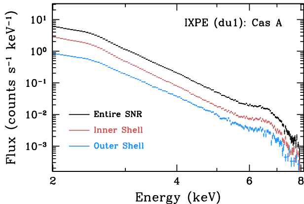
Figure 2. X-ray spectra of Cas A as detected by detector unit 1 of IXPE for three different extraction regions. The spectrum oversamples the spectral resolution, which is \Delta E \approx 0.5 at 2 keV—c.f. Appendix B for sample spectra of Cas A at a higher spectral resolution as obtained with the Chandra ACIS-S detector.
