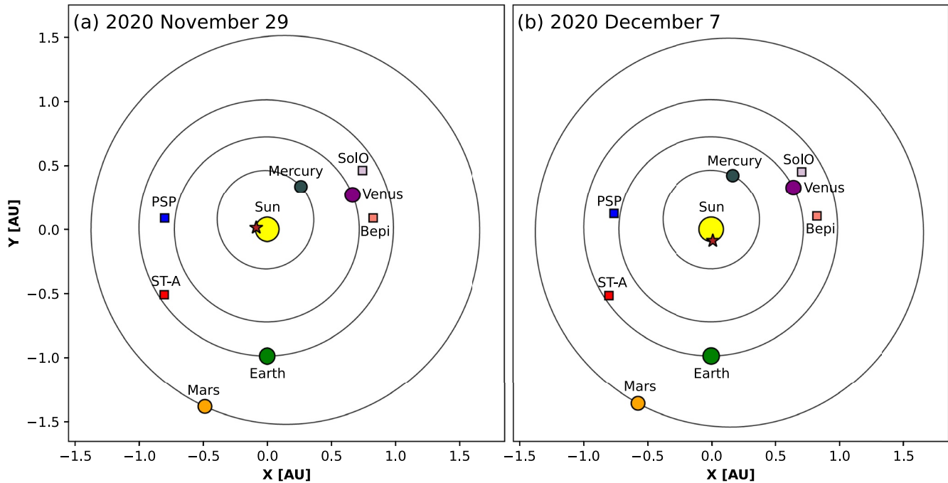
Figure 1. Position of planets and spacecraft in the inner heliosphere on (a) 29 November 2020 and (b) 7 December 2020. The orbits of all planets are also indicated. The locations of (a) Flare1 and (b) Flare2 are marked with star symbols on the surface of the Sun. Bepi = BepiColombo; PSP = Parker Solar Probe; SoLO = Solar Orbiter; ST-A = STEREO-A.
