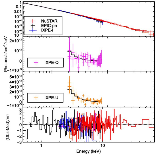
Figure 1. Spectro-polarimetric fit of the NuSTAR (red), XMM EPIC-pn (black), and IXPE (blue, magenta, and orange) spectra. From the top to the bottom, we show the fit of the I , Q , U spectra and the residuals of the best fit model (solid line). The spectral channels have been rebinned for clarity.
