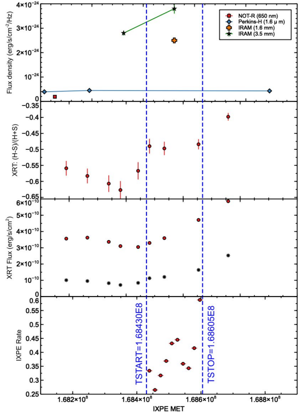
Figure 3. From the top to the bottom: light-curves of the optical, infrared and millimeter flux densities, light-curve of Swift XRT hardness ratio, light-curve of the soft (S band: 0.3-2.0 keV) and hard (H band: 2.0-10.0 keV) Swift XRT fluxes, and light-curve of the IXPE count rates. In the first panel, the legend displays the symbols for the different instruments and wavelengths. Multiple data points from the same instrument are connected by a line to guide the eye. In the third panel, soft and hard fluxes are coded as red circles and blue asteriks. The dashed vertical lines indicate the beginning and the end of the IXPE observation.
