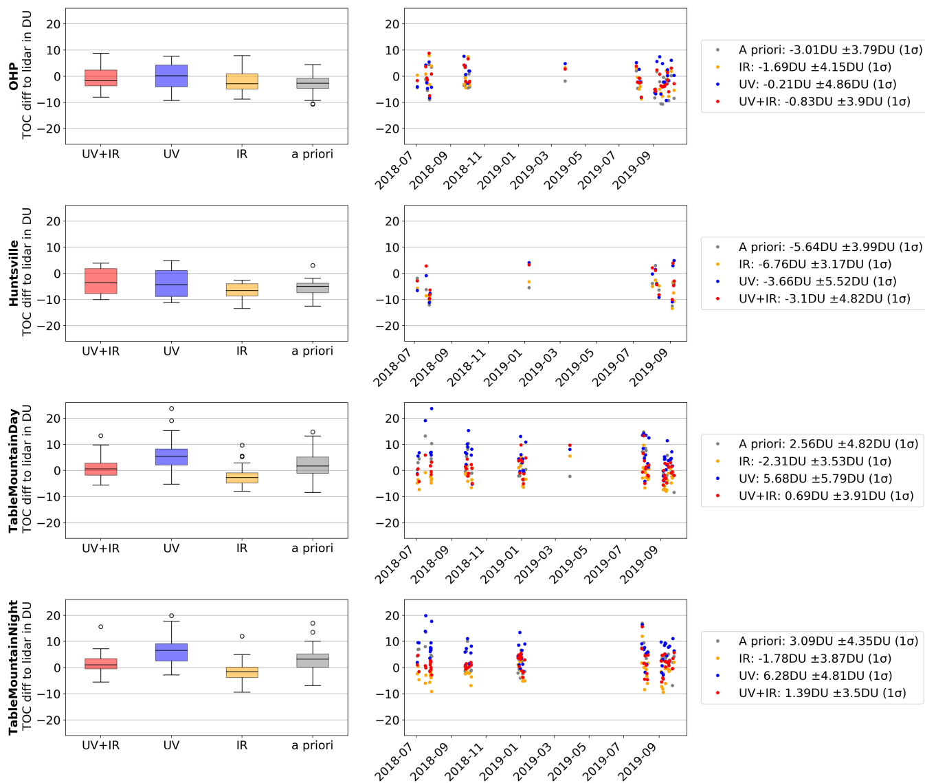
Figure 6. Absolute differences in the tropospheric ozone content (TOC) with respect to the tropospheric lidar data. The differences are shown as Box-Whisker plots in the left panels and as time series in the middle panels. The right panels show statistical information (mean absolute differences and the standard deviations). TOCs are calculated by integrating ozone profiles from the lowermost retrieval level altitude up to the tropopause. The height of the tropopause is obtained from the ERA5 reanalysis data using the 2PV definition.
