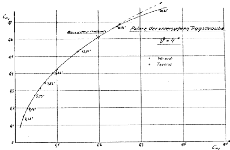
Fig. 6: Polar of the autorotating airscrew, comparison of calculation with wind tunnel measurements
