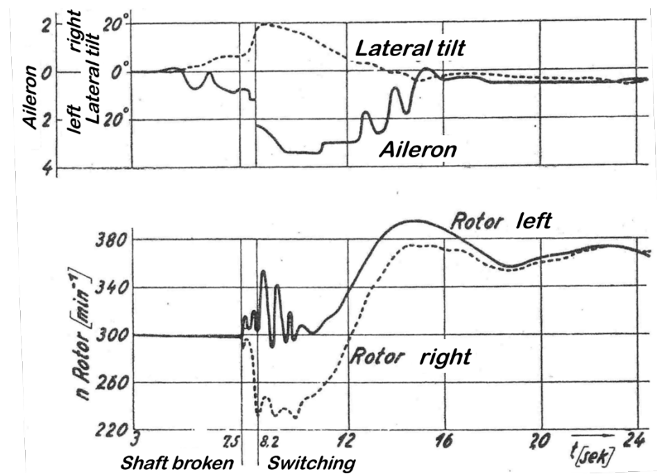
Fig. 4: Fw 61. One-sided switchover after shaft break from V = 40 km/hr
