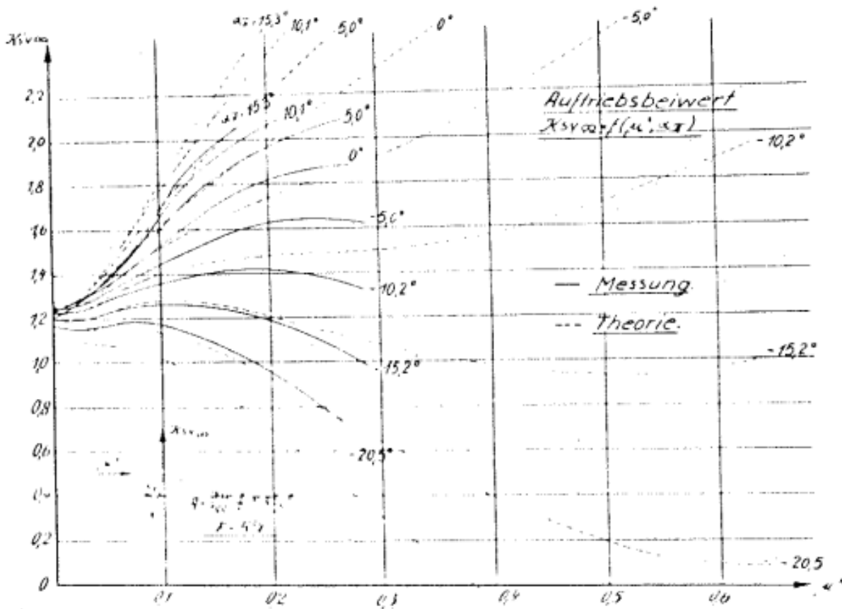
Fig. 8: Vertical thrust coefficient as function of advance ratio.
