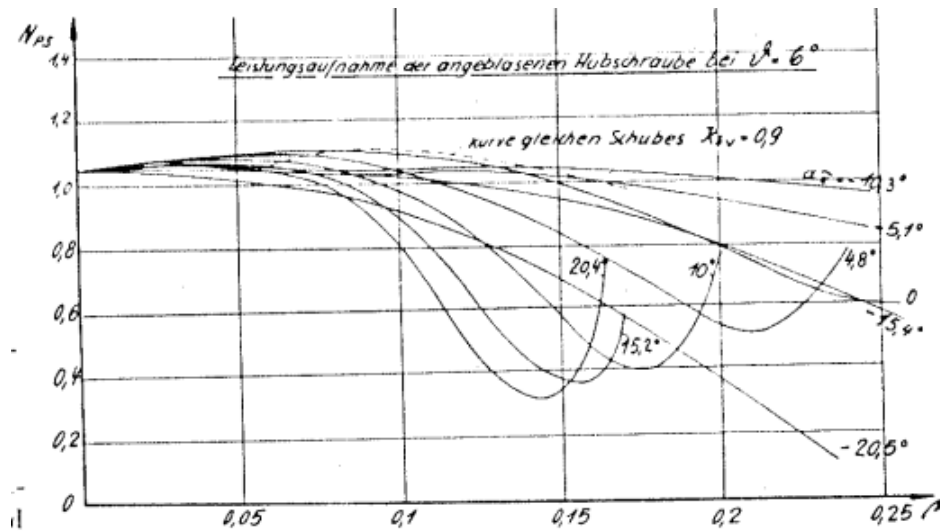
Fig. 26: Power consumption of a lifting screw versus advance ratio
