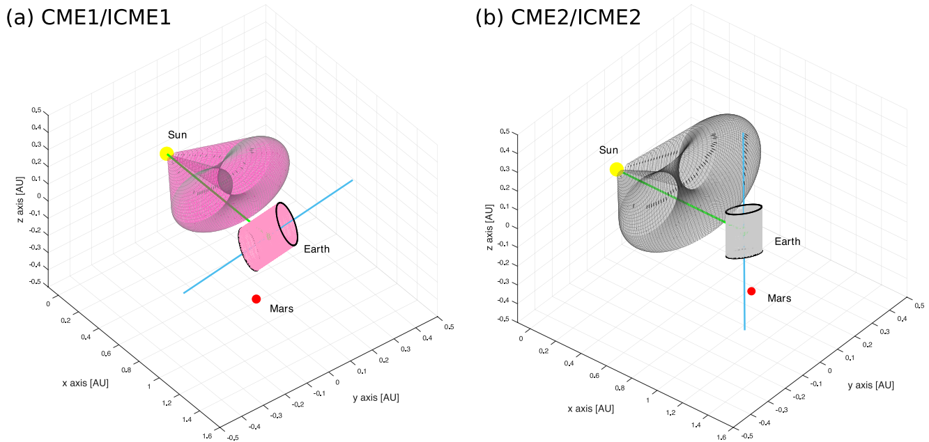
Figure 7. Comparison of the Graduated Cylindrical Shell (GCS)-derived coronal mass ejection (CME) orientation in the solar corona and Elliptic-Cylindrical (EC)-derived interplanetary coronal mass ejection (ICME) ejecta orientation at Earth for (a) CME1/ICME1, in pink, and (b) CME2/ICME2, in gray. The crossant-like features show the CME morphology obtained via the GCS reconstructions shown in Figure 2, whilst the cylinders represent the corresponding ICME structures retrieved via the EC fits displayed in Figure 5.
