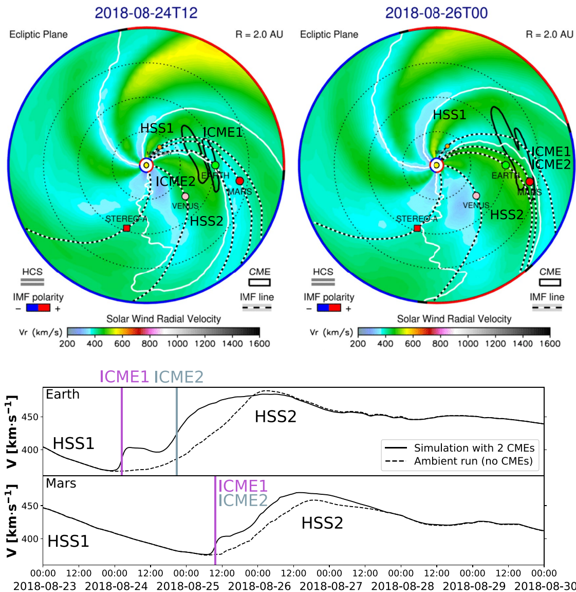
Figure 4. Overview of the WSA–Enlil simulation results at Earth and Mars. Top: Snapshots of the simulation results for the radial speed V_r on the ecliptic plane around the arrival times at (left) Earth and (right) Mars. Bottom: Results for the solar wind speed V at Earth and Mars.
