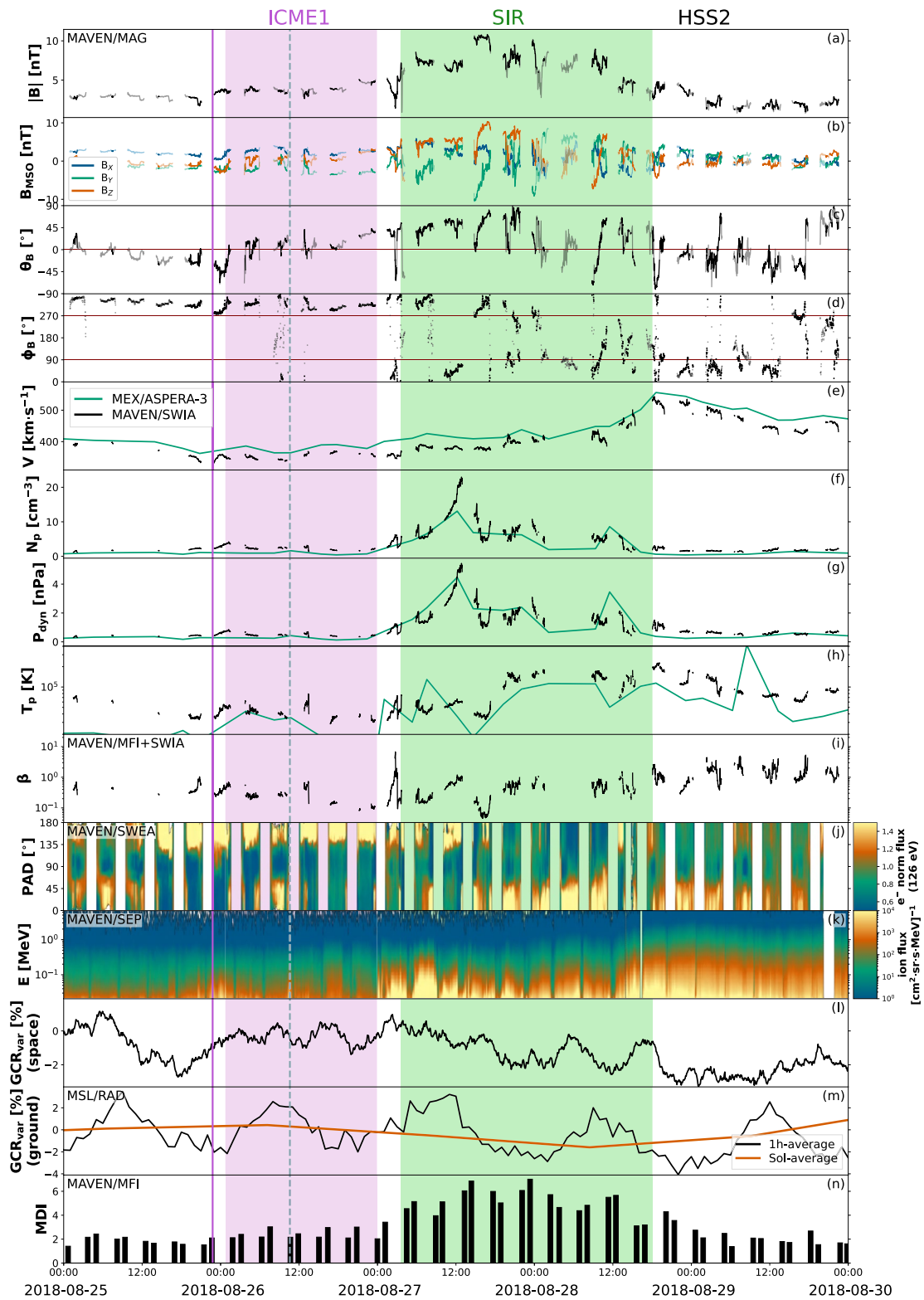
Figure 6. In-situ measurements at Mars, showing (a) magnetic field magnitude, (b) magnetic field components in Mars Solar Orbital coordinates, (c) \theta and (d) \phi components of the magnetic field, solar wind (e) speed, (f) density, (g) dynamic pressure, and (h) temperature, (i) plasma \beta , (j) electron pitch angle distribution, (k) ion intensities, galactic cosmic ray variation (l) in space and (m) on ground, and (n) Magnetospheric Disturbance Index index, quantifying arieeffectiveness. The lighter portions of magnetic field data are sampled in the Martian foreshock rather than in the solar wind.
