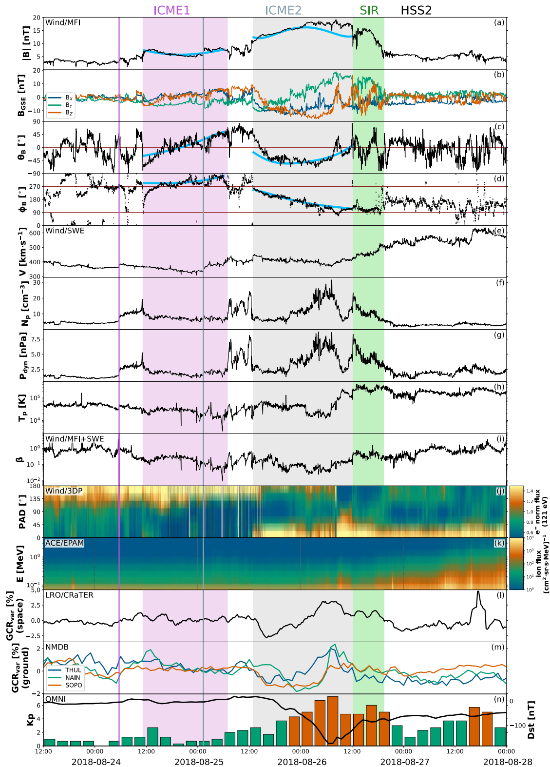
Figure 5. In-situ measurements at Earth, showing (a) magnetic field magnitude, (b) magnetic field components in Geocentric Solar Ecliptic coordinates, (c) \theta and (d) \phi components of the magnetic field, solar wind (e) speed, (f) density, (g) dynamic pressure, and (h) temperature, (i) plasma \beta , (j) electron pitch angle distribution, (k) ion intensities, galactic cosmic ray variation (l) in space and (m) on ground, and (n) Kp and Dst indices, quantifying geoeffectiveness. The ejecta intervals show flux rope fitting results with the Elliptic-Cylindrical model superposed on the magnetic field data.
