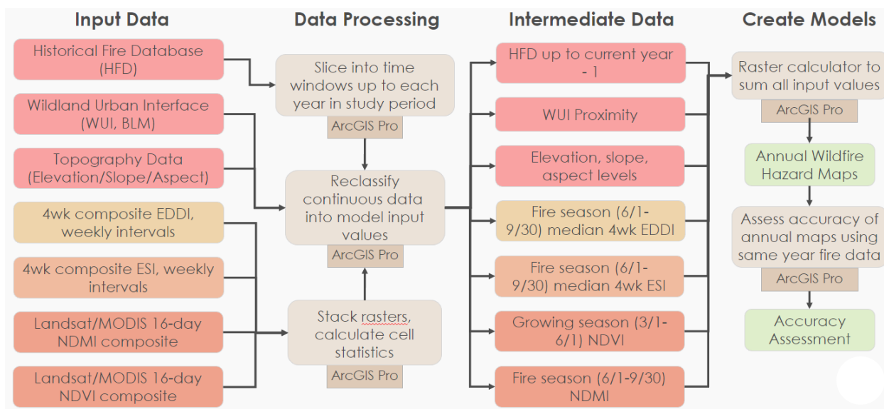
Figure C2: Flowchart of Wildfire Hazard Modeling performed during Term 1 of Idaho Wildfires.
