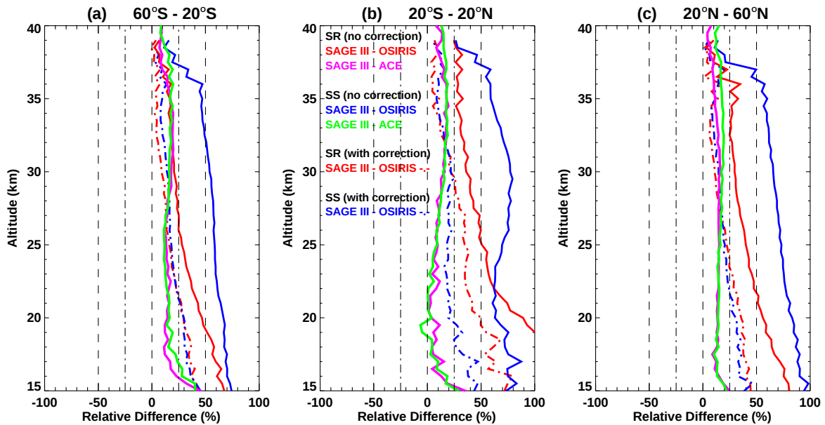
Fig. 7: The percent difference between SAGE III/ISS sunrise (SR) and sunset (SS) NO 2 and OSIRIS and ACE-FTS observations averaged over three latitude bands. The OSIRIS comparisons without application of diurnal corrections are shown in solid red and blue lines for sunrise and sunset, respectively, while the comparisons with the diurnal scaling factors are shown in dashed red and blue lines for sunrise and sunset, respectively.
