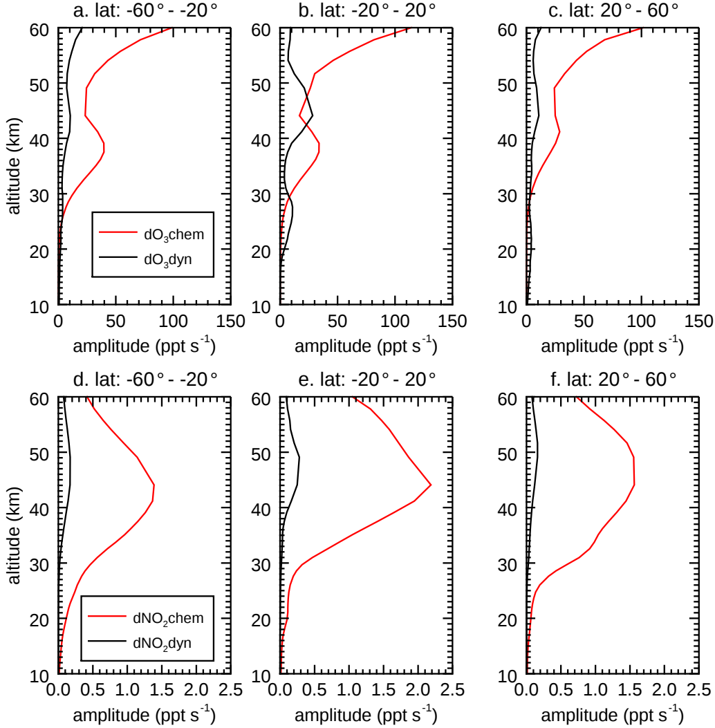
Figure 1: The amplitude of the diurnal cycle of the simulated O 3 tendency (top) and NO 2 tendency (bottom) due to dynamics (black) and chemistry (red) for January 2019, averaged over three latitude bands.
