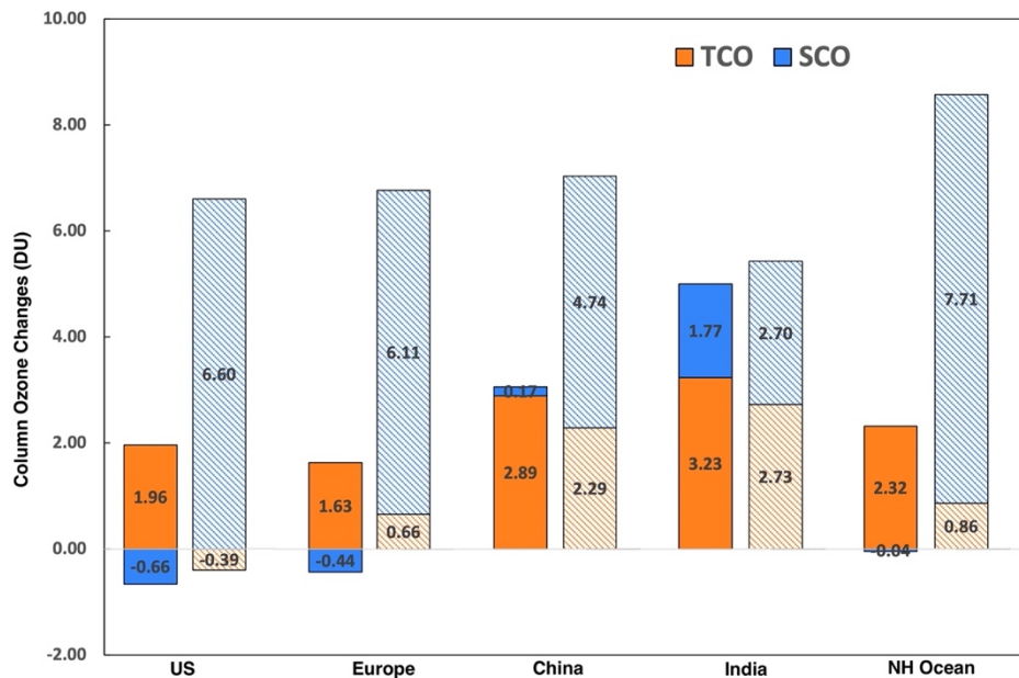
Figure S1: Changes in tropospheric column ozone (TCO, red) and stratospheric column ozone (blue) between 2005 and 2018 averaged over averaged over anthropogenic emission regions (US, Europe, China and India) and NH Ocean background region calculated from observations (bars with solid color) and RefD1 simulation (bars with patterned color).
