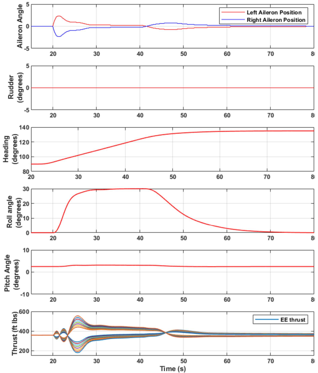
Figure 14. Coordinated turn using EEs instead of rudder. The ailerons manage the 30-degree bank, accounting for the roll induced by the EEs. The bottom plot shows the EE thrust distribution across the wings, where that of the outermost EEs varies the most.
