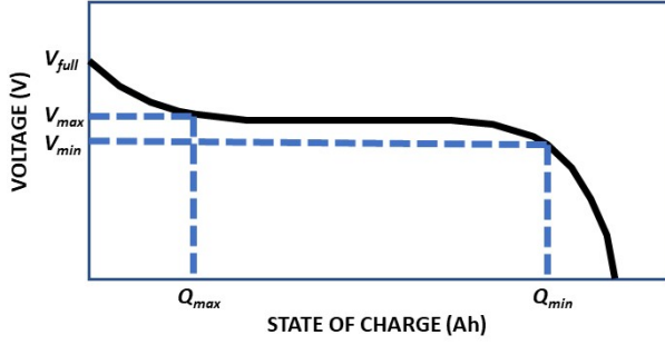
Figure 11. Battery Discharge Curve.
