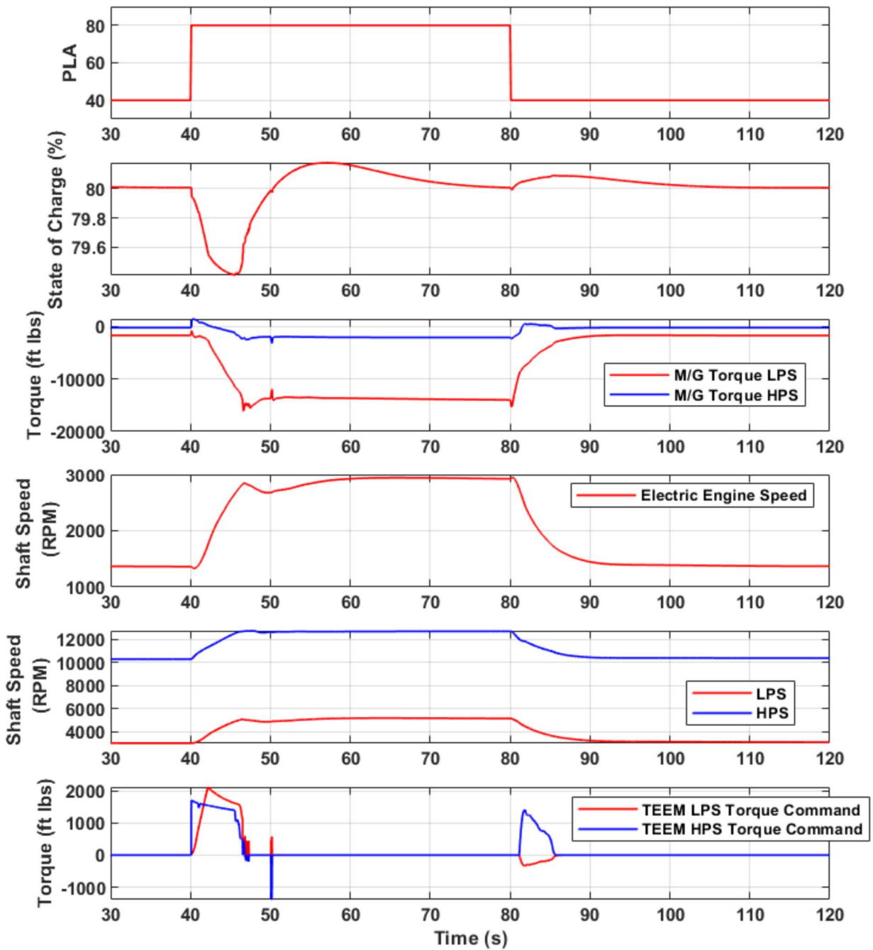
Figure 13. Burst and Chop transient. The top plot shows the power command. The second plot shows the battery SOC throughout the transient. The third plot shows the total torque on both the LPS and HPS. The fourth plot shows the EE speed. The fifth plot shows the LPS and HPS speed. The last plot shows the torque command due to the TEEM control, the result of which is visible in the third plot.
