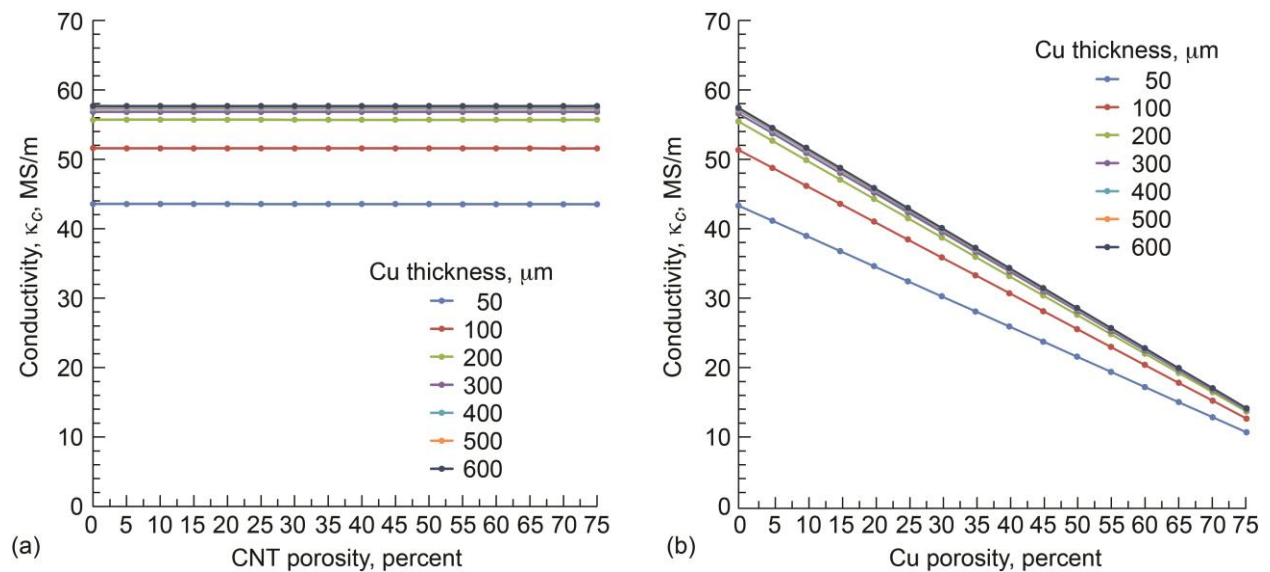
Figure 7.—Calculated theoretical electrical conductivity \kappa_c of Cu/CNT composite (at CNT diameter d_{\text{CNT}} = 100 \mu\text{m} and increasing Cu thickness) versus component porosity. (a) Changing CNT porosity X_{\text{CNT}} . (b) Changing Cu porosity X_{\text{Cu}} .
