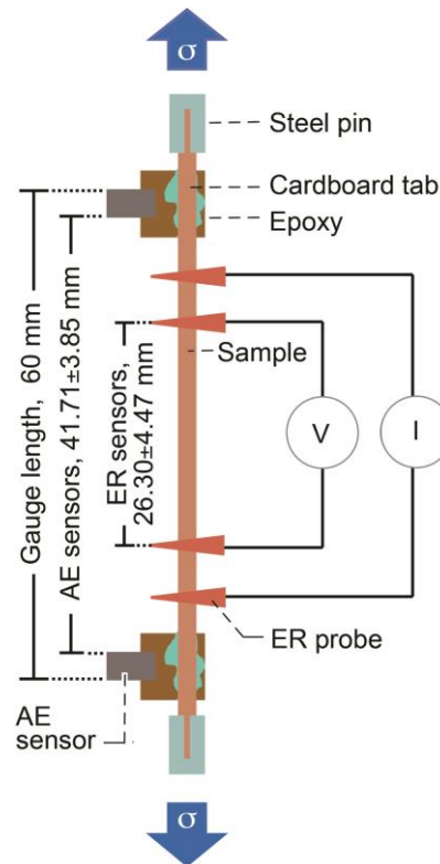
Figure 4.—Tensile test, indicating voltage (V) and current (I) measuring devices,
