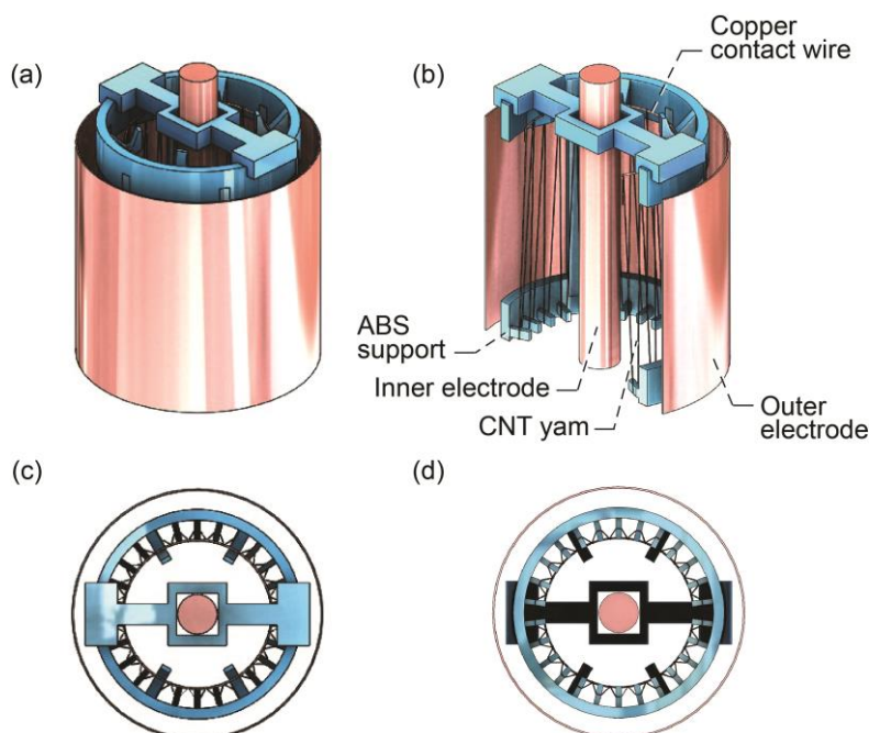
Figure 3.—Cu-carbon nanotube (CNT) electroplating setup, three-dimensional printed from acrylonitrile butadiene styrene (ABS). (a) Full view. (b) Cross-sectional view of setup strung with CNT yarn for plating. (c) Top view. (d) Bottom view.
