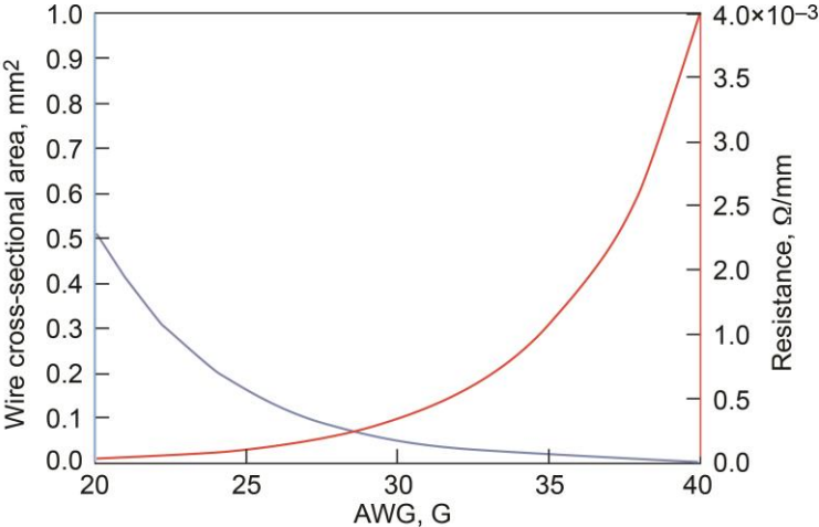
Figure 1.—Cross-sectional area and specific resistance versus Cu-based American Wire Gauge (AWG). 5
