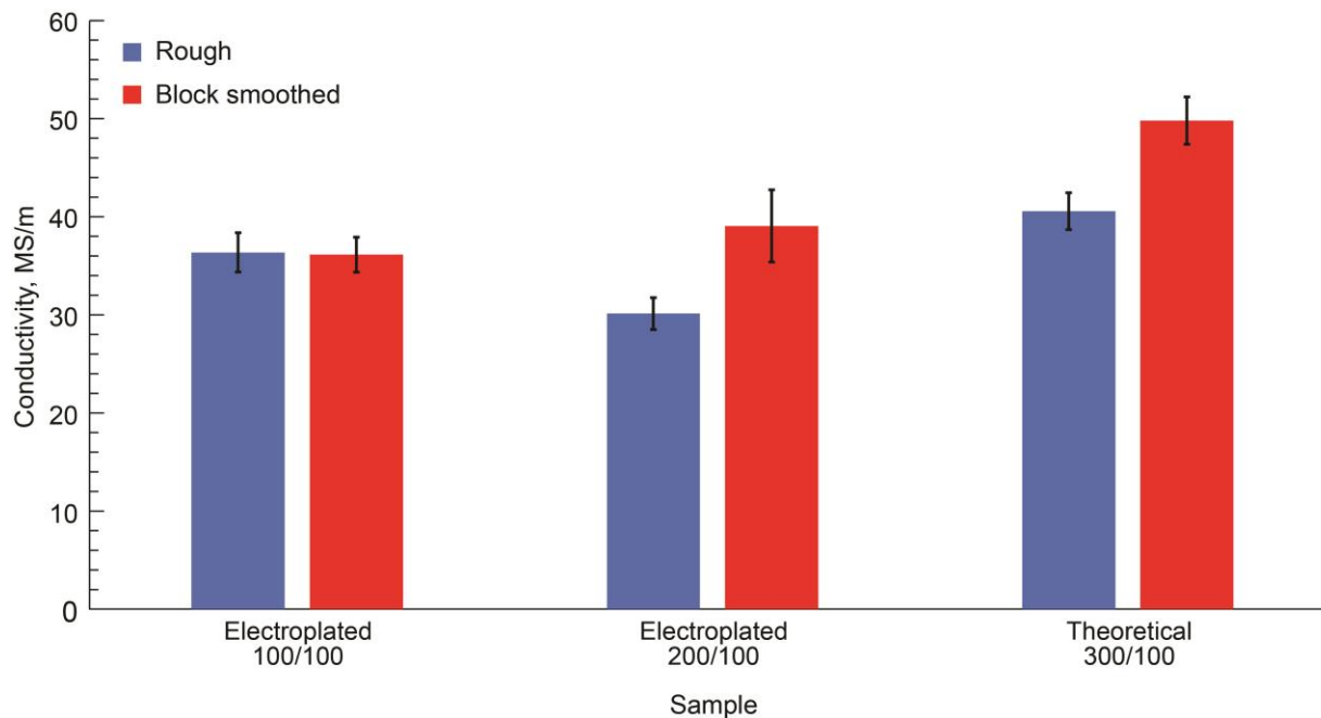
Figure 12.—Effect of surface finish on measured electrical conductivity of electroplated Cu/CNT samples.
