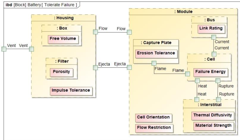
Figure 2. Enabling Tolerate Failure Functionality
