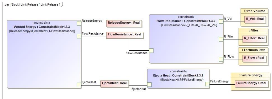
Figure 11. Limit Release Parametric Diagram
