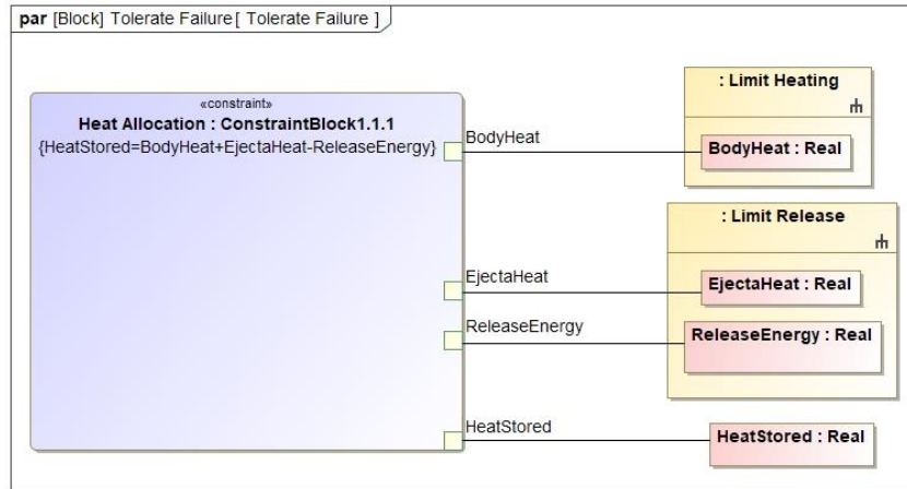
Figure 5. Tolerate Failure Parametric Diagram
