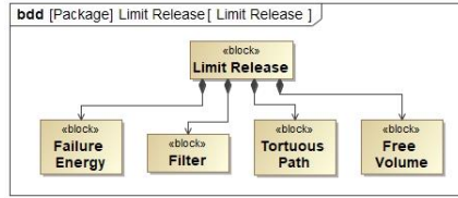
Figure 9. Limit Release BDD
