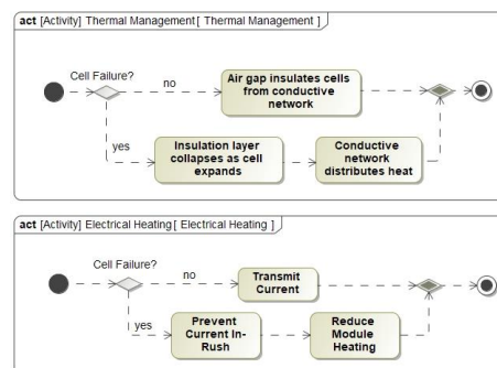
Figure 7. Limit Heating Design Activities
