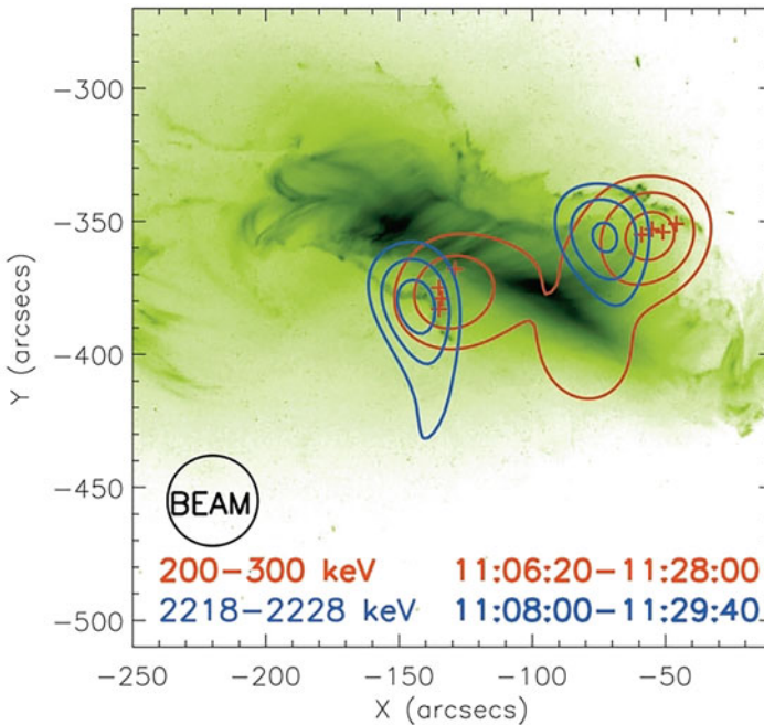
Fig. 5 Overlay of gamma-ray and X-ray contours on a TRACE 195 Å image of the 28 October 2003 flare. (From Hurford et al. 2006)
