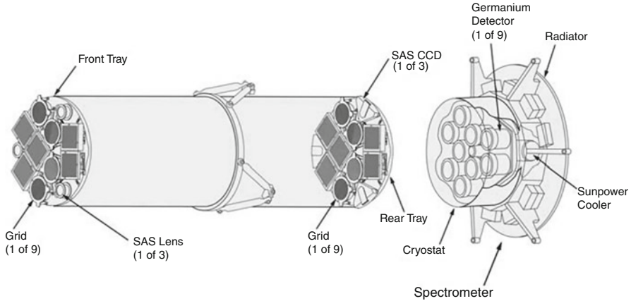
Fig. 1 Perspective of RHESSI showing the components necessary for imaging. Two essentially identical sets of nine grids are mounted on front and rear grid trays, with all the grids made of tungsten except for the finest grid pair that was made of molybdenum for ease of etching. A corresponding set of nine cooled germanium detectors is mounted behind the rear grids. The solar aspect system (SAS) consists of three lenses mounted on the front grid tray that focus optical images of the Sun onto three linear diode arrays (labeled SAS CCD in the figure) on the rear grid tray. It provides sub-arcsec knowledge of the radial pointing with respect to Sun center. Two optical roll angle systems (RASS, not shown) pointed perpendicular to the spin axis detect multiple stars each spacecraft rotation and provide the necessary roll angle information. The combined SAS and RAS data enables the absolute orientation of the grids to be determined on millisecond time scales and allows X-ray sources to be located on the solar disk to sub-arcsec accuracy (Fivian et al., 2002). (From Hurford et al. 2002)
