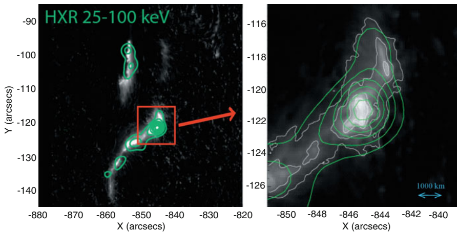
Fig. 11 Hard X-ray (green contours) and white light (G-band) imaging of a flare ribbon for a flare on 6 December 2006 reported by Krucker et al. (2011). The left image shows the two ribbons. The right image is an enlargement of the brightest part of the southern ribbon. (From RHESSI Science Nugget #142 available from https://hesperia.gsfc.nasa.gov/rhessi3/news-and-resources/results/nuggets/ )
