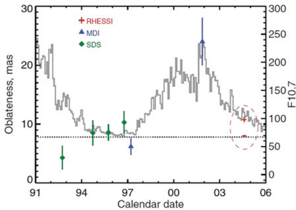
Fig. 14 Comparison of oblateness measurements from space. The RHESSI oblateness measurements are from data from 29 June to 24 September 2004 (red crosses). Results are also shown from the balloon-borne Solar Disk Sextant (SDS) (green diamonds) and the MDI instrument on board SOHO (blue triangles). The surface rotation rate predicts the value shown with the dotted line. The histogram (scaled to the uniform-rotation oblateness at solar minimum and to the higher MDI data point) shows the radio flux index F10.7, a good indicator of the solar cycle. (From Fivian et al. 2008 with permission of H. Hudson)
