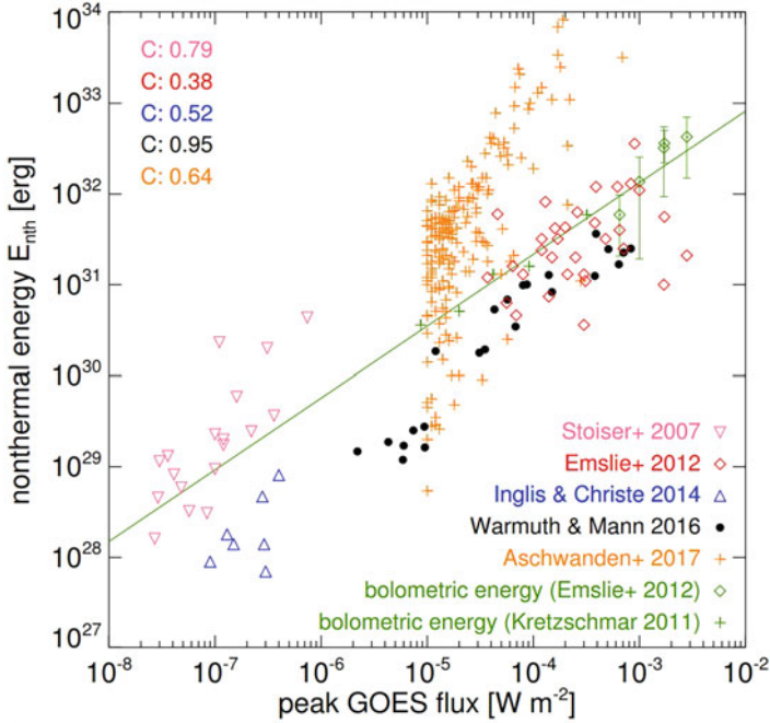
Fig. 6 Energy in non-thermal electrons, E_{nth} , plotted versus peak GOES flux for all five studies. For comparison, the total radiated energies E_{bol} derived from SORCE/TIM (green diamonds) and SOHO/VIRGO (green crosses). The green line is a power-law fit to these data points). (From Warmuth and Mann 2020 with permission of A. Warmuth)
