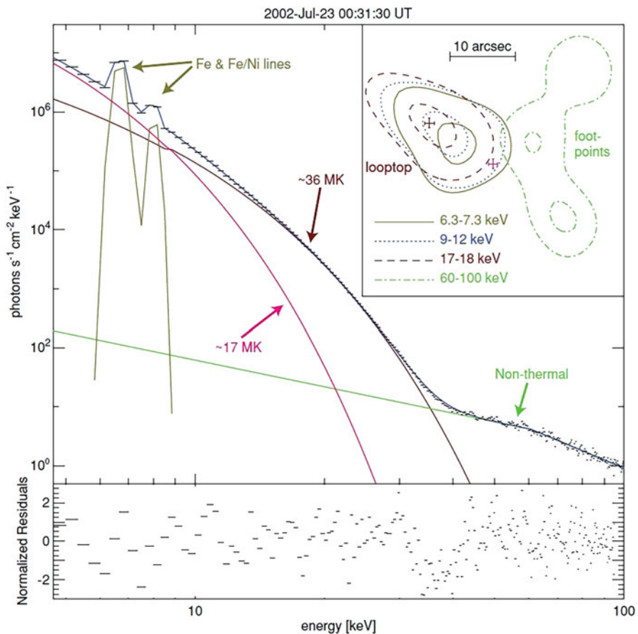
Fig. 12 X-ray spectrum and image of the 2002 July 23 X4.8 flare. (From Caspi and Lin 2010 with permission of A. Caspi)
