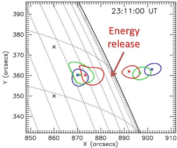
Fig. 8 RHESSI images made for a flare on 15 April 2002 at 23:11:00 UT showing twin thermal X-ray sources and the presumptive location of the coronal energy release site. Color-coded contours at 80% of the peak flux in each case, and asterisks marking the centroids, are shown for three energy bins. For the contours to the left on the solar disk, the energy bins were 6–8, 10–12, and 16–20 keV. In this case, the source is presumed to be at the top of a large, symmetric magnetic loop joining the two footpoints seen in other images and marked here with crosses. For the contours to the right above the solar limb, the energy bins were 10–12, 12–14, and 14–16 keV. In each case, the color coding was blue, green, and red, respectively. (From Sui and Holman 2003 with permission of L. Sui)
