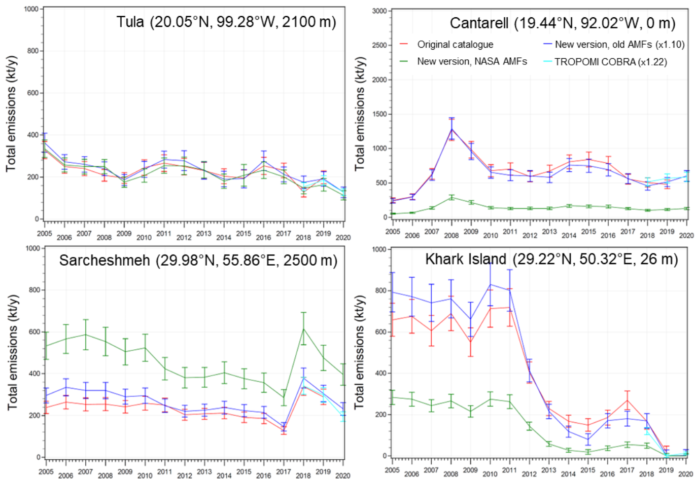
Figure 1. Four examples of SO 2 emission estimates with 2σ error bars from the original catalogue (red), emissions estimated from OMI Version 2 SCD values and converted to VCDs using the same AMFs as in the original catalogue (blue), and emissions estimated using Version 2 OMI VCD data (green). We also included TROPOMI-based estimates (cyan). The emission source names, coordinates, and elevations above sea level are shown. TROPOMI-based estimates were increased by 22% and OMI and OMPS data were increased by 10% as discussed in the text.
