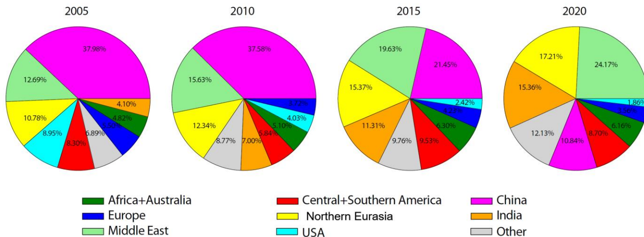
Figure 8. (Top) Pie charts of contributions to total SO 2 emissions by the source type. Power plants are the main source of emissions and degassing volcanoes contribute between one quarter to one third of total emissions. (Bottom) Pie charts of contributions to total anthropogenic SO 2 emissions by region.
