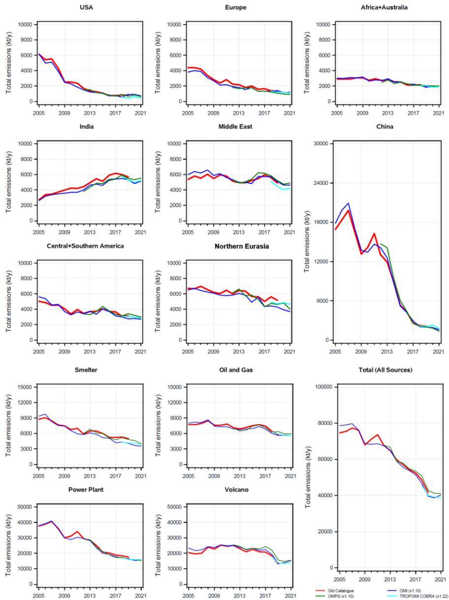
715 Figure 3. Annual SO 2 emissions estimated from four satellite data sets: the original catalogue (red), OMI-based estimates for the version 2 catalogue (blue), OMPS-based estimates for the version 2 catalogue (green), and TROPOMI COBRA-based estimates for the version 2 catalogue (cyan). The data are grouped by region (8 top panels), by emission source type (bottom 4 panels) and the bottom right panel shows total emissions from all sources. TROPOMI-based estimates are adjusted upwards by 22% to account for the difference in used SO 2 cross-sections and OMI and OMPS data are adjusted upwards by 10% as 720 discussed in the text. Only sources included in the original catalogue with the original AMF values were used in this comparison.
