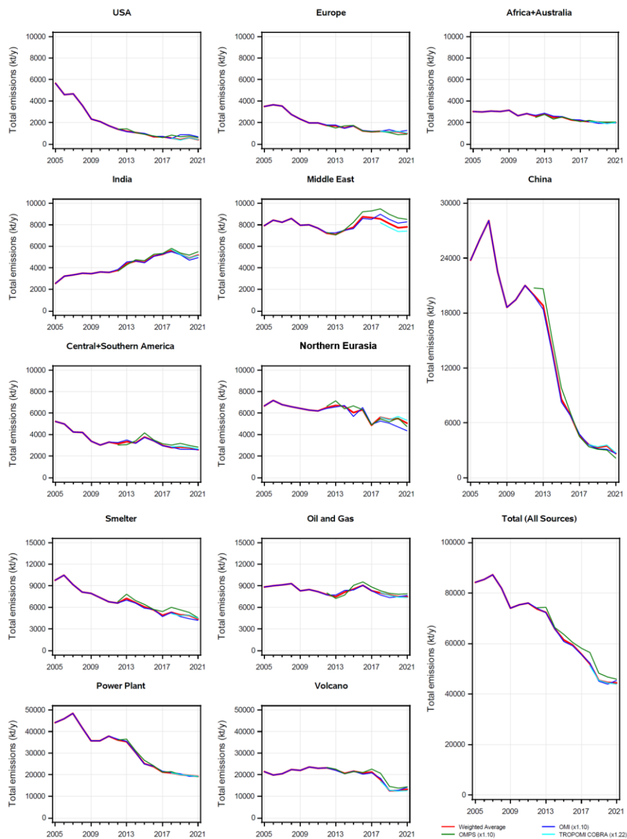
730 Figure 5. Annual SO 2 emissions from four satellite data sets: version 2 catalogue OMI VCD data (blue), version 2 catalogue 735 OMPS data (green), version 2 catalogue TROPOMI COBRA data (cyan) and the weighted average (red). The data are grouped by region (8 top panels), by emission source type (bottom 4 panels) and the bottom right panel shows total emissions from all sources. TROPOMI-based estimates were increased by 22% and OMI and OMPS data were increased by 10% as discussed in the text. The weighted average is based on OMI data only in 2005-2011, on OMI and OMPS data in 2012-2017, and on data from all three instruments in 2018-2021.
