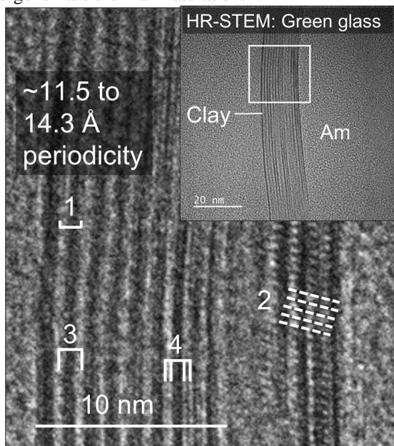
Figure 1: Transmission electron microscope images of a clay mineral with varying periodicity between \sim 11.5 to 14.3\text{ Å} (1), interpreted as the silicate layer basal (001) spacing. Area (2) denotes cross-fringe measurements interpreted as the clay mineral d(060) , measuring \sim 1.50 to 1.53\text{ Å} . Sections (3) and (4) show some layer thickness variability. Am = amorphous.
